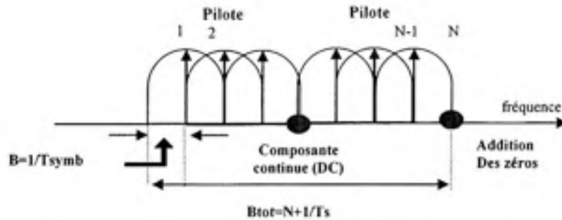
Figure 3.3 Bande du signal OFDM
