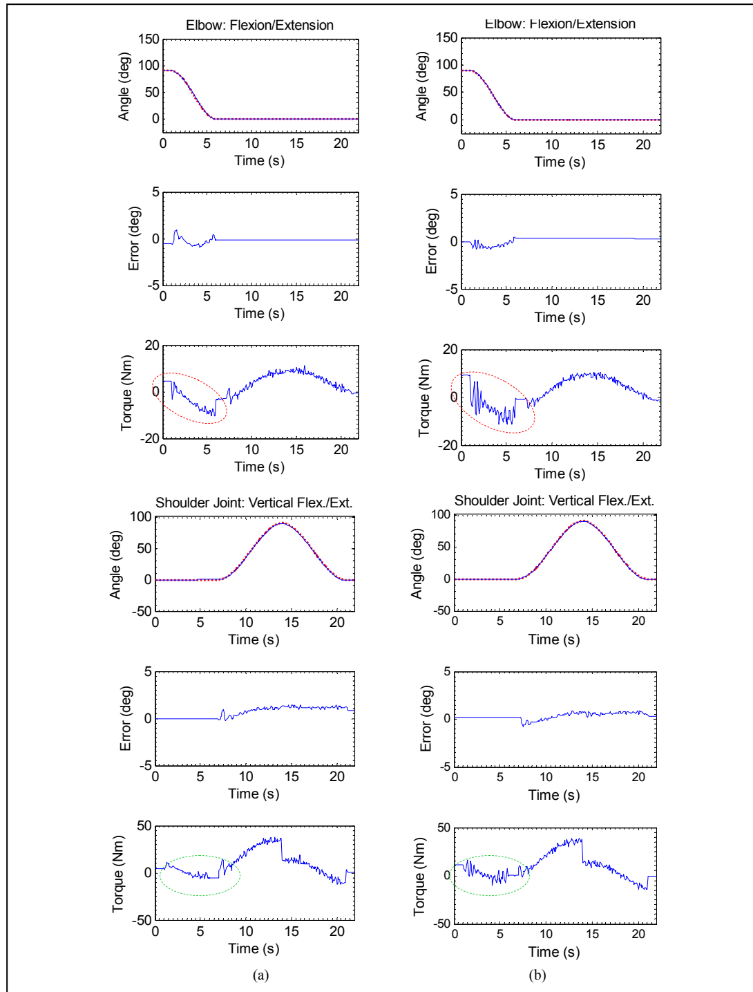
Figure 5.23 Shoulder joint vertical flexion/extension (a) mSMERL (b) SMC with boundary layer
