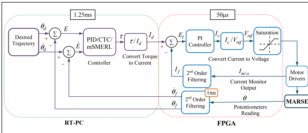
Figure 5.3 Control architecture
