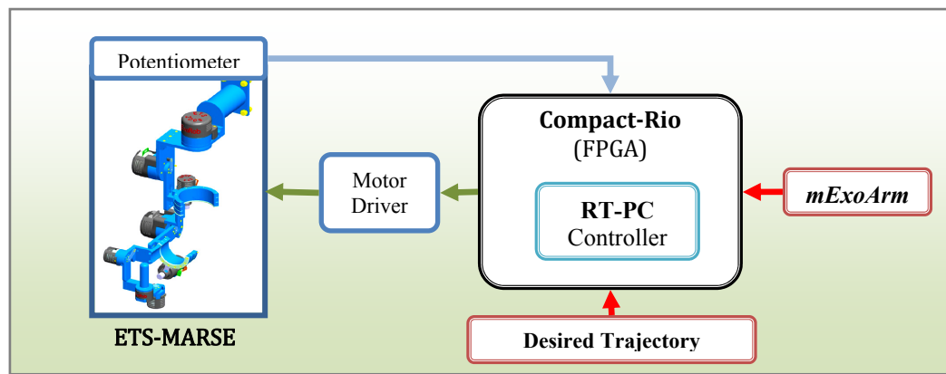
Figure 5.1 Experimental setup
