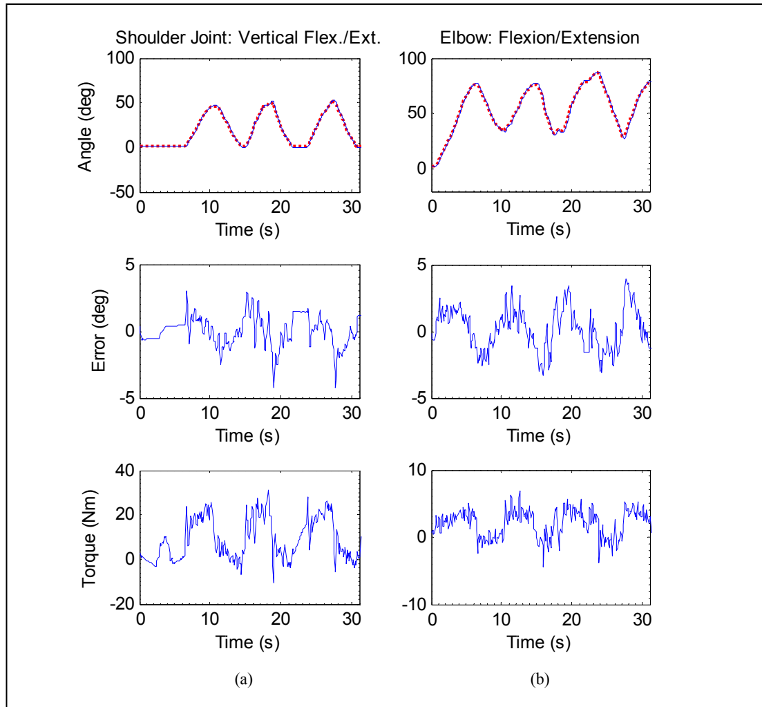
Figure 5.51 Reaching movement by mExoArm (a) Shoulder joint vertical flexion/extension (b) Elbow flexion/extension
