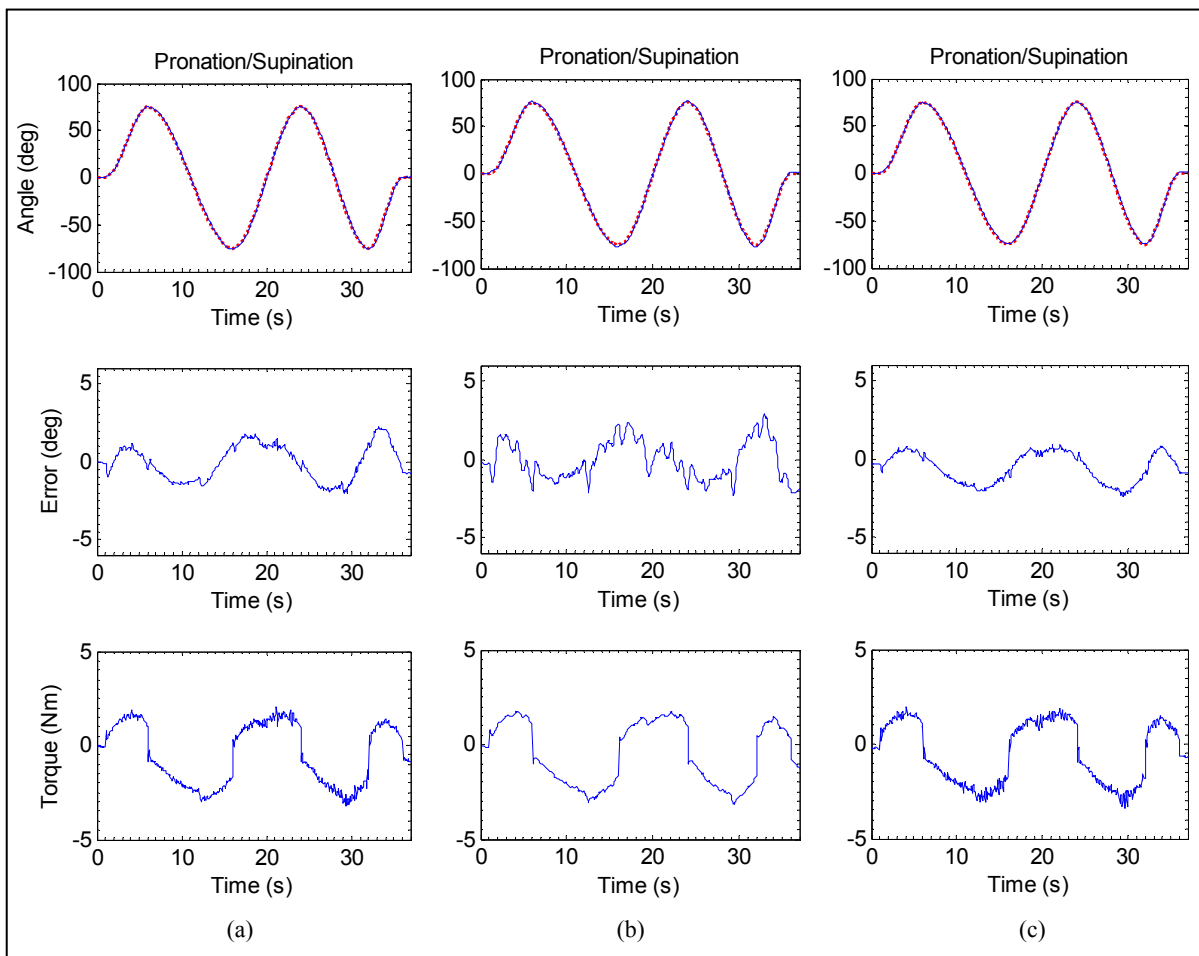
Figure 5.30 Forearm pronation/supination (a) PID (b) CTC and (c) mSMERL
