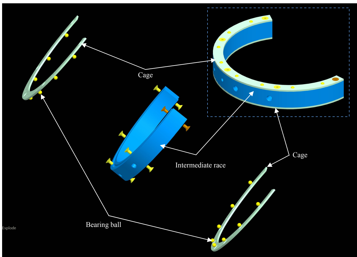
Figure 2.13 Intermediate race assembly
