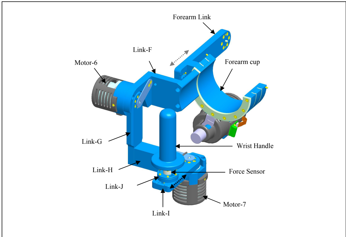
Figure 2.24 Wrist motion support part (2DoFs)
