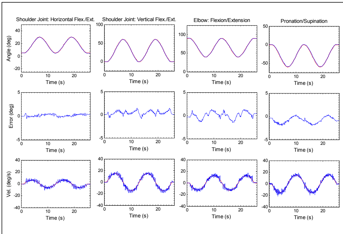
Figure 5.28 Diagonal reaching movement with mSMERL
