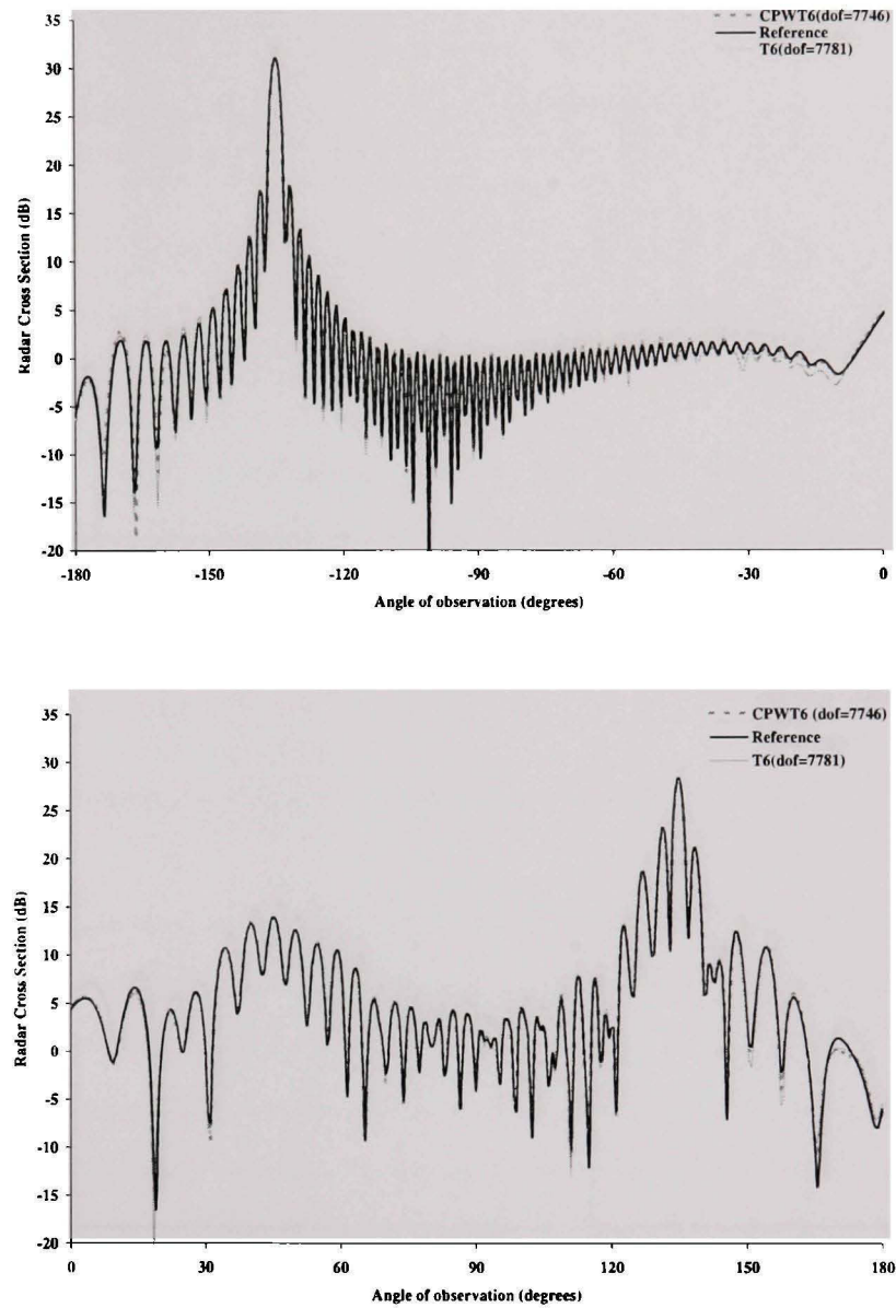
Figure 3.10 Comparison of the RCS of the sound-hard submarine-like scatterer for kD = 20 , m = 1.0 and \theta^{inc} = 225 degrees using the Padé-type ABC with the T6 and CPWT6 finite elements (setting now n_\lambda = 2 and n_q = 3 for the CPWT6 FEM and n_\lambda = 3.5 for the T6 FEM).
