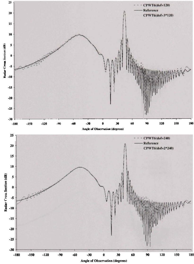
Figure 3.4 Comparison of the computed RCS of the sound-hard elliptical cylinder at ka = 60 , for \theta^{inc} = 45 degrees and m = 0.15 . We use the CPWT6 FEM for different values of n_q .
