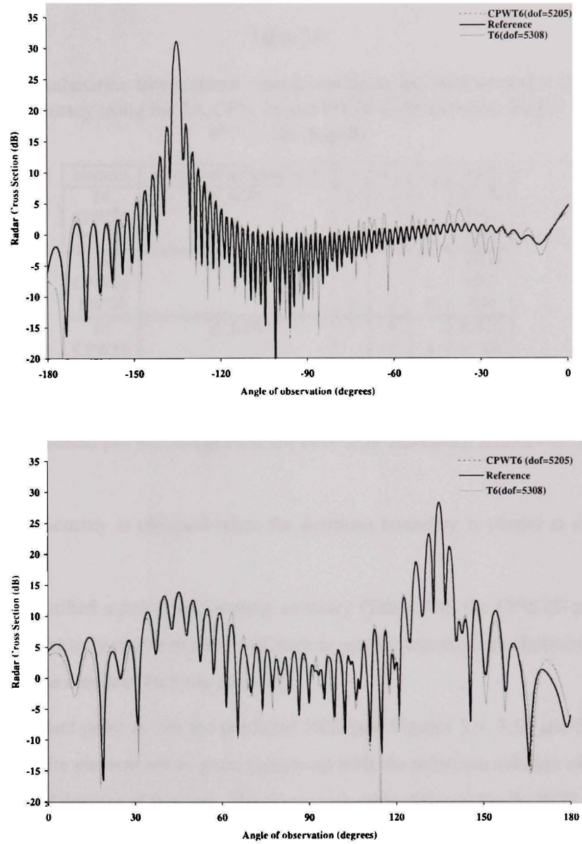
Figure 3.11 Comparison of the RCS of the sound-hard submarine-like scatterer for kD = 20 , m = 2.0 and \theta^{inc} = 225 degrees using the Padé-type ABC with the T6 and CPWT6 FEM ( n_\lambda = 1 and n_q = 5 for the CPWT6 and n_\lambda = 2.3 for the T6 FEM).
