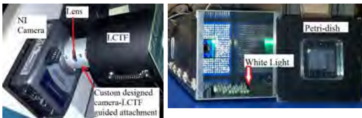
Figure 2.4 White LEDs and biological sample holder showing installed Petri dish with calibration targets
