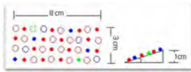
Figure 1.7 Grow light distribution pattern, size and installation angle
