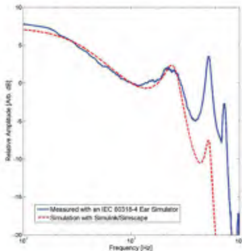
Fig. 14. Comparison of the fine-band frequency response of a Knowles® CI22955 - reproduced from the PSpice model provided by Knowles® - measured on an IEC 60318-4 Ear Simulator and a lumped-element simulated in Simulink®/Simscape™.
