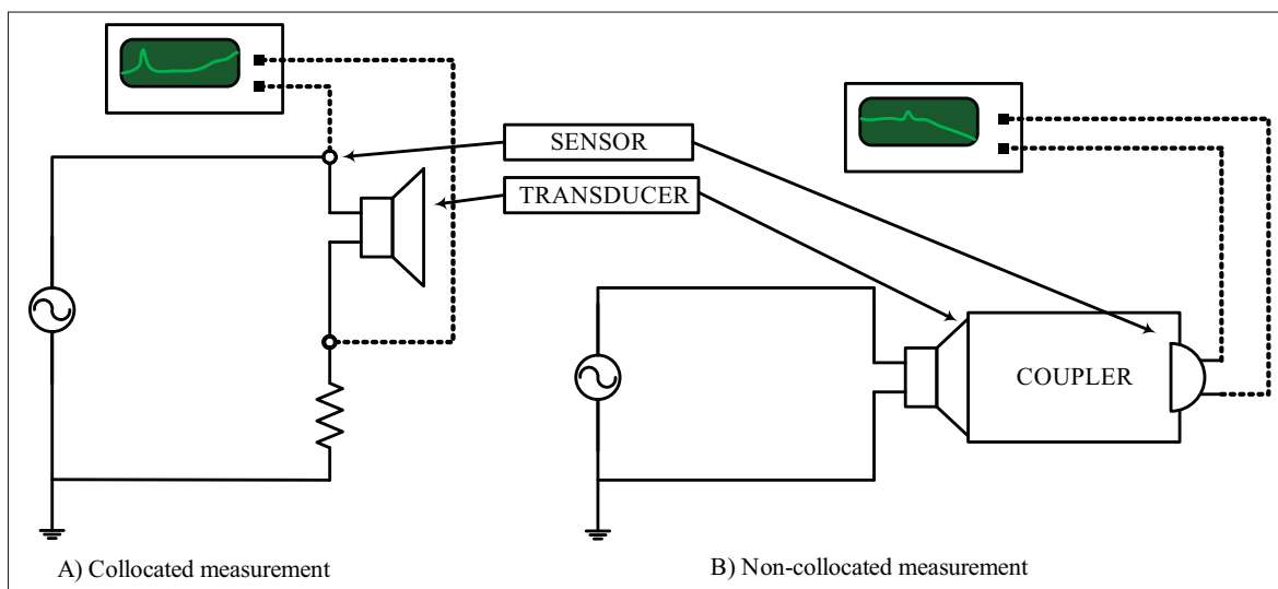
Figure 2.1 Difference between a collocated measurement and a non-collocated measurement.
