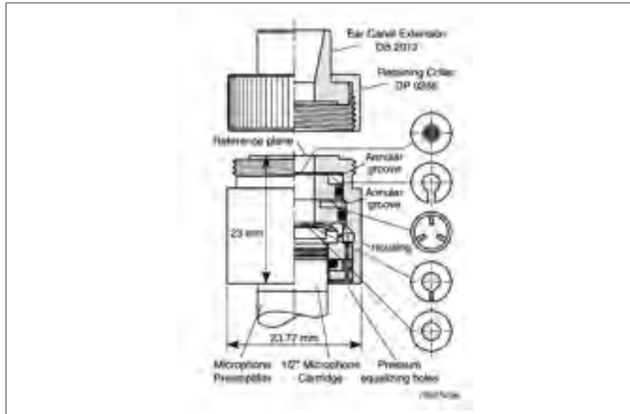
Figure 3.7 Sectional view of the Brüel & Kjaer Ear Simulator Type 4157, compliant to IEC 60318-4 (Formerly known as IEC 711) [as presented in Jönsson et al. (2004)]
