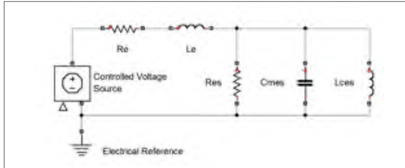
Figure 3.32 Lumped-Element equivalent electrical impedance circuit of a moving-coil micro-loudspeaker.
