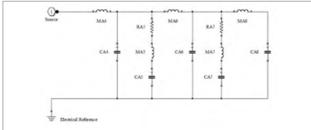
Figure 3.35 Equivalent Lumped-Element model of the Brüel & Kjaer Ear Simulator Type 4157 which is compliant to IEC 60318-4 (Formerly known as IEC 711) Jönsson et al. (2004).
