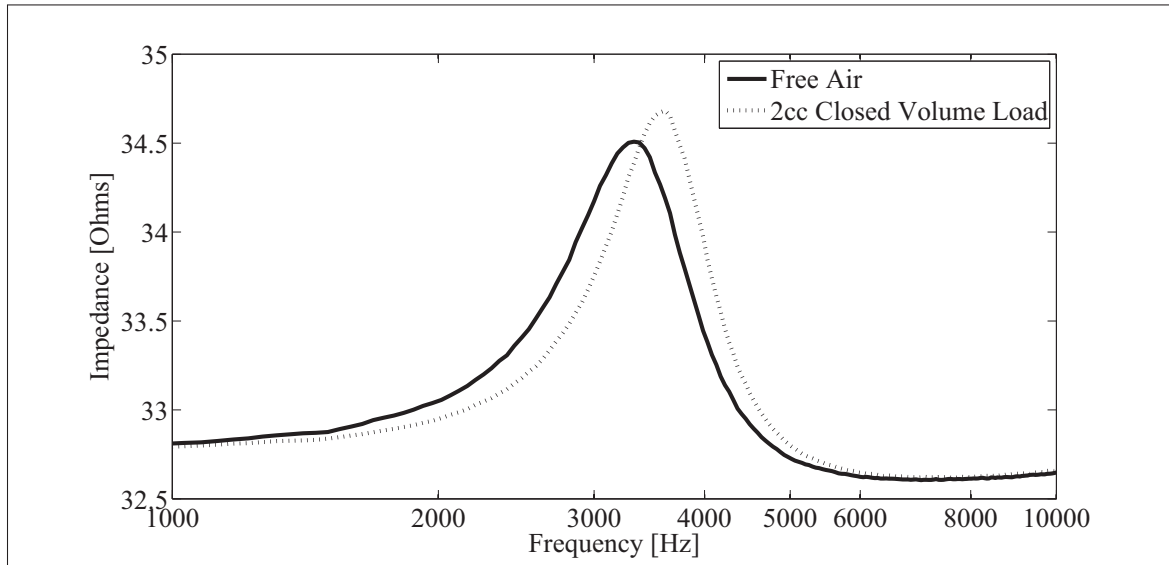
Figure 2.3 Impedance curve of a moving-coil micro-loudspeaker measured in free air and with a 2cc closed volume air load.
