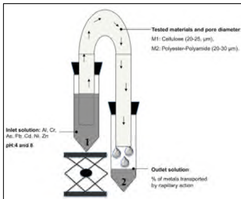
Figure 2.1 Capillary siphon
