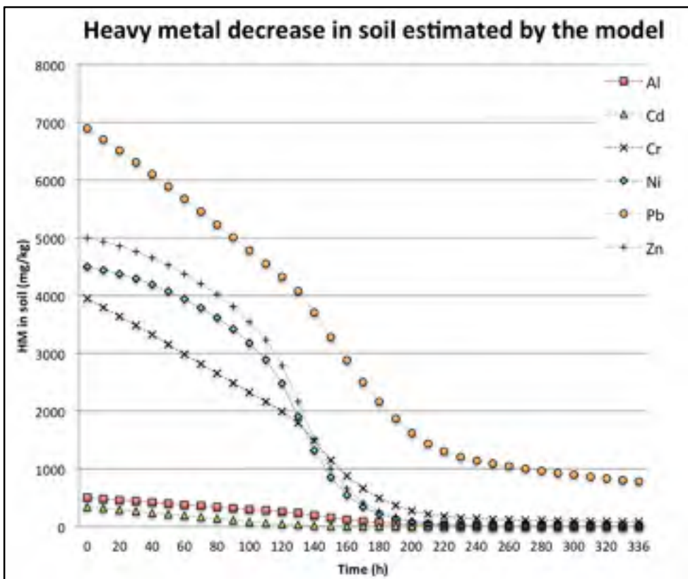
Figure 5.3 Behaviour of the heavy metal concentration estimated through the model
