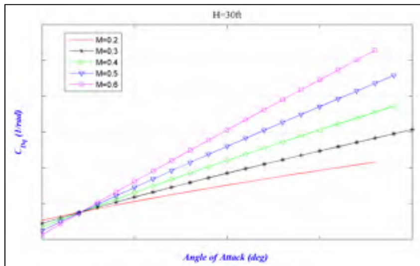
Figure 2.9 C_{Dq} versus \alpha at the altitude H = 30 \text{ ft} and q = 5 \text{ deg/s}
