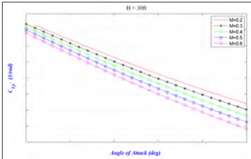
Figure 2.11 C_{y\dot{\beta}} versus \alpha at the altitude H = 30 ft
