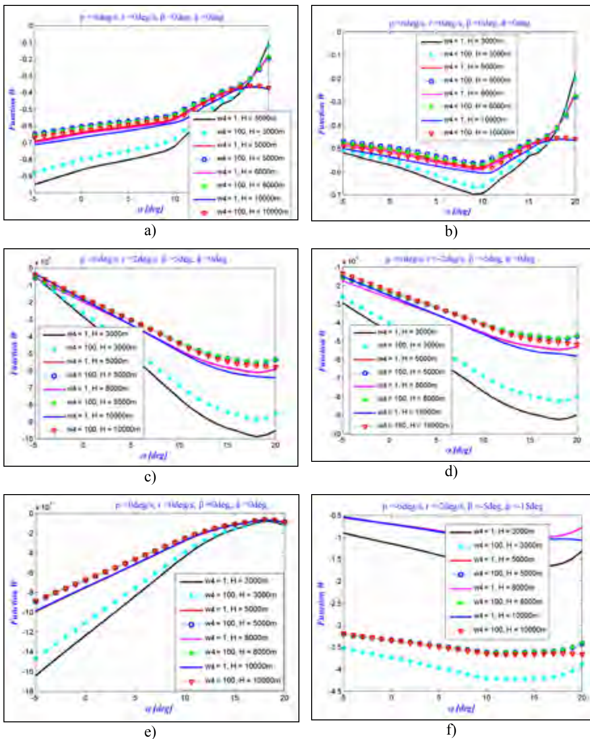
Figure 5.6 Lateral-directional stability analysis with the WFM for different values of constant w_4 as a function of the angle of attack for M = 0.4
