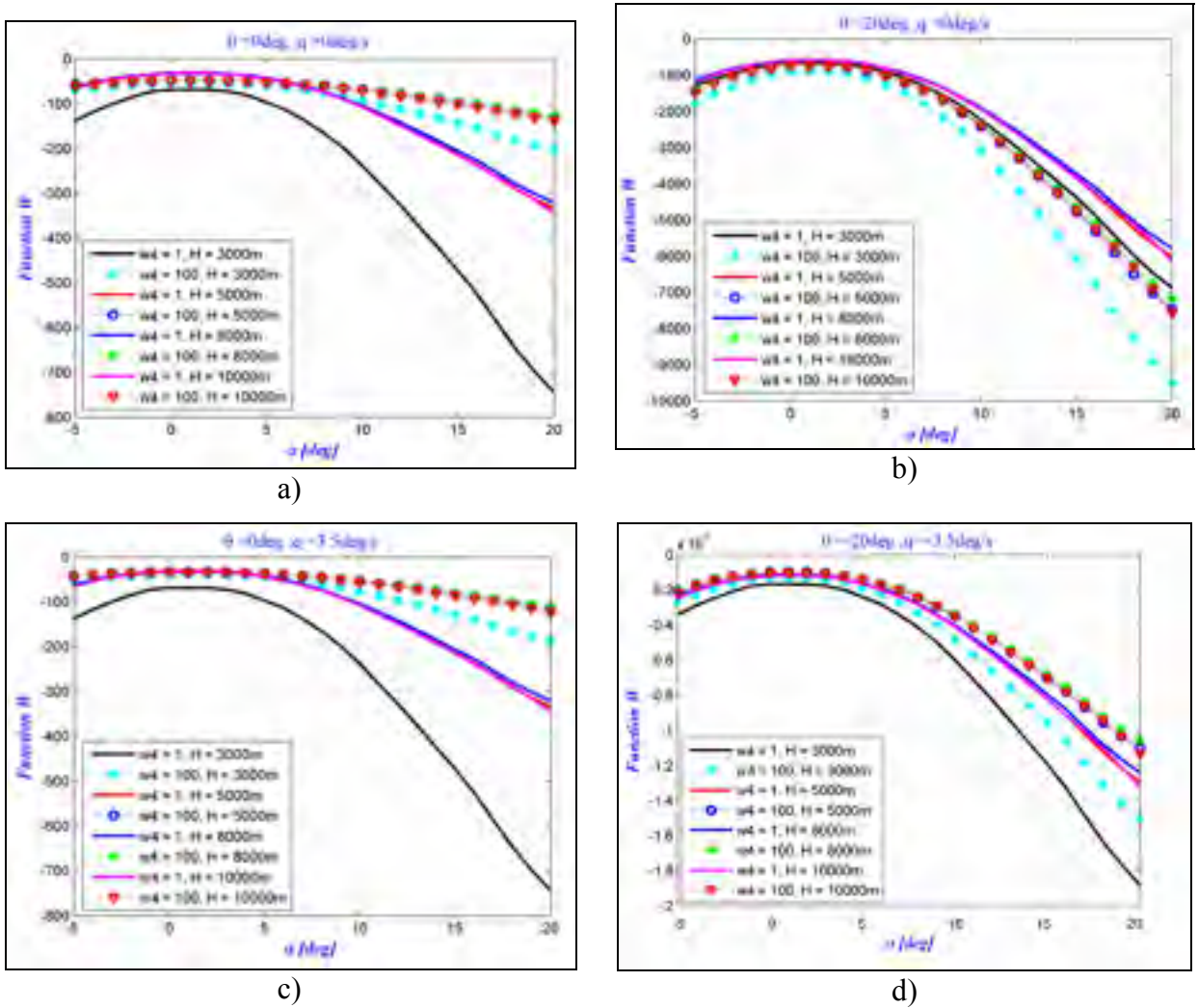
Figure 5.3 Stability analysis with the WFM for different values of constant w_{4long} as a function of angle of attack for Mach number M = 0.4
