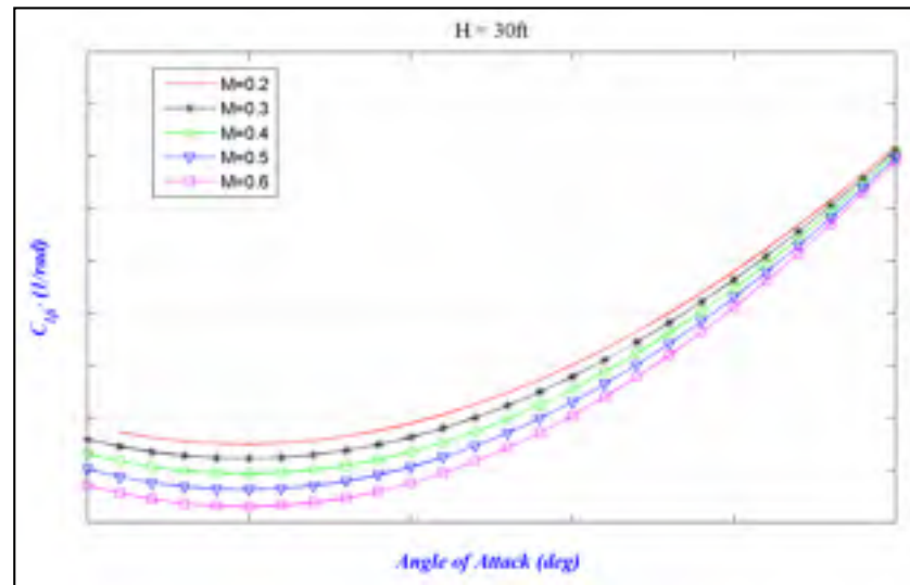
Figure 2.10 C_{l\dot{\beta}} versus \alpha at the altitude H = 30 ft
