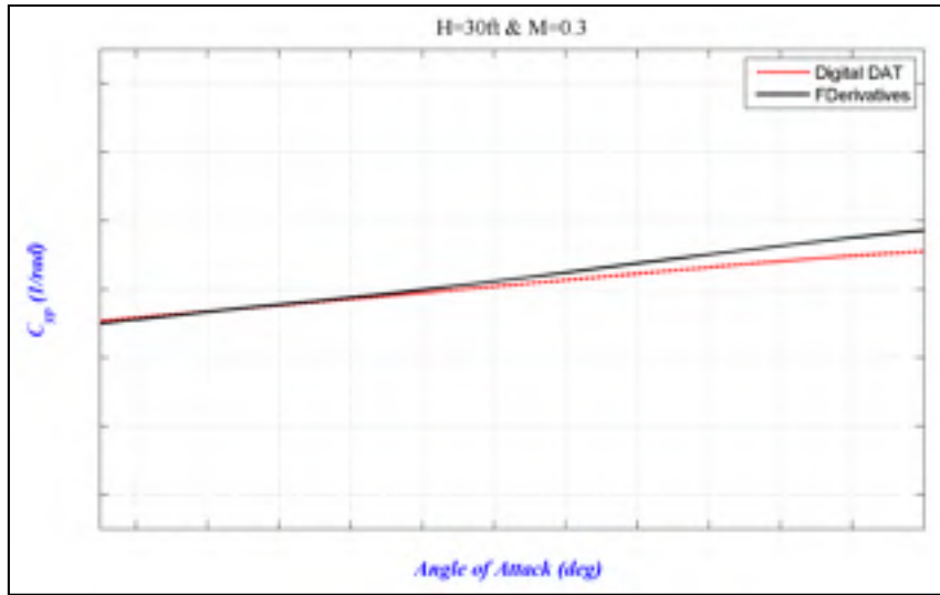
Figure 2.21 C_{np} versus \alpha at Mach number M = 0.3
