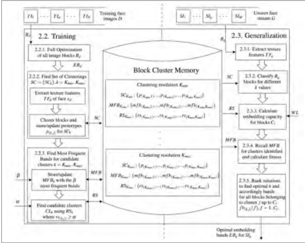
Figure 2.1 General overview of BMRC architecture and processing steps for training and generalization phases. BCM is organized based on clustering resolution k ranging from K_{min} to K_{max} .
