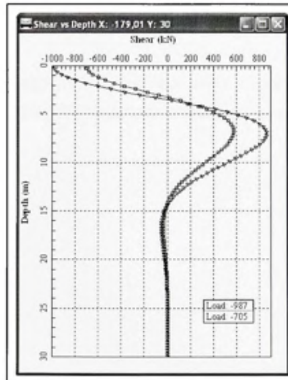
Figure VI.4 Effort tranchants ( V_y ) versus profondeur.
