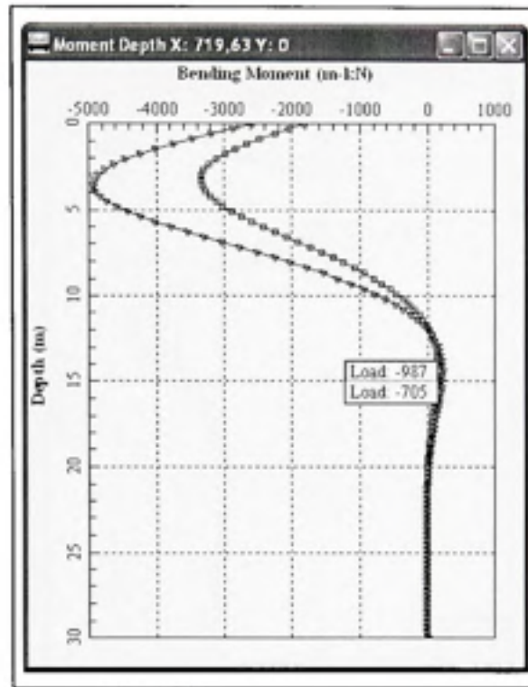
Figure VI.3 Moments ( M_x ) versus profondeur.
