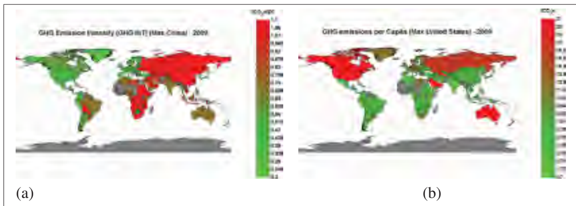
Figure-A II-1 a) GHG Emission intensity (GHGINT) in 2009 (in GtCO 2 e/$B). b) GHG emissions per capita in the same year (in GtCO 2 e/Million Capita). Data Sources: US Energy Information Administration, World Bank, United Nations Statistics and Research Database, International Monetary Fund, and United Nations Development Programme.
