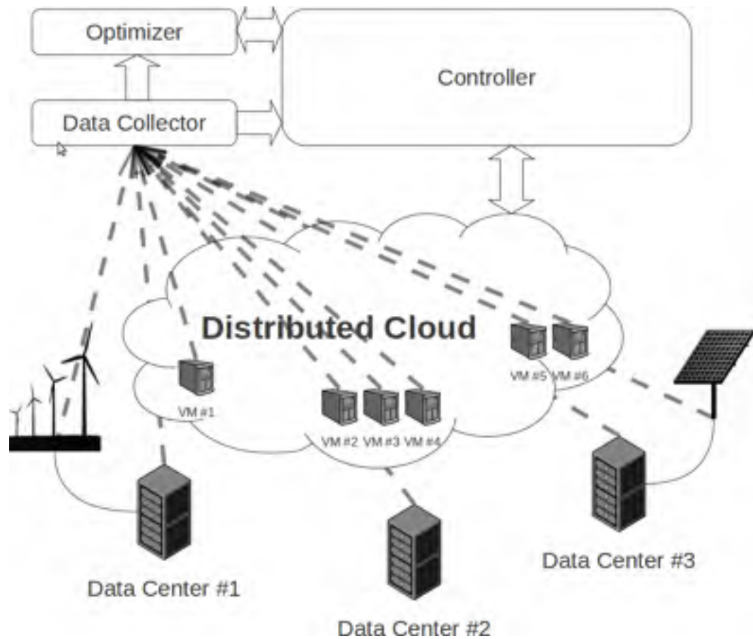
Figure 5.4 CADCloud Schema.
