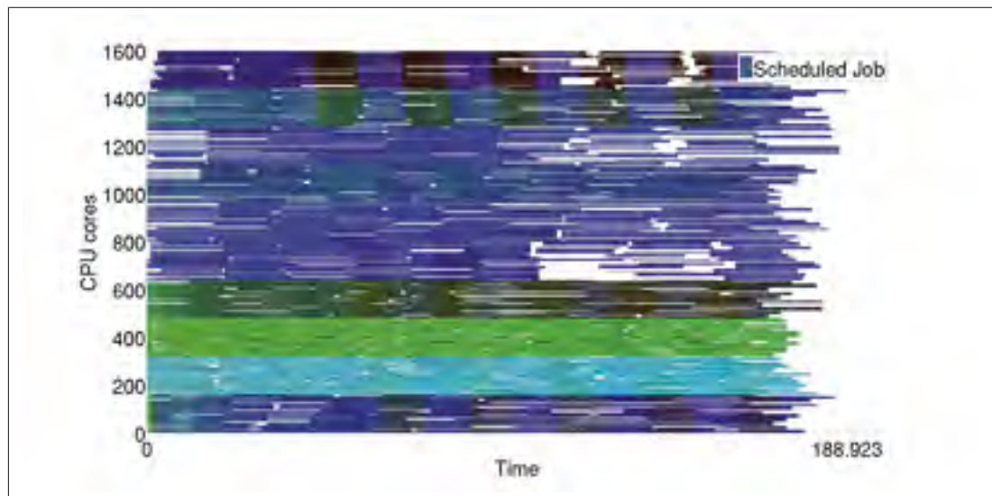
Figure 6.10 Scheduled jobs plot by CARB algorithm
