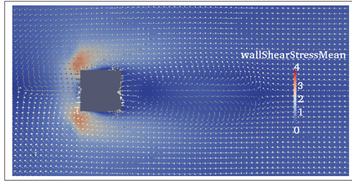
Figure 5.35 Time-averaged wall shear stresses at the bottom boundary for the thick boundary layer case B3. Units: [\text{m}^2/\text{s}^2] .
