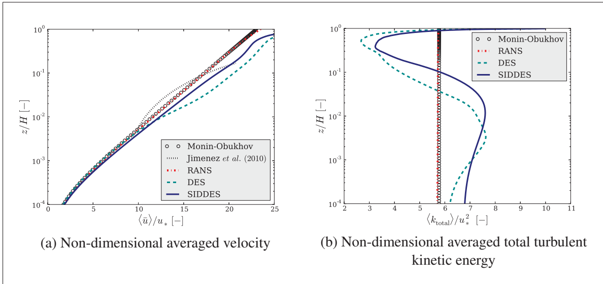
Figure 4.1 Atmospheric surface layer case with z_0 = 0.1 m. The k - \omega SST, k - \omega SST-DES and k - \omega SST-SIDDDES results are compared to the Smagorinsky results obtained from the Jimenez et al. (2010) figures.
