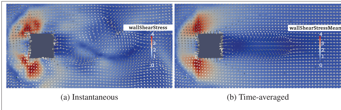
Figure 5.14 Wall shear stresses at the bottom boundary for case A with SIDDES. The colour bar represents the magnitude. Units: [\text{m}^2/\text{s}^2] .
