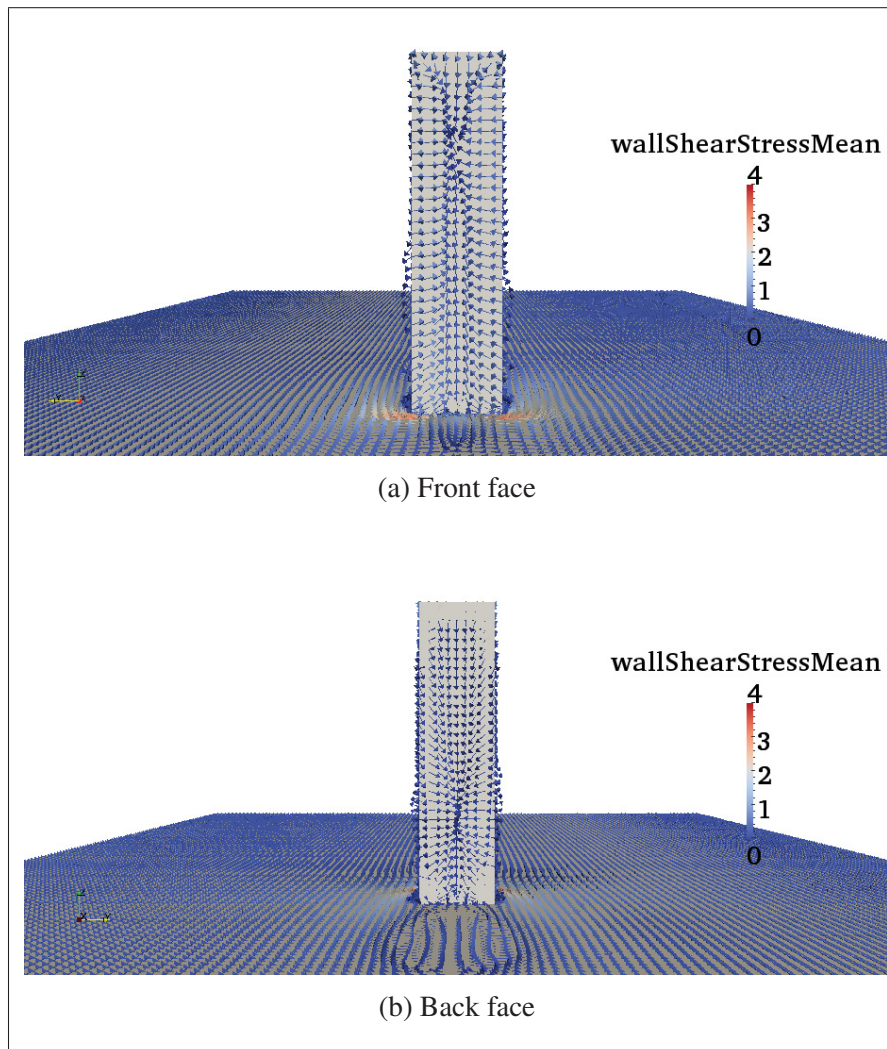
Figure 5.34 Time-averaged wall shear stresses vectors on the cylinder for SIDDES case B3. Colour scale represents their magnitude. Units: [\text{m}^2/\text{s}^2] .
