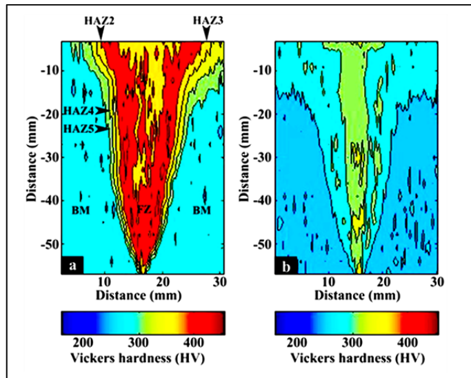
Figure 3-8 2D Microhardness map of fully penetrated CA6NM welds in the (a) as-welded and (b) PWHTed conditions
