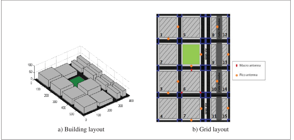
Figure 5.3 Madrid grid model layout
