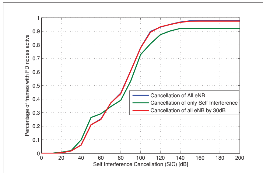
Figure 5.11 Madrid grid model: FD node activity
