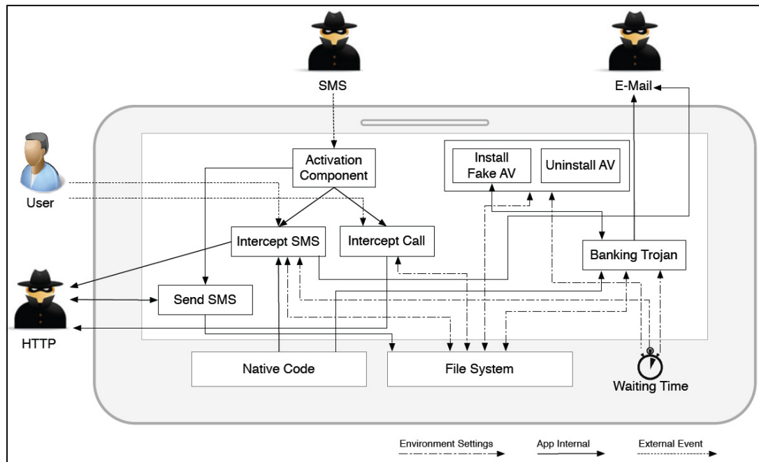
Figure 2.2 Le Malware Android / BadAccents (Felt, Finifter, Chin, Hanna, & Wagner, 2011)
