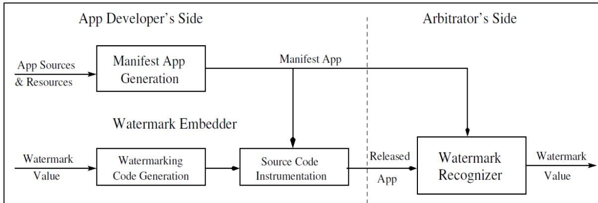
Figure 2.5 L'architecture globale d'AppInk (Zhou, Zhang, & Jiang, AppInk: watermarking android apps for repackaging deterrence, 2013)
