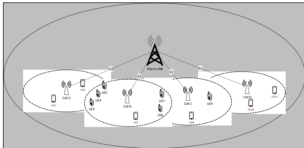
Figure 5.1 Heterogeneous Radio Access Network Architecture
