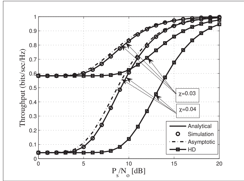
Figure 3.13 Throughput vs. P_S/N_0 for different values of \chi with \bar{\gamma}_{ID}=15 dB, m_{ij}=2 , \bar{\gamma}_{RR}=5 dB and R_S=R_T=1 bit/sec/Hz
