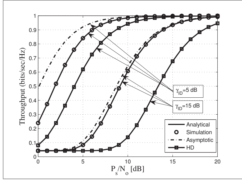
Figure 3.12 Throughput vs. P_S/N_0 for different values of \bar{\gamma}_{ID} with m_{ij}=2 , \bar{\gamma}_{RR}=5 dB and R_S=R_T=1 bit/sec/Hz
