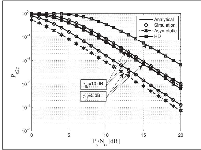
Figure 3.3 End-to-end outage probability vs. P_S/N_o for different values of \bar{\gamma}_{ID} with m_{ij}=2 , \bar{\gamma}_{RR}=5 dB, and R_T=1 bit/sec/Hz
