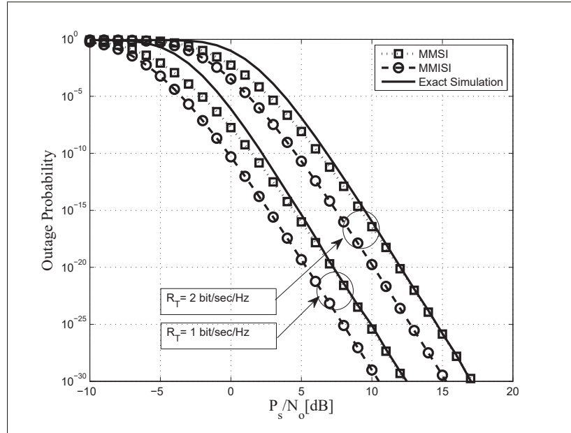
Figure 5.5 Analytical and simulation results for the outage probability vs. P_S/N_o of V2V wireless communications in the presence of interference over Nakagami- m fading channels for different values of R_T , m_{ij} = 2 , where i, j \in \{S, R, D\} , \delta = 2 vehicles/lane/unit length, w = 0.04 , M_R = M_L = 2 , T_R = d_{SD} = 1 , d_{SR_i} = 0.4 and 0.7 , d_{R_iD} = 0.6 and 0.3 , respectively, d_{R_iR_i} = 0.01 , \bar{\gamma}_{R_iR_i} = 0 dB and \eta = 3.18
