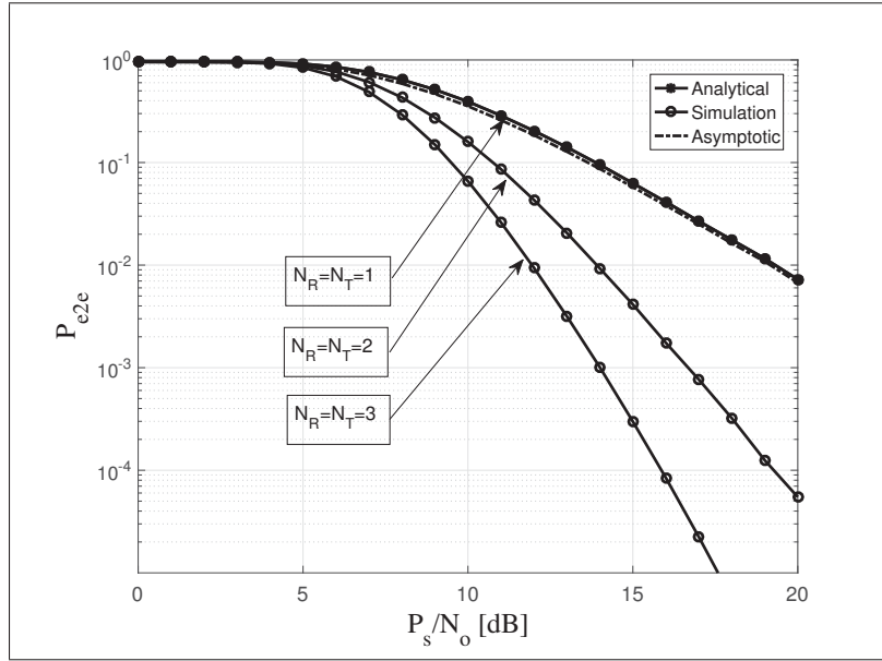
Figure 3.11 End-to-end outage probability vs. P_S/N_O for different numbers of transmitting ( N_T ) and receiving ( N_R ) antennas at the relay node with m_{ij}=2 , \bar{\gamma}_{RR}=5 dB, \bar{\gamma}_{ID}=15 dB, and R_T=1 bit/sec/Hz
