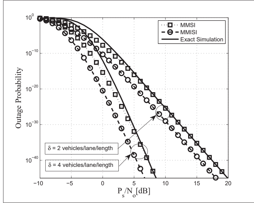
Figure 5.7 Analytical and simulation results for the outage probability vs. P_S/N_o of V2V wireless communications in the presence of interference over Nakagami- m fading channels for different values of \delta , M_R = M_L = 2 , m_{ij} = 2 , where i, j \in \{S, R, D\} , w = 0.04 , T_R = d_{SD} = 1 , d_{SR_i} = 0.4 and 0.7 , d_{R_iD} = 0.6 and 0.3 , respectively, d_{R_iR_i} = 0.01 , \bar{\gamma}_{R_iR_i} = 0 dB, R_T = 1 bit/sec/Hz and \eta = 3.18 .
