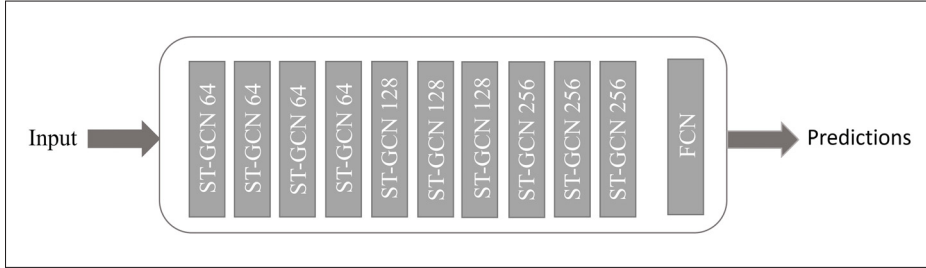
Figure 2.3 Spatial temporal graph convolution network architecture
