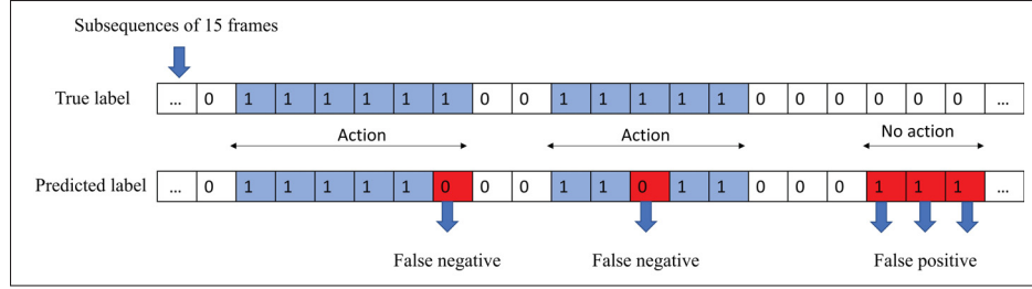
Figure 3.4 Action detection module classification errors
