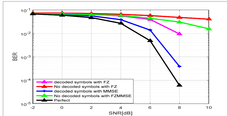
Figure 2.7 LT code with MMSE and ZF
