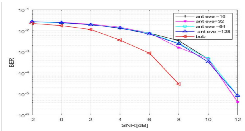
Figure 3.5 BER of Eve with different number of antennas
