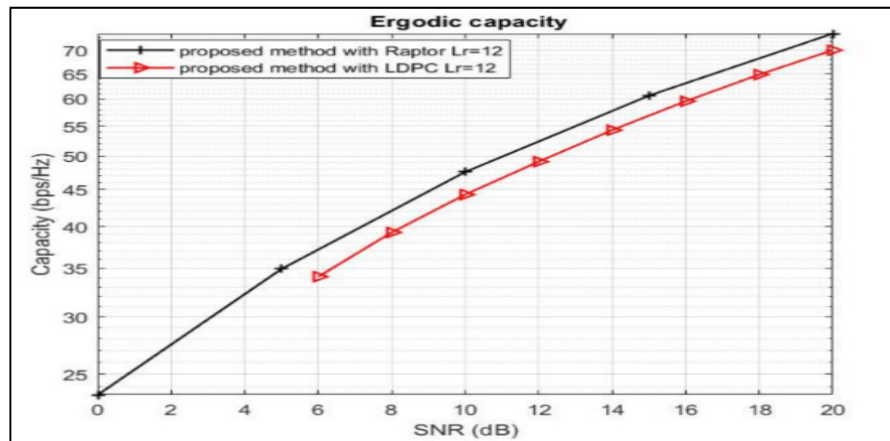
Figure 4.3 Ergodic capacity of Raptor and LDPC codes
