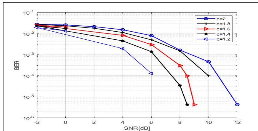
Figure 3.6 BER of Eve with different values of a coefficient c
