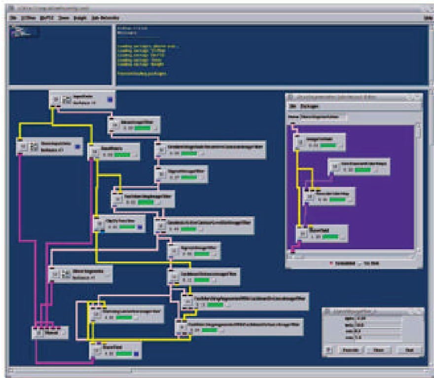
Figure 4.6 Exemple SCIRun.
