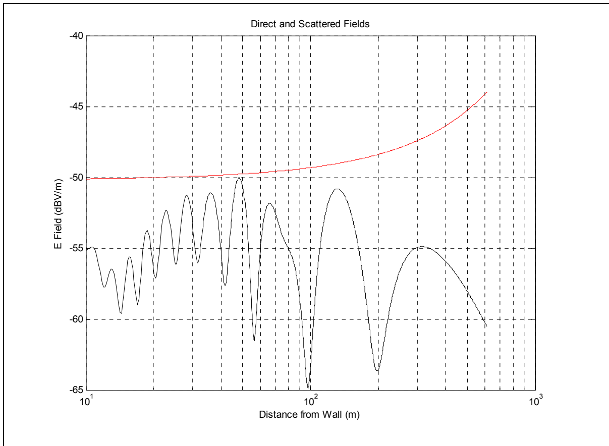
Figure 2.7 Vertical electric field magnitude, 10 m × 20 m wall, ground reflection. Red: direct field, Black: reflected field.
