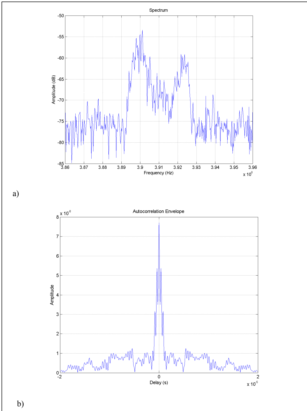
Figure 3.13 Spectrum analysis (a & b).
