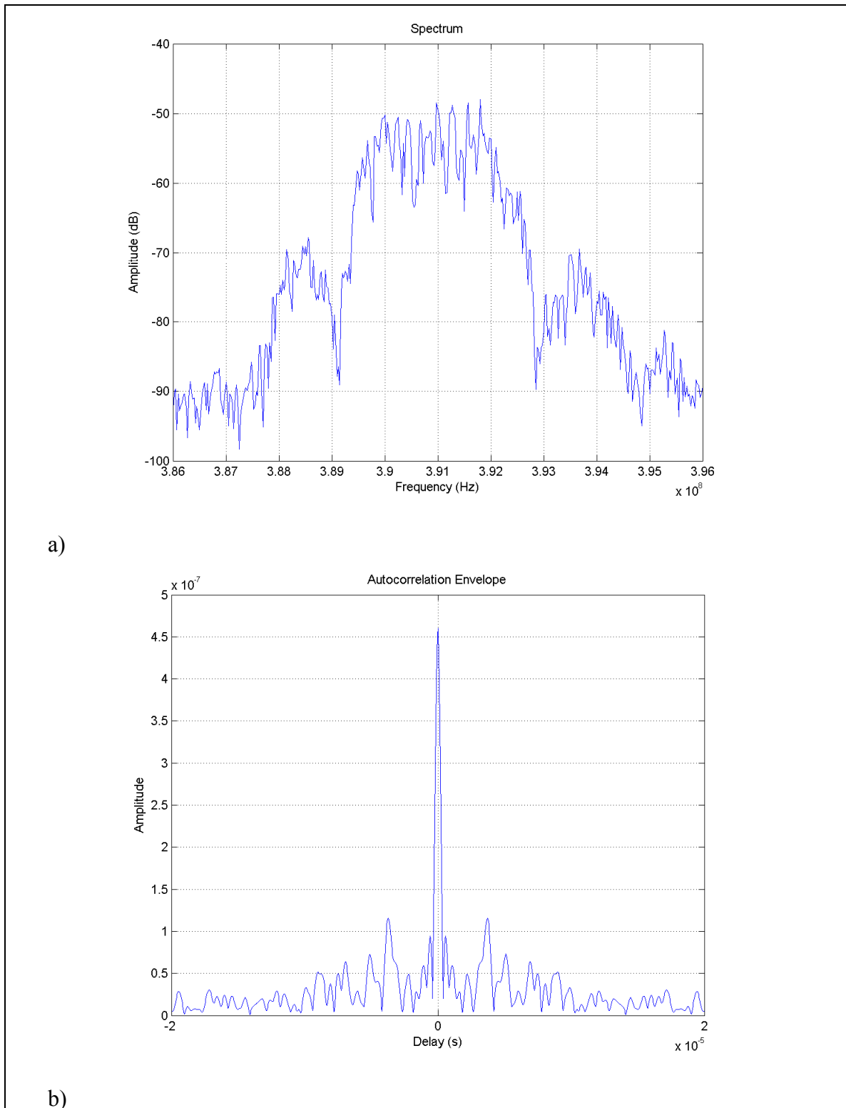
Figure 3.15 Spectrum analysis (a & b).
