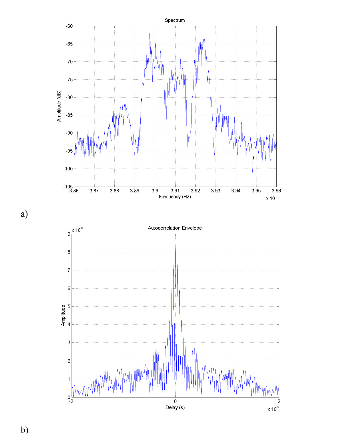
Figure 3.12 Spectrum analysis (a & b).
