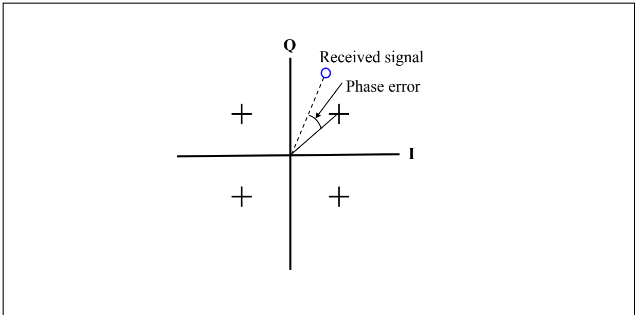
Figure 5.3 QPSK constellation.
