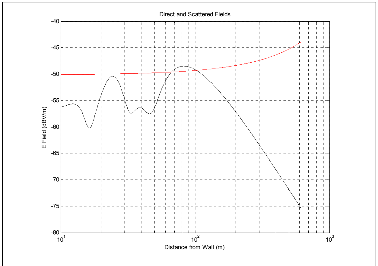
Figure 2.6 Vertical electric field magnitude, 10 \text{ m} \times 10 \text{ m} wall, ground reflection. Red: direct field, Black: reflected field.
