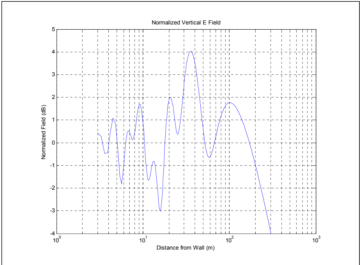
Figure 2.4 Vertical electric field magnitude, 20m × 10 m wall.
