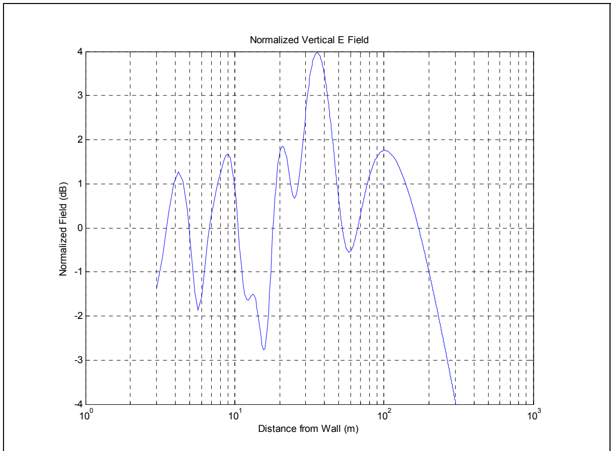
Figure 2.3 Vertical electric field magnitude, 10 m × 20 m wall.
