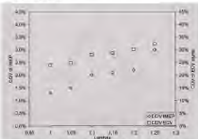
Figure 3: Trends in COV of IMEP and of ECV signal at 1500 RPM, 40 N-m and MBT for different excess ratio.
