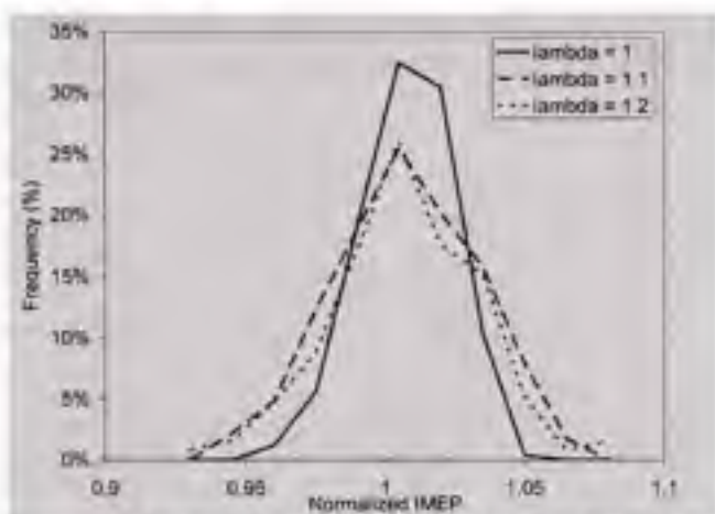
Figure 4: Frequency distribution of IMEP for different excess ratio at 1500 RPM, 40 N-m and MBT spark timing.
