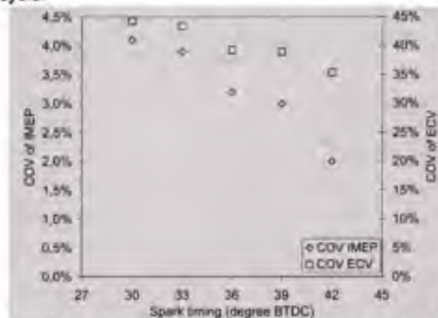
Figure 6: Trends of COV of IMEP and of ECV signal at 2000 RPM, 30 N-m and an excess ratio of 1.1 for different spark timing
