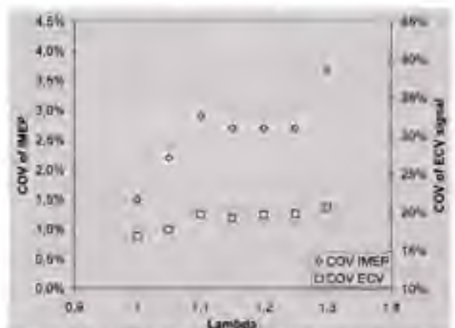
Figure 13: COV of IMEP and COV of ECV signal at 1000 RPM, 40 N-m and MBT spark timing at each operating point.
