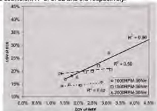
Figure 12: COV of temperature sensor signal as a function of COV of IMEP at 30 N-m for different engine speeds, different excess ratio and constant spark timing.
