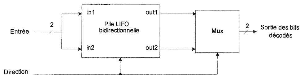
Figure 26 Unité LIFO
