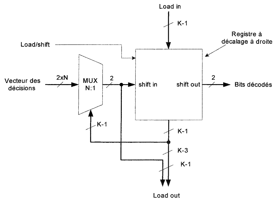
Figure 24 Bloc Mux_logic
