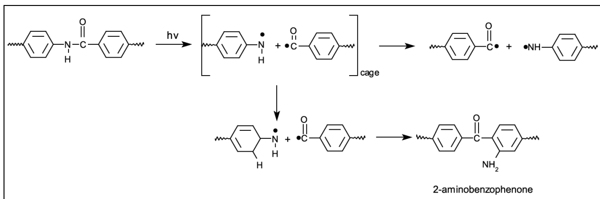
Figure 5.2 Mechanism of Photo-Fries rearrangement for Kevlar ® .
