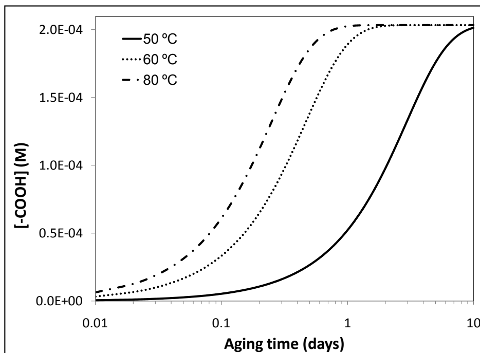
Figure 5.13 Plots of [-\text{COOH}] values yielded by equation (5.5) for the selected aging temperatures.
