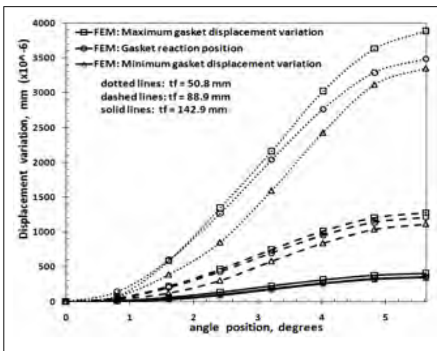
Figure 5.4 FEA Gasket displacement variations of 52 in HE flange, 32 bolts
