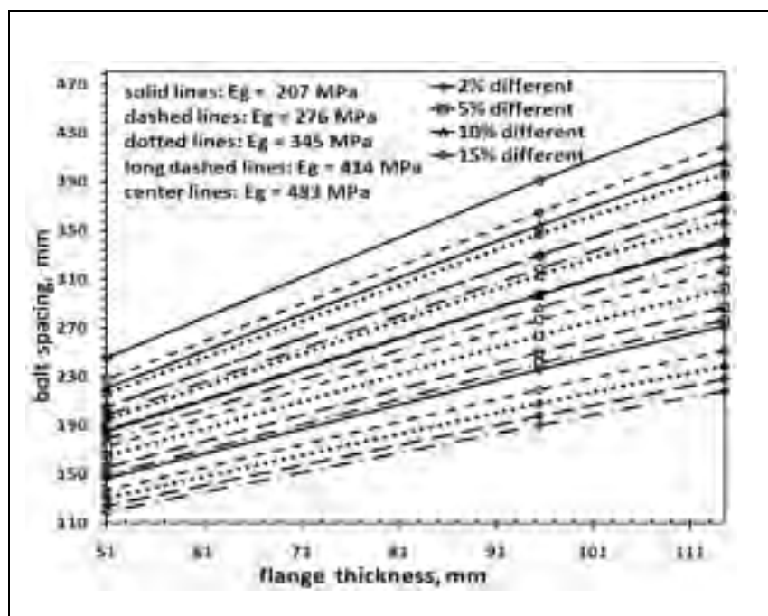
Figure 6.11 Relationship between bolt spacing and flange thickness; 120 in HE flange
