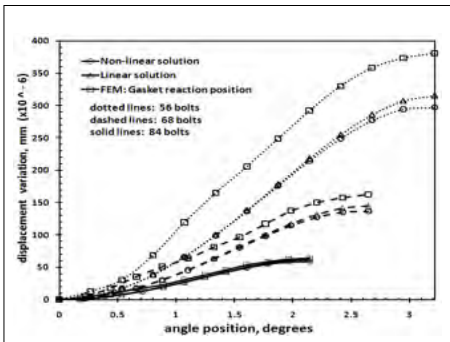
Figure 5.9 Gasket displacement variations of 120 in HE flange, t_f = 165.1 mm
