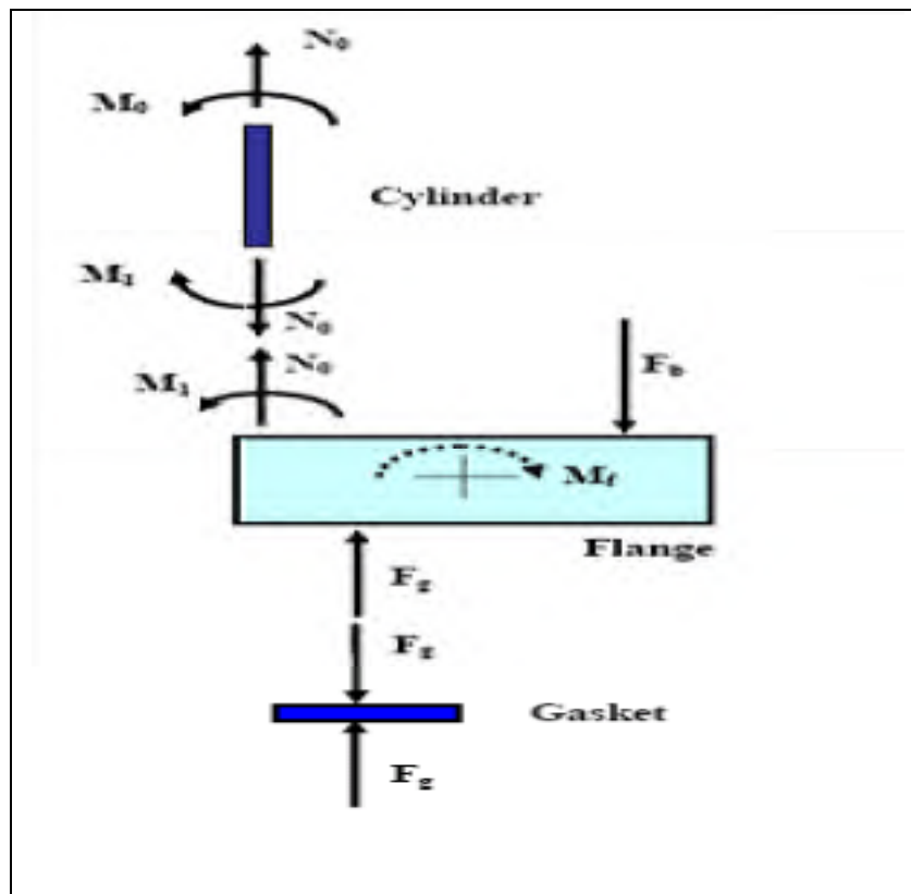
Figure 4.2 Loads in a bolted flange gasketed joint
