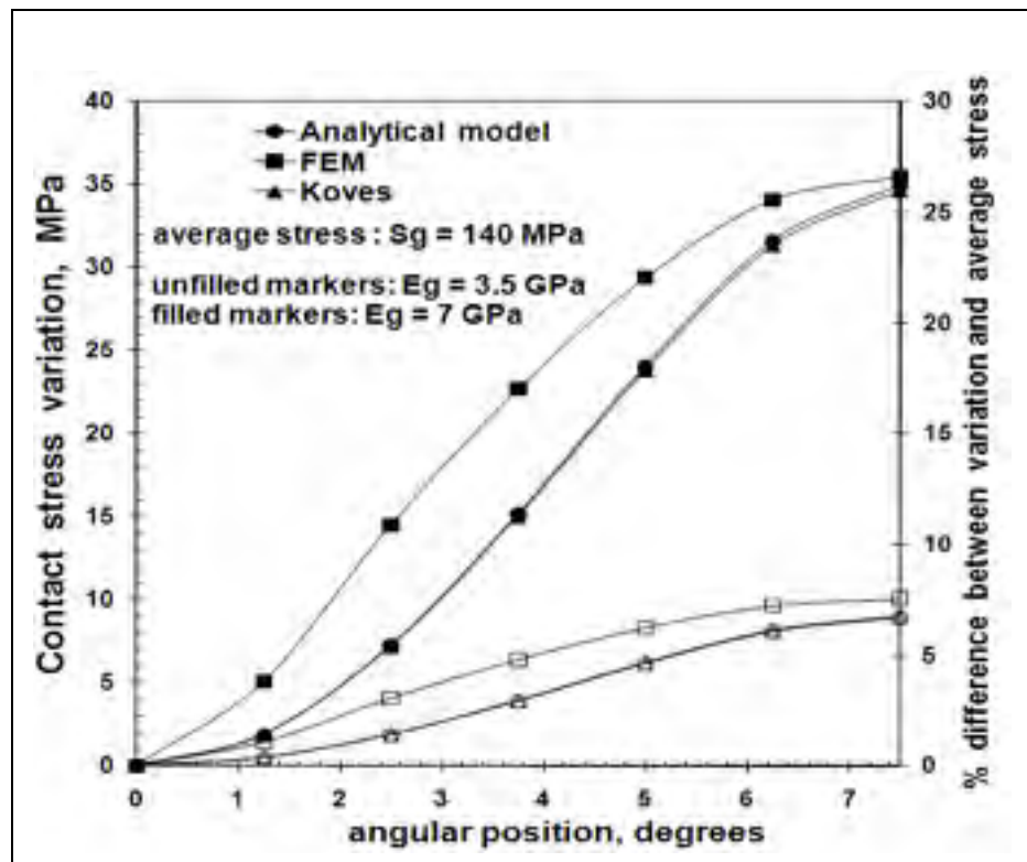
Figure 4.4 Contact stress variation of 52 in. HE flange t_f = 89 mm, 24 bolts
