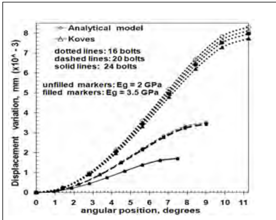
Figure 4.9 Displacement variation of 24 in. HE flange t_f = 38 mm
