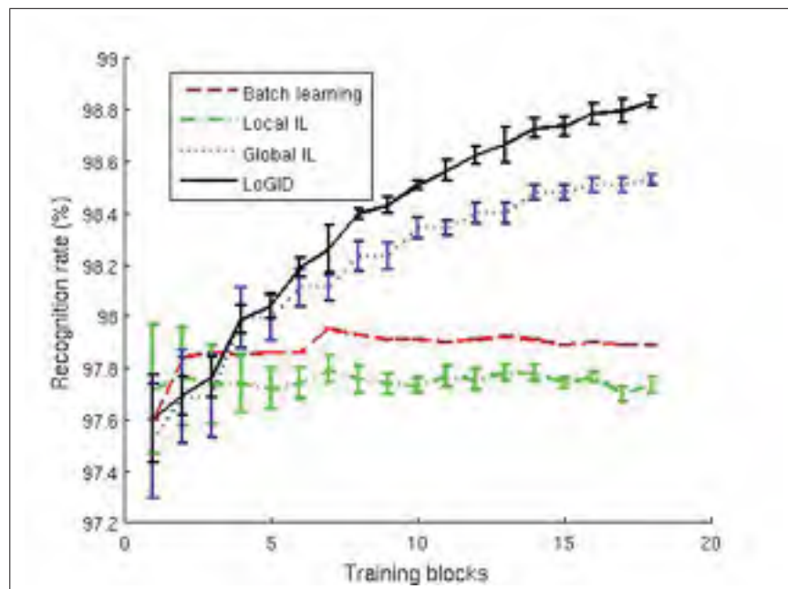
Figure 3.14 Performance comparison for NIST Digits in test1 .
