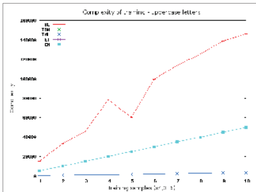
Figure 1.8 Training complexity for uppercase letters
