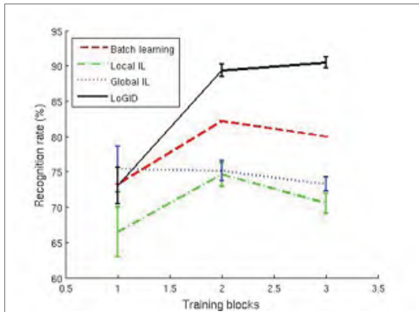
Figure 3.11 Performance comparison for Japanese Vowels.
