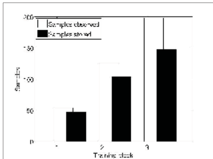
Figure 3.16 Comparison of the number of samples held in DSet' with all the samples observed, on Japanese Vowels.
