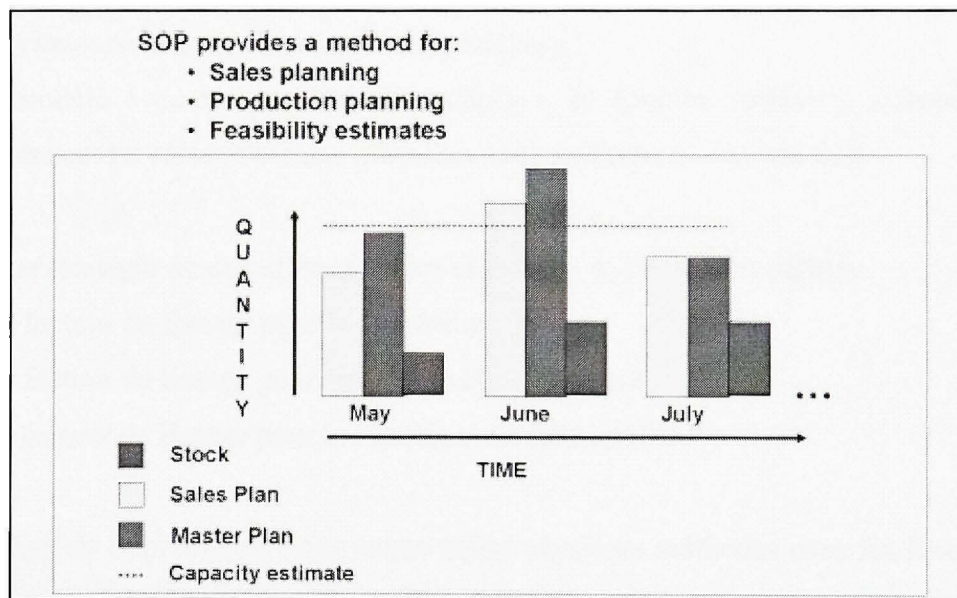
Figure 3.2 SOP plan.
