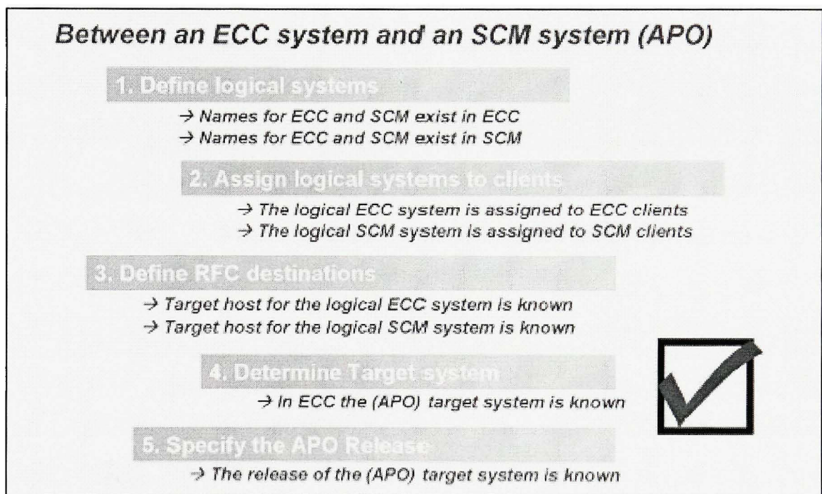
Figure 2.8 Configuration du CIF.
