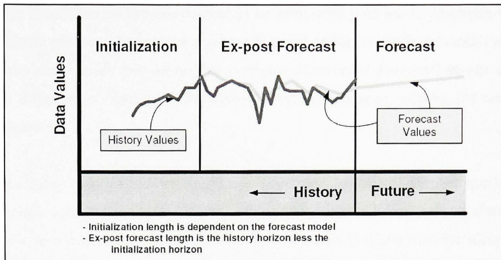
Figure 4.18 Ex-post forecast.
