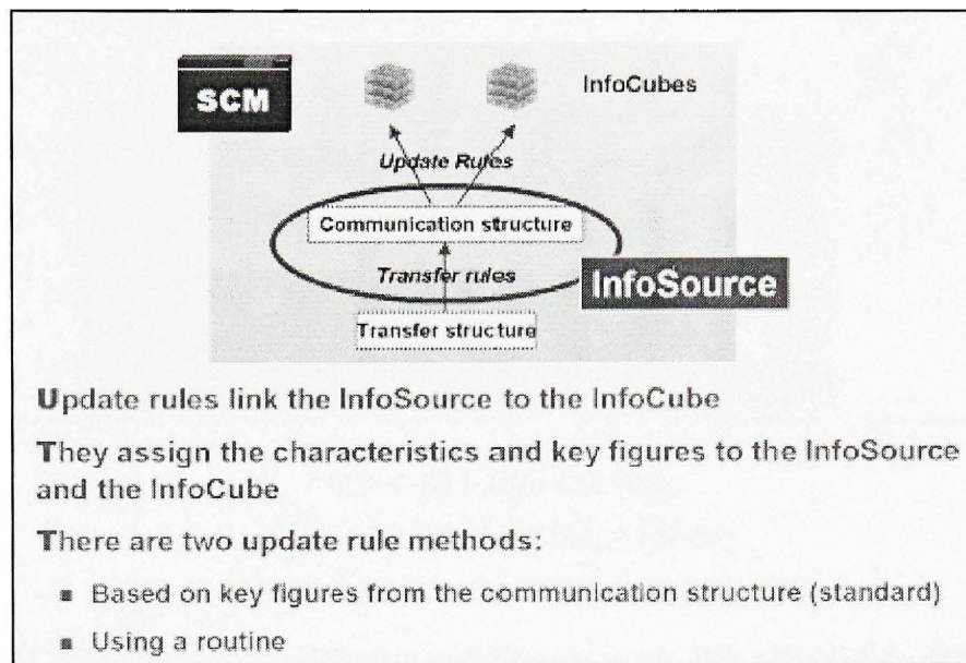
Figure 4.12 Update Rule.
