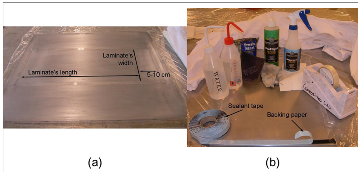
Figure 3.1 Mold preparation: (a) Transparent tape protection for a thick laminate and (b) WaterWorks products and sealant tape installation
