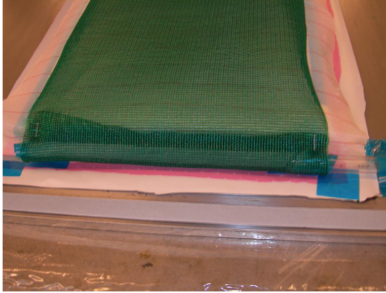
Figure 3.11 Inlet tube installation for a thick laminate
