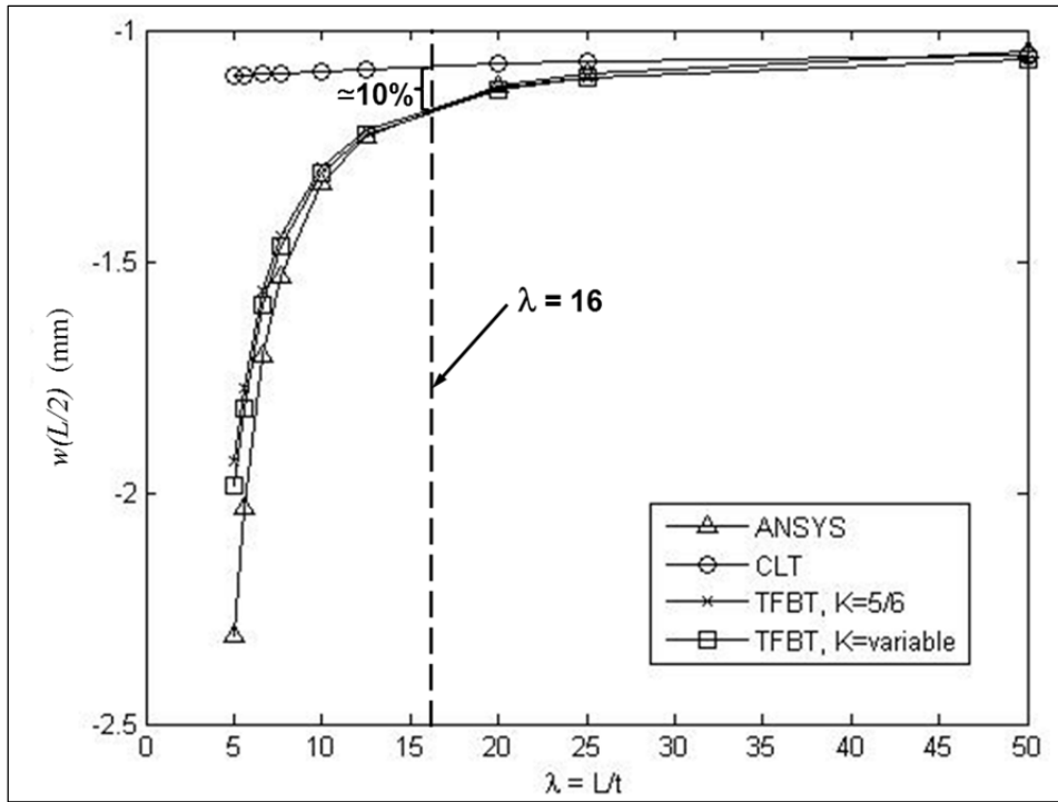
Figure 2.4 Mid-span deflections as a function of \lambda for quasi-isotropic lay-ups
