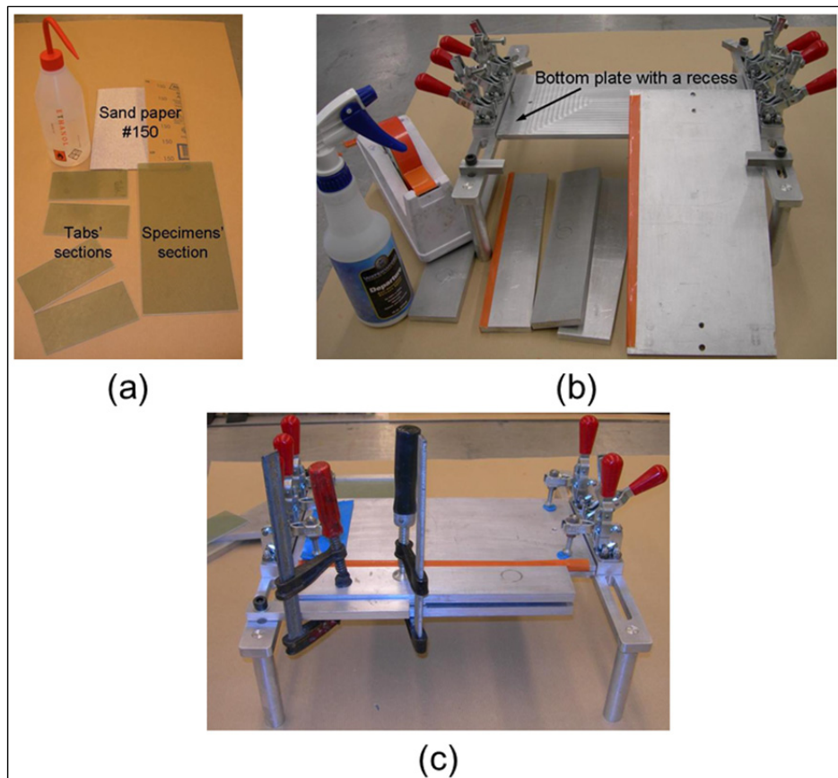
Figure 3.16 Fixture for the assembly of the tabs: (a) Preparation of the tabs material, (b) Preparation of the fixture parts and (c) Gluing the tabs and curing installation
