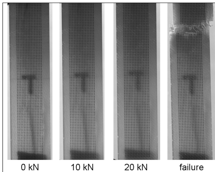
Figure 5.1 Pictures of the methodology using a grid of points
