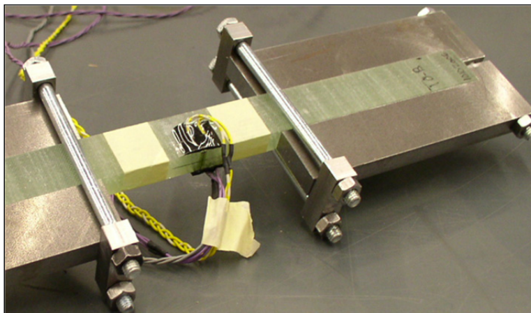
Figure 3.24 Thick specimen for a longitudinal tensile test with lateral supports
