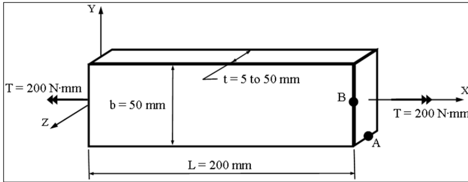
Figure 5.4 Rectangular bar in torsion
