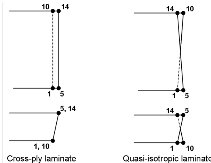
Figure 4.11 Disturbed cross sections due to axial loading
