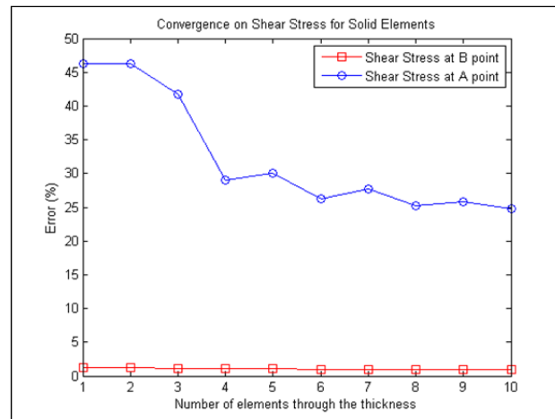
Figure 5.8 Convergence on shear stress for solid elements
