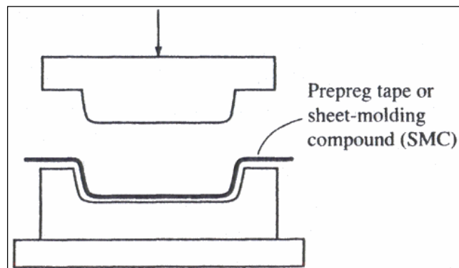
Figure 1.5 Compression moulding process Drawn from Gibson (2007)
