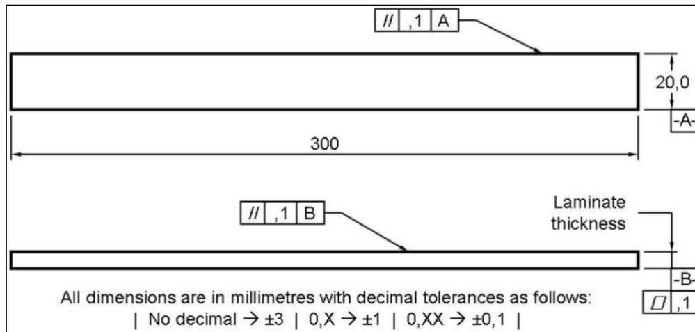
Figure 3.23 Geometry of longitudinal tensile specimen
