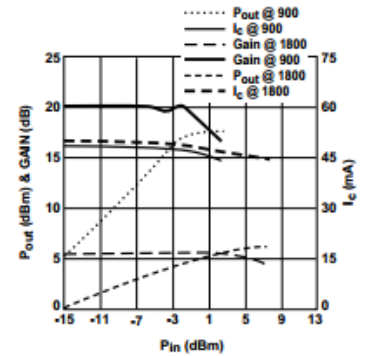
Figure 9. P_{out} (dBm), Gain (dB), and I_c (mA) vs. P_{in} (dBm) at 2 V, 50 mA. 900 MHz: \Gamma_S : Mag: 0.68, Ang: 121°; \Gamma_L : Mag: 0.38, Ang: 171° 1800 MHz: \Gamma_S : Mag: 0.44, Ang: 158°; \Gamma_L : Mag: 0.28, Ang: 159°
