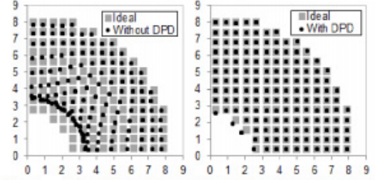
Fig. 4 Comparison of the resulting constellation without/with digital predistortion (DPD) and the expected constellation.
