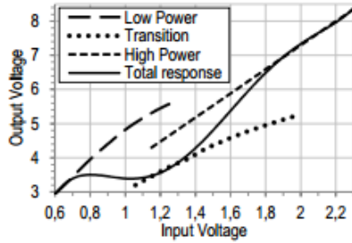
Fig. 2 Voltage input to output response of the proposed reconfigurable amplifier architecture.
