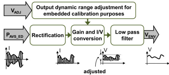
Fig. 2. Envelope Detector block diagram.
