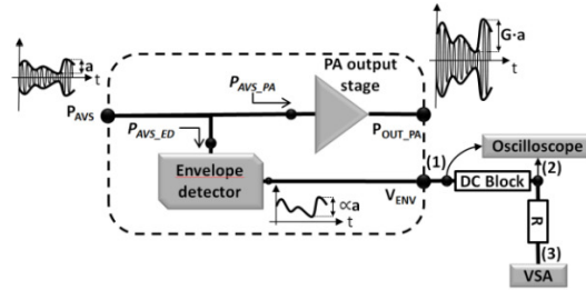
Fig. 5. Schematic highlighting the measurement nodes: (1) for the detector's static transfer function; (2) for the output voltage swing with time; (3) for frequency response.
