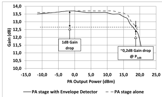
Fig. 9. Gain of output PA stage compared to the gain of the output PA stage with the envelope connected at the input.
