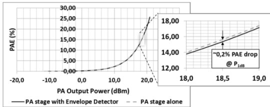
Fig. 10. PAE of output PA stage compared to the PAE of the output PA stage with the detector connected at the input.
