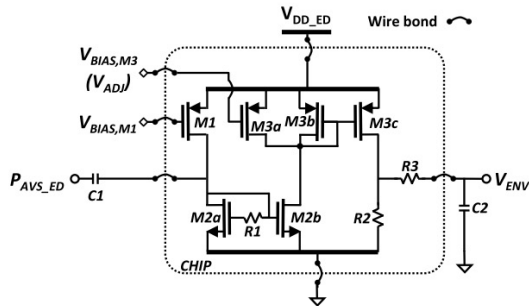
Fig. 3. Envelope detector circuit schematic
