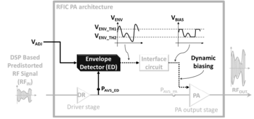
Fig. 1. Investigated RFIC PA architecture (in light gray) requiring the envelope detector presented in this paper (in darker shade).
