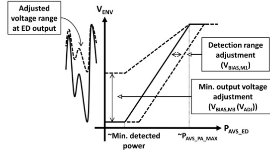
Fig. 4. Ideal detector conversion gain profile illustrating possible adjustments for embedded calibration.
