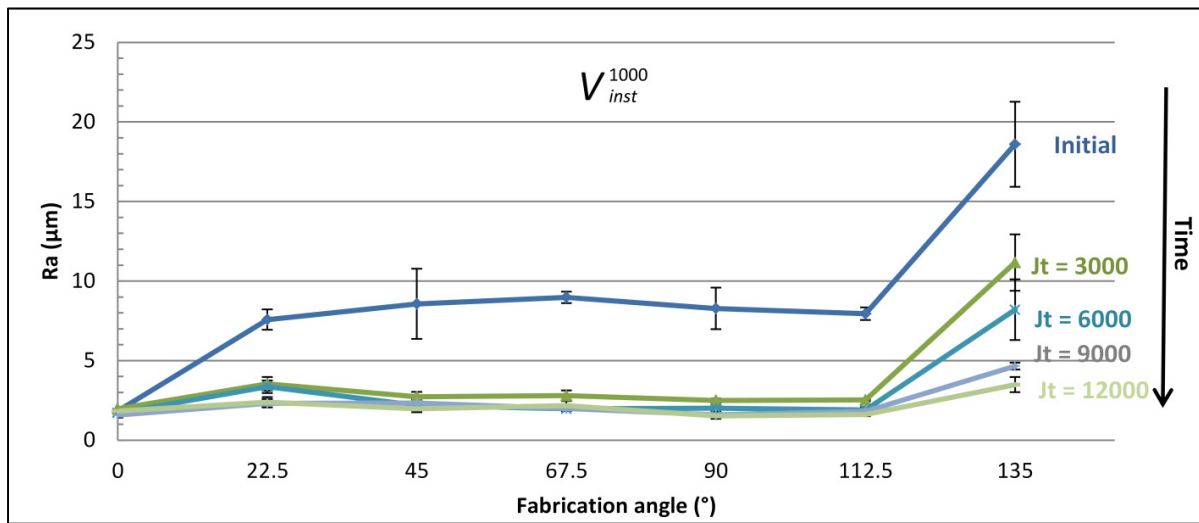
Figure 3.13: Ra evolution of barrel staves during electropolishing ( V_{inst}^{1000} )
