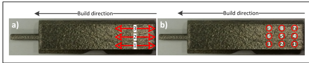
Figure 3.8: Illustration of a) stylus profilometer and b) thickness measurements of stave specimens
