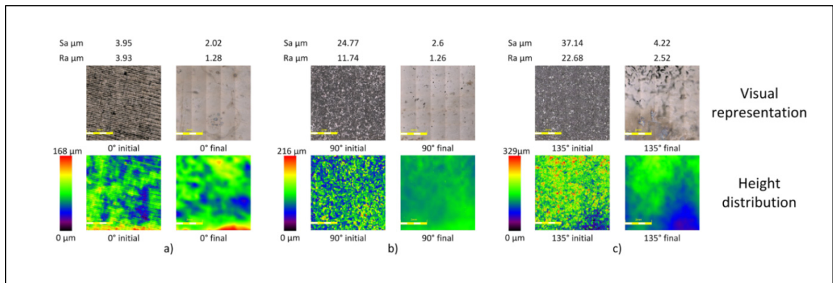
Figure 2.12: Sa surface topography characterization (5000 \mu\text{m} x 5000 \mu\text{m} at 10X) along with stylus profilometry Ra values of the initial and final surfaces of stave shaped specimens oriented at a) 0°, b) 90° and c) 135°
