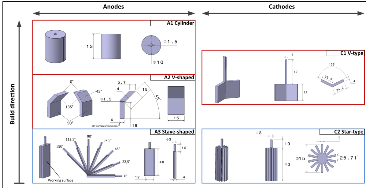
Figure 2.3: Cylindrical-shaped A1, V-shaped A2, and stove-shaped A3 anodes. V-type C1 and star-type C2 cathodes (dimensions in mm)
