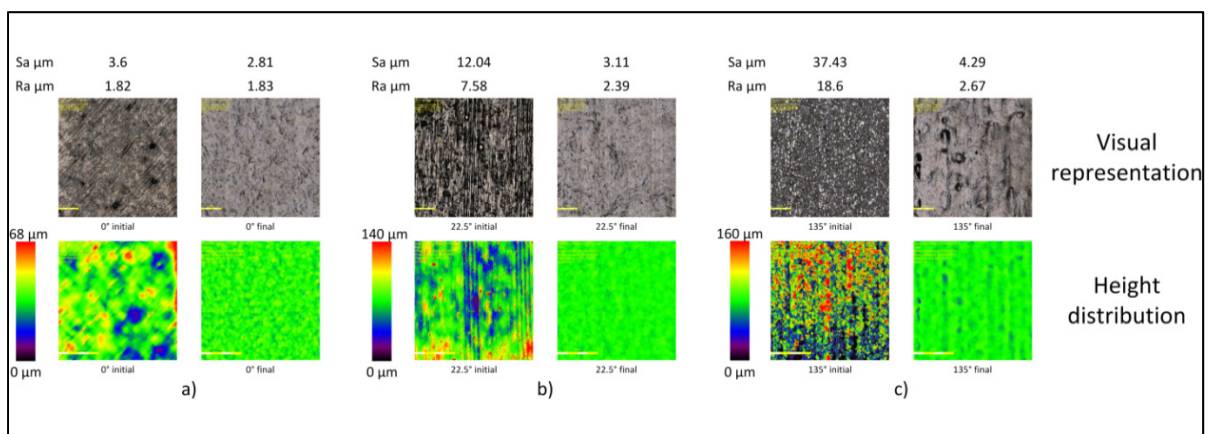
Figure 3.15: Sa surface topography characterization ( 5000\mu\text{m} \times 5000\mu\text{m} at 10X) along with stylus profilometry Ra values of the initial and final surfaces of stave shaped specimens oriented at a) 0, b) 22.5^\circ and c) 135^\circ .
