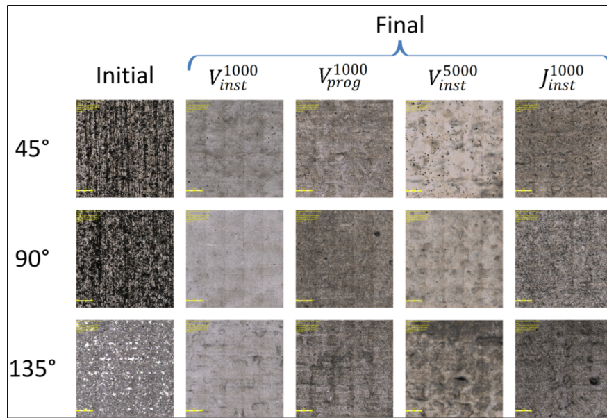
Figure 3.11: Initial and final ( Jt=10000\text{ mA cm}^{-2}\text{ min} ) surface images of V-shaped specimens at 5X ( 2560\text{ }\mu\text{m} \times 2560\text{ }\mu\text{m} )
