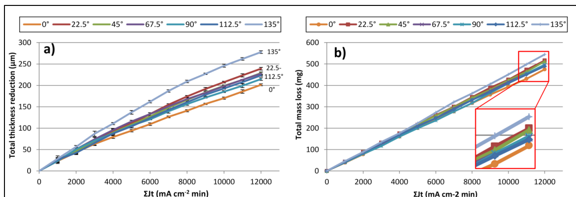
Figure 3.17: Thickness reduction and b) mass loss of barrel staves as functions of time
