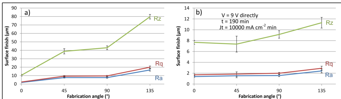
Figure 3.10: R_a , R_q and R_z values: a) before and b) after EP of V-shaped specimens
