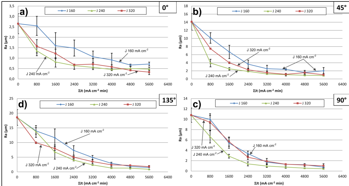
Figure 2.7: R_a evolution after EP of the V-shaped specimens on a) 0^\circ -, b) 45^\circ -, c) 90^\circ - and d) 135^\circ -oriented surfaces, at 3 current densities: 160, 240 and 320 \text{ mA cm}^{-2}
