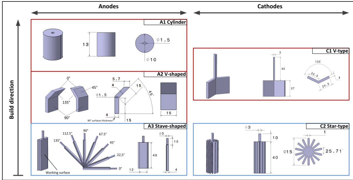
Figure 3.3: Cylindrical-shaped A1, V-shaped A2, and stove-shaped A3 anodes. V-type C1 and star-type C2 cathodes (dimensions in mm)
