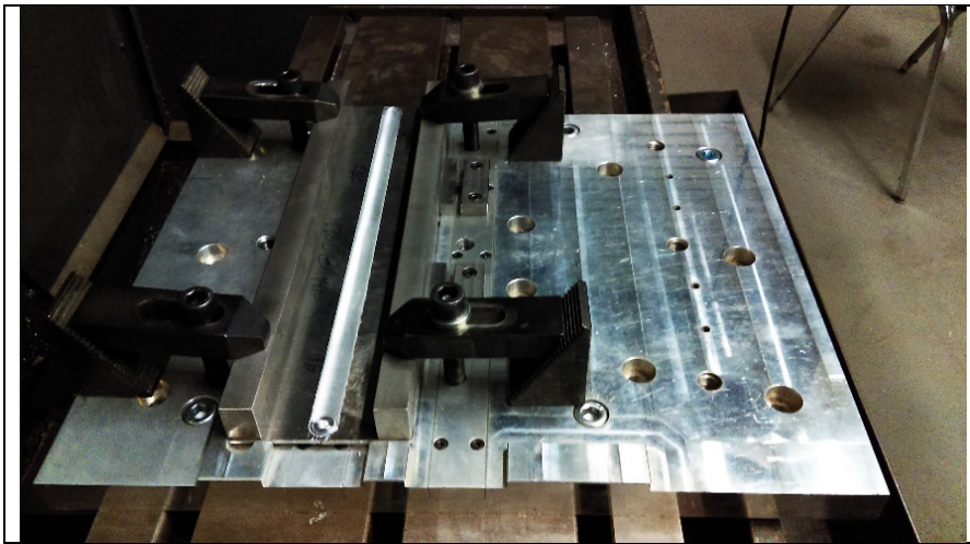
Figure 2.2 Manufactured fixture used for FSW process.
