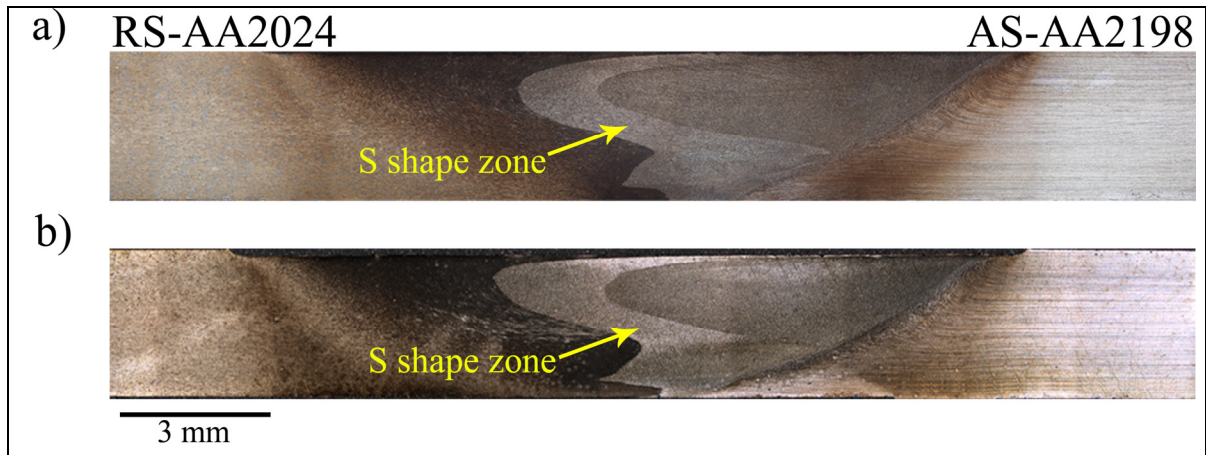
Figure 5.1 Cross-section observations in CWD-ND plane of as-welded samples: a)AW-T3 and b)AW-T8. The both micrograph are similar and S shape zone with lighter color can be seen in the center of nugget.
