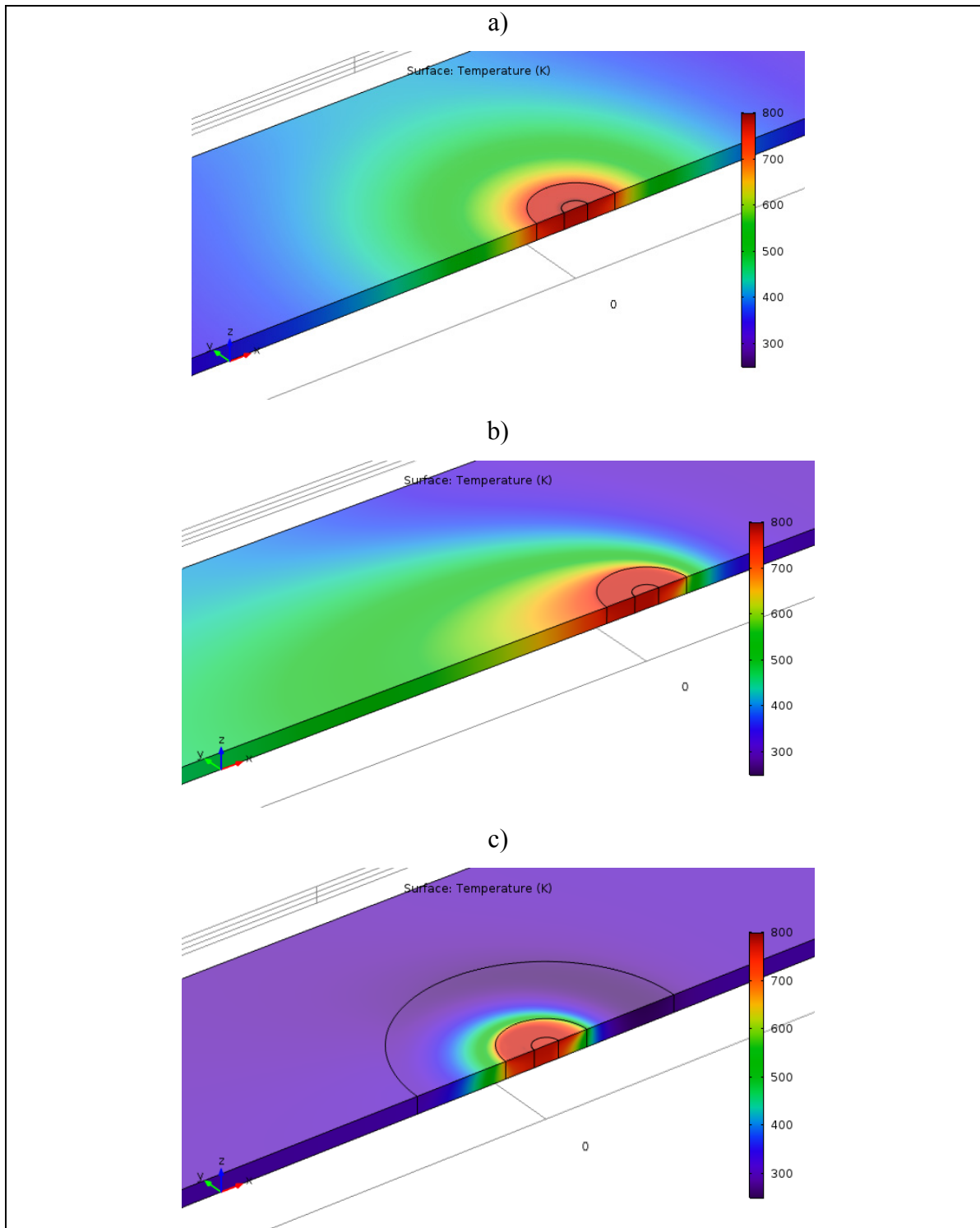
Figure 6.3 Temperature distribution of workpiece in different welding traverse speed and same rotational speed of 750 RPM with and without cooling: a) 50 mm/min b) 450 mm/min c) 450 mm/min with cooling
