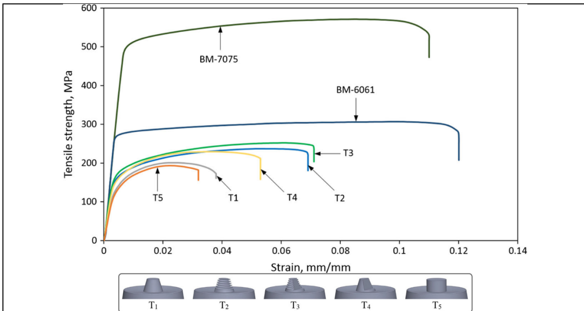
Figure 1.15 Stress–strain curves of the joints between AA7075-AA6061 using the five different pin designs such as cylindrical and tapered, smooth and threaded, flatted and non-flatted (Hasan et al., 2016)
