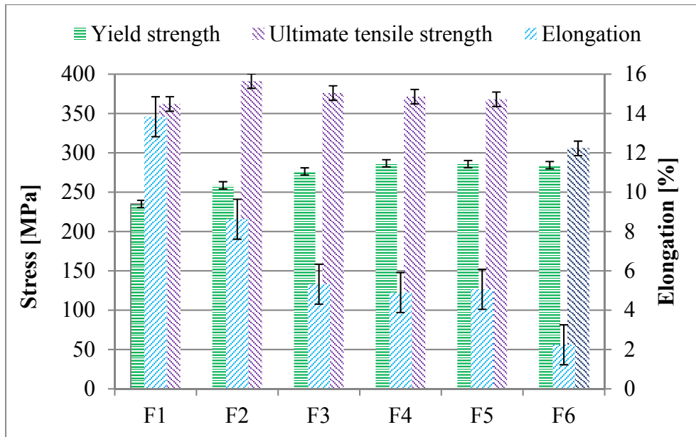
Figure 4.3 Mechanical properties of FSW joints produced by tool F according to welding conditions in Table 2.4 Welding speed parameters.. The parameters of 750 RPM and 450 \text{ mm/min} produced the joint with highest yield strength.
