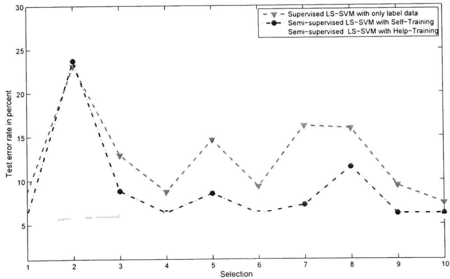
Fig. 3. Correlation between supervised and semi-supervised performance: test error rate obtained on the Gaus50 dataset with respect to each selection.
