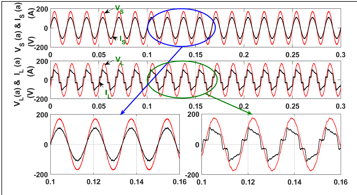
Figure 2.8 Lagging voltage
