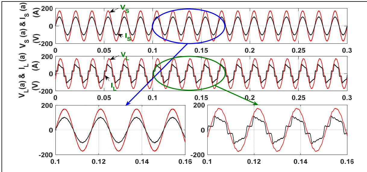
Figure 2.21 Lagging voltage
