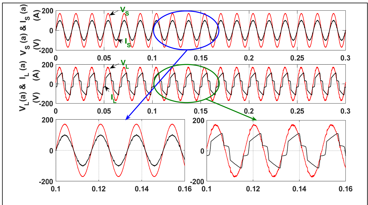
Figure 2.7 Leading voltage
