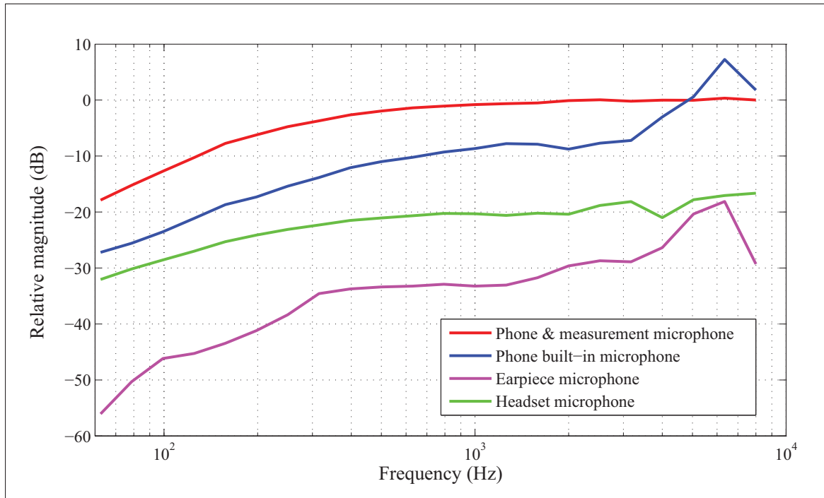
Figure 3.1 Relative magnitude of the frequency of response as subtracted to the magnitude of the reference system measurement frequency response, while measuring Source 3 at 90 dB(A)
