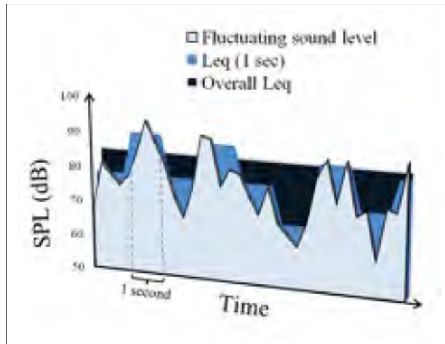
Figure-A II-1 Fluctuating sound pressure level, Overall L_{eq} and short L_{eqs}
