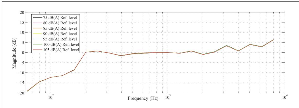
Figure 3.6 Frequency responses of the measurements conducted with the headset with the magnitude normalized at the 1 kHz third-octave band noise level
