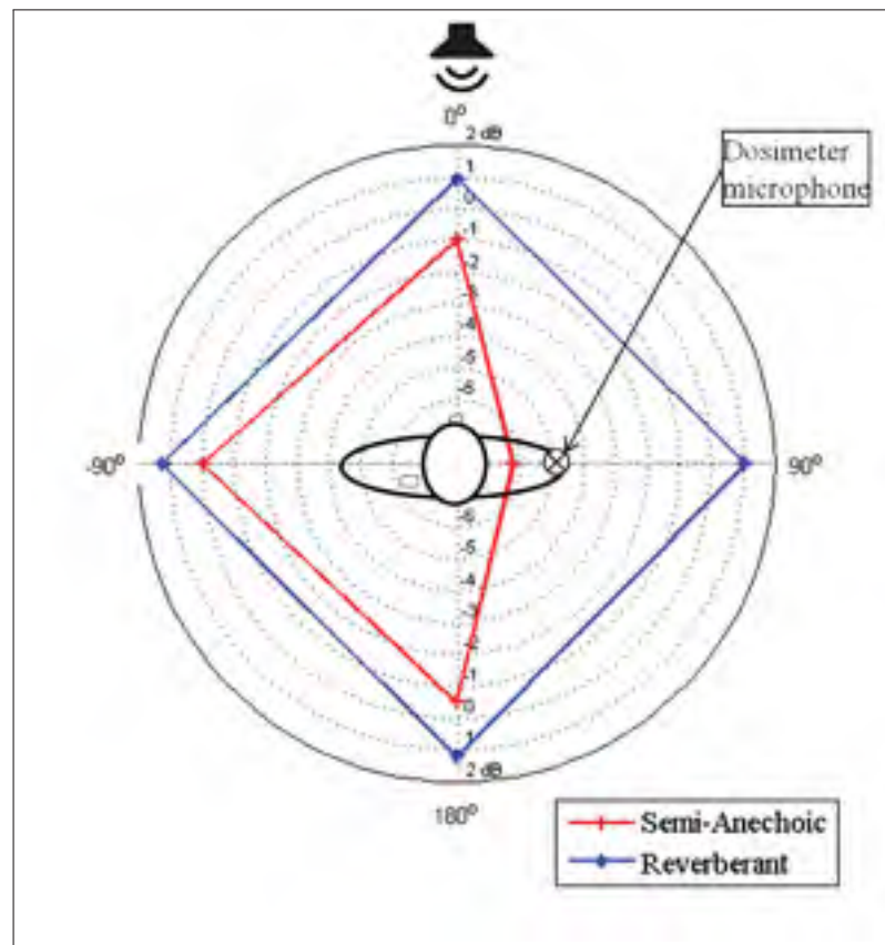
Figure 3.41 Noise dosimeter overall A-weighted errors averaged over the range of noise levels in the semi-anechoic chamber (in red) and in the reverberant chamber (in blue)
