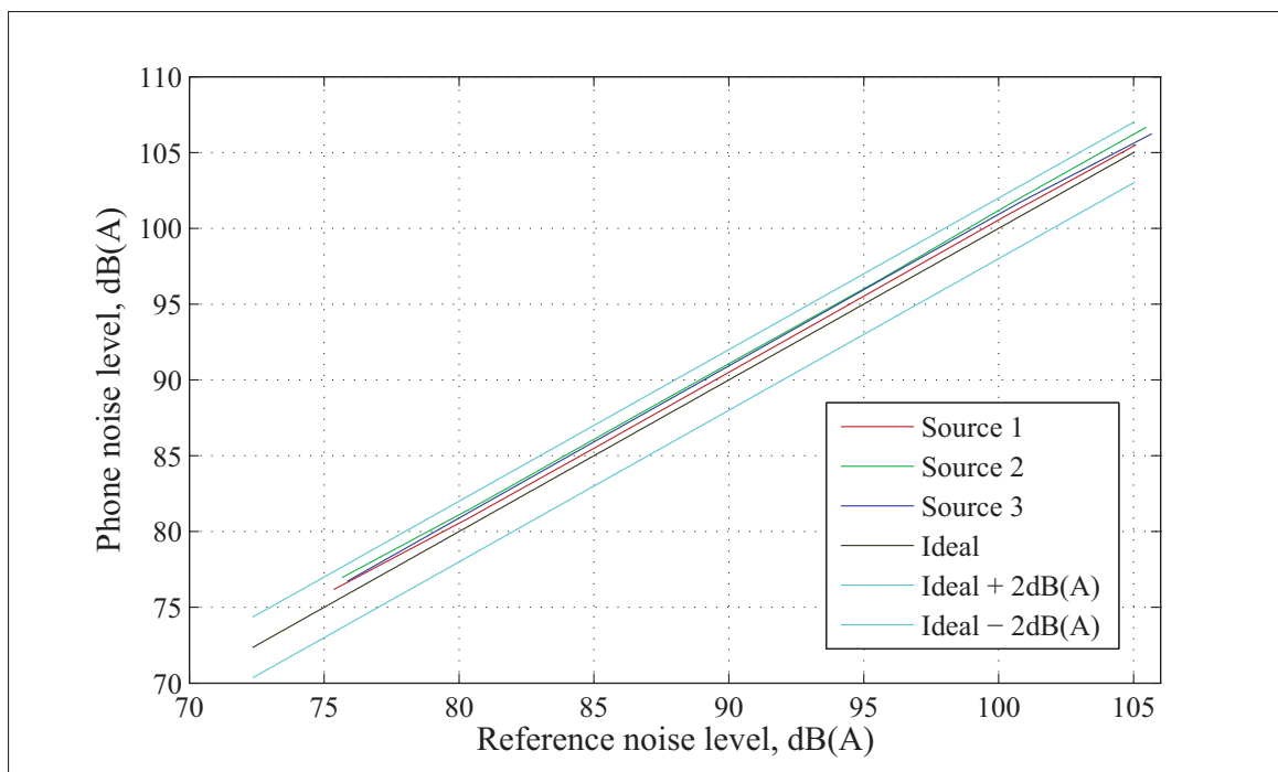
Figure-A IX-3 Calibrated noise levels in dB(A), measured with the headset microphone, right after the calibration measurement
