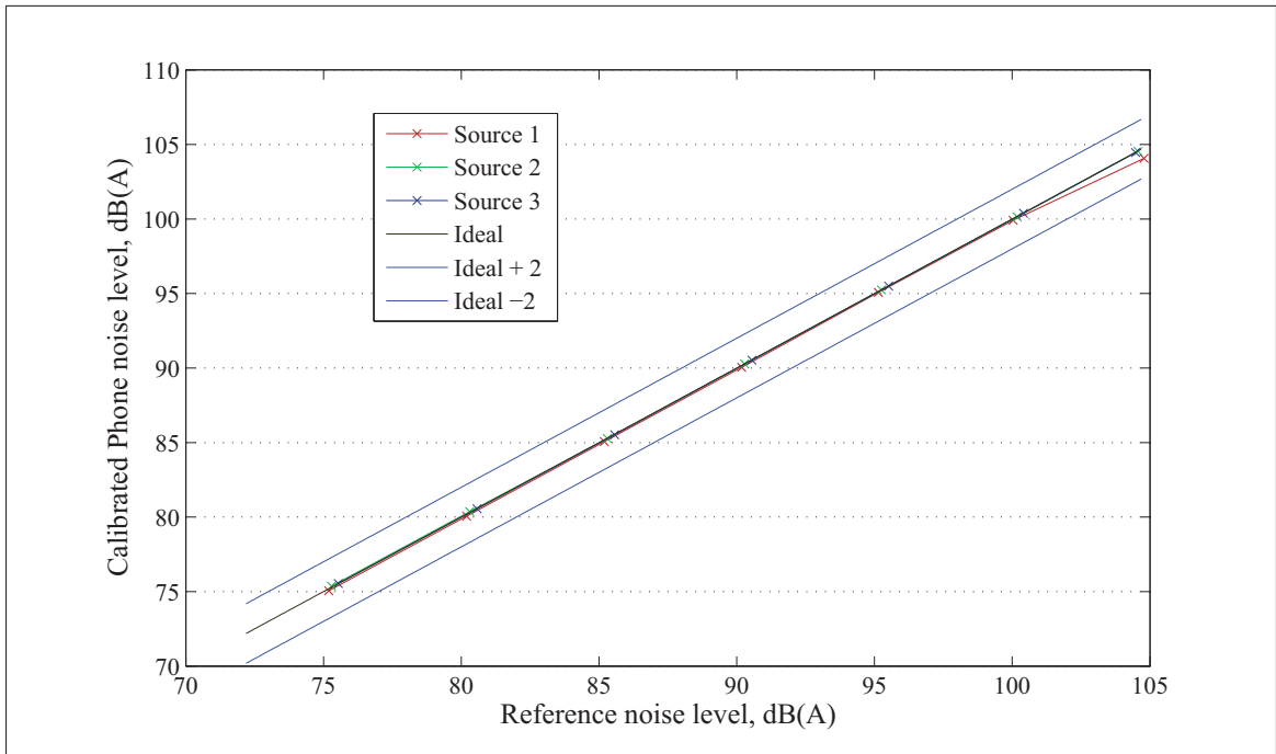
Figure-A IX-1 Calibrated noise levels in dB(A), measured with the headset microphone, right after the calibration measurement
