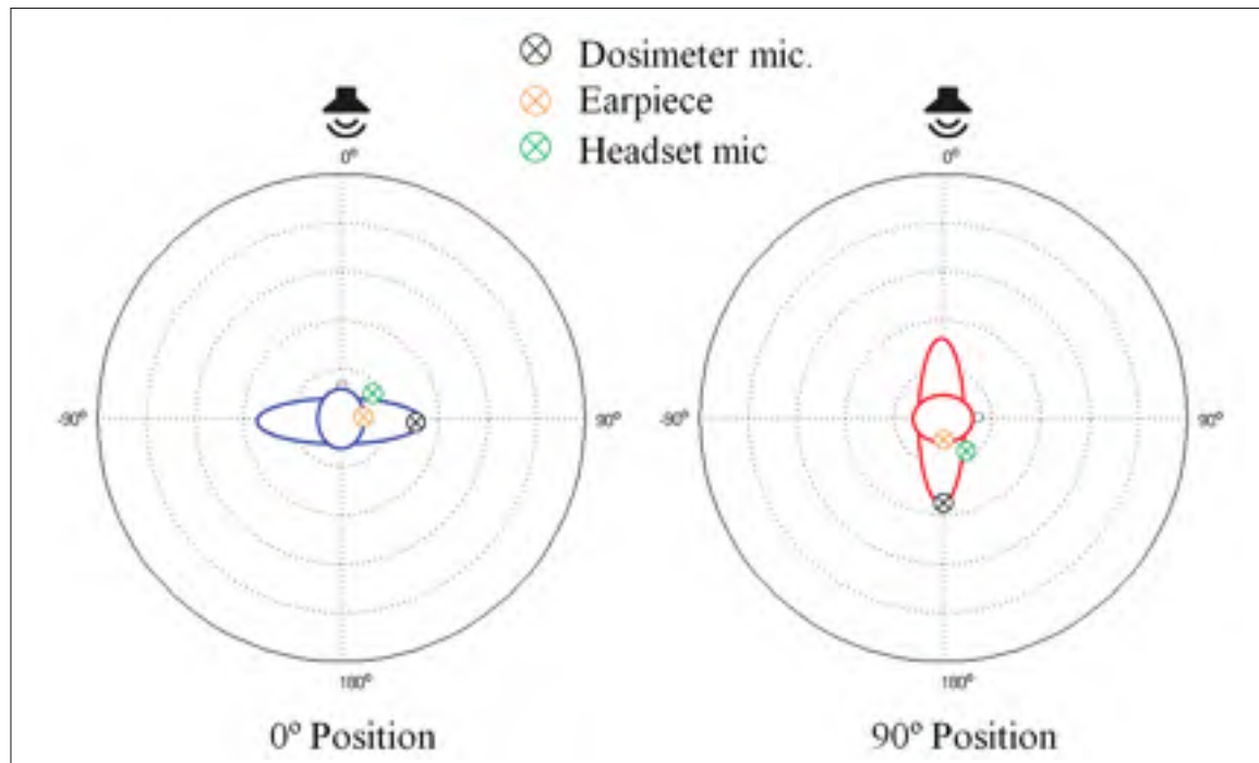
Figure 2.18 Top view of 2 of the 4 ATF positions relative to the source in the semi-anechoic chamber
