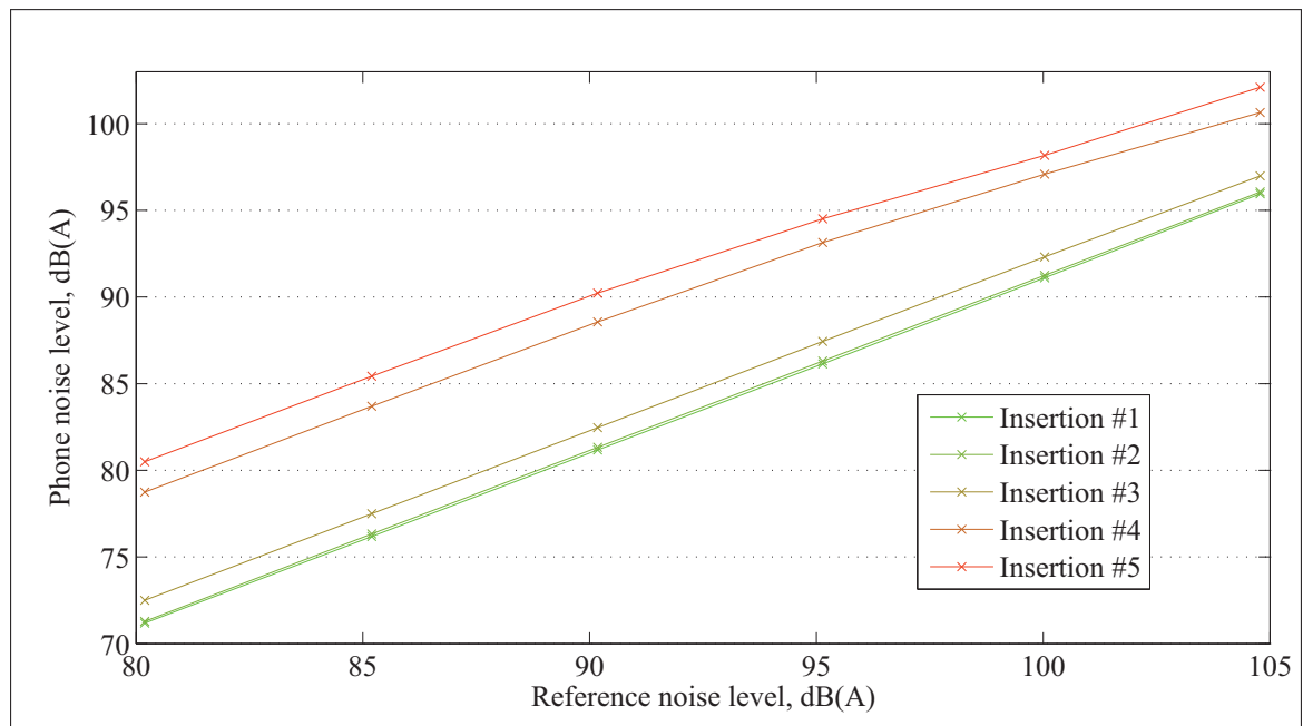
Figure 3.14 Noise level corrections measurements for five variations of earpiece placement within the built-in ear simulator measured in the semi-anechoic chamber
