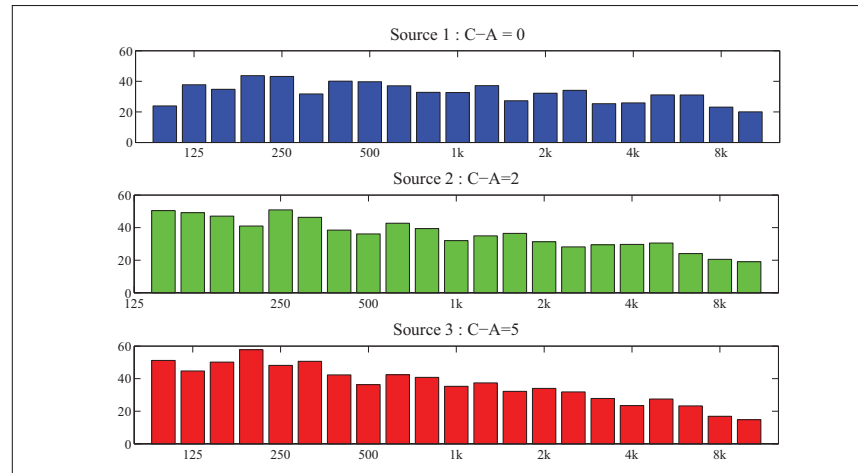
Figure 2.3 Noise spectrum of Sources 1, 2 and 3 with C-A value of 0, 2 and 5 respectively
