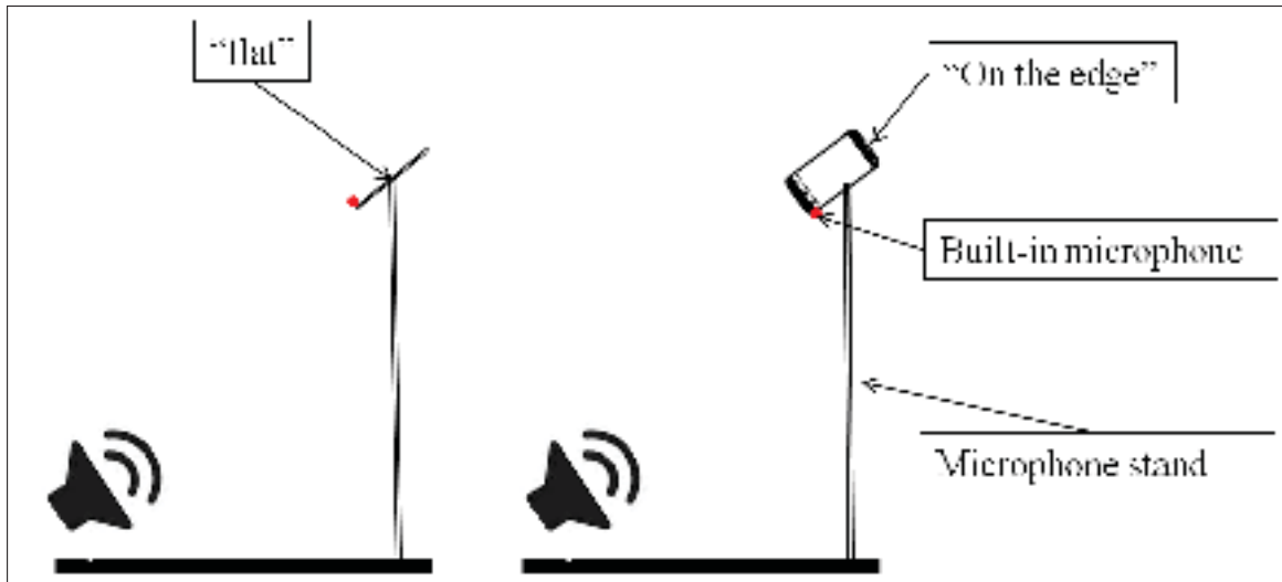
Figure 2.22 Side view of the built-in microphone orientation in the semi-anechoic chamber: mobile phone placed flat (on the left) and on the edge (on the right)
