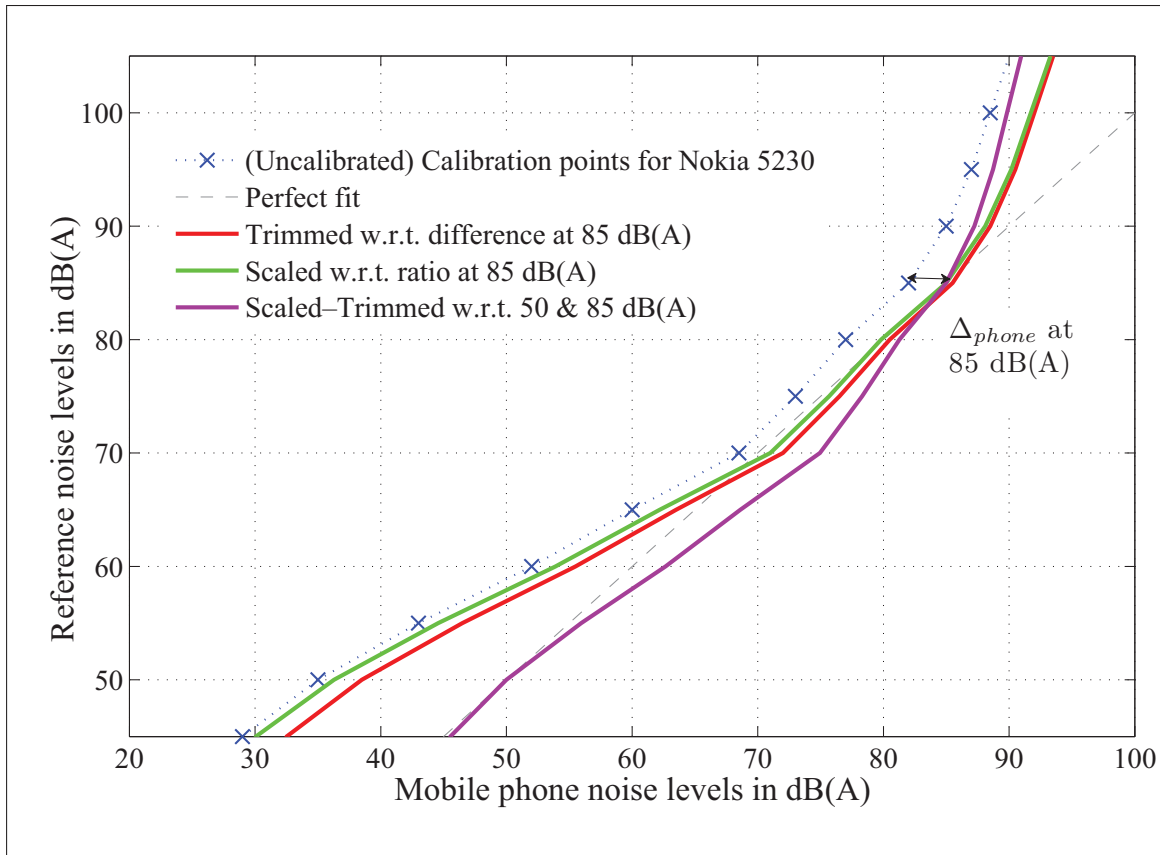
Figure 1.4 Existing calibration methods found in related work, numerically computed for a Nokia 5230 mobile phone, adapted from Stevens (2012)
