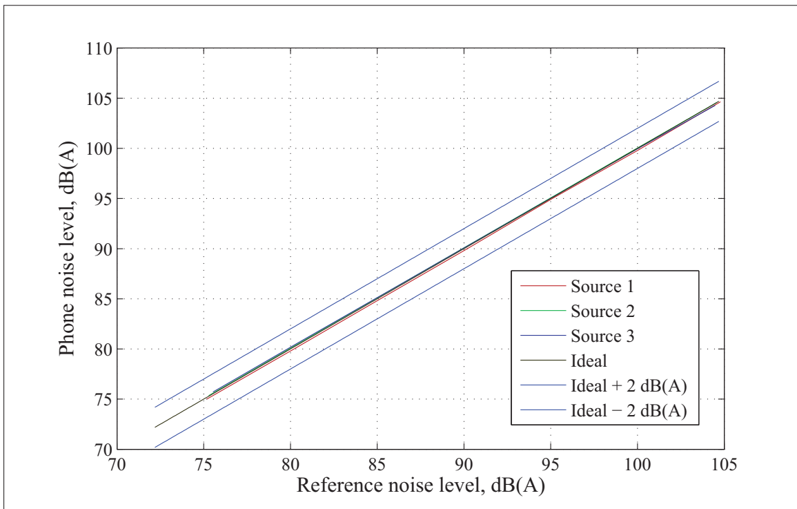
Figure-A IX-2 Calibrated noise levels in dB(A), measured with the headset microphone, right after the calibration measurement
