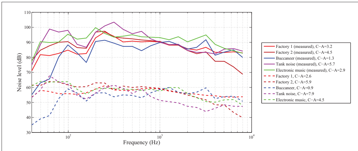
Figure 2.7 Frequency content, in third-octave bands of the original signals of the noise sources used for the validation and the measured noise sources with the reference system in the semi-anechoic chamber
