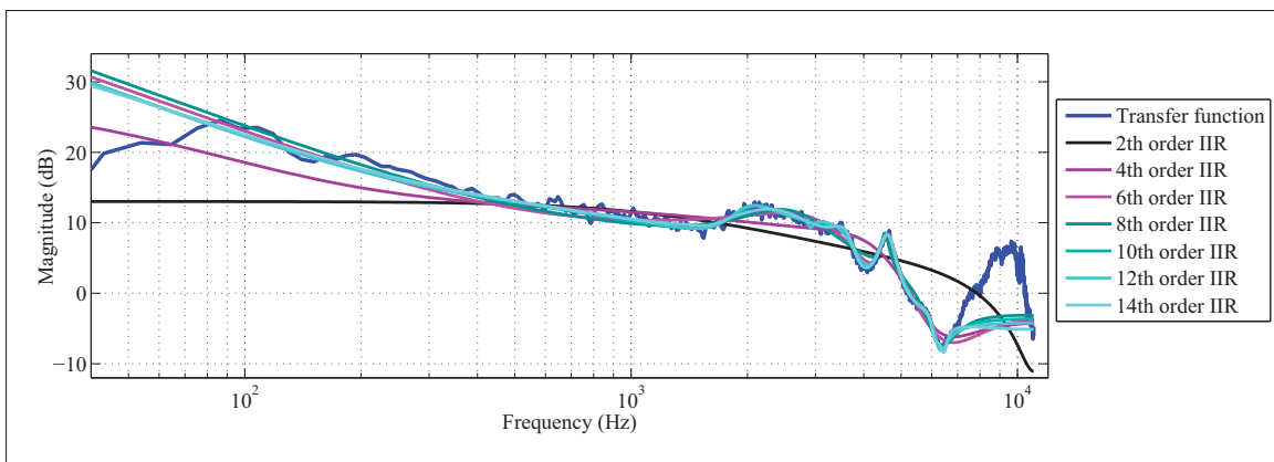
Figure 3.17 Built-in microphone initial transfer function, defined from 0 to 11025 Hz, and frequency responses of IIR filters for orders from 2 to 14, calculated from the truncated-transfer function (from 80 Hz to 6700 Hz)
