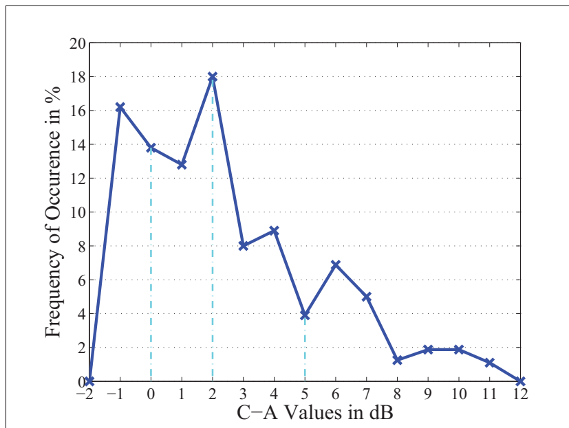
Figure 2.2 Histogram of the C-A values of NIOSH100 noise source database highlighting the 20th, 50th and 80th percentile of the C-A values distribution: 0, 2 and 5 respectively
