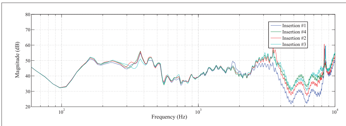
Figure 3.9 Transfer functions calculated from the earpiece measurements with slight variations of the earpiece placement within the built-in ear simulator
