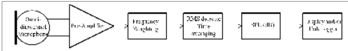
Figure-A III-1 Simplified block diagram of a sound level meter
