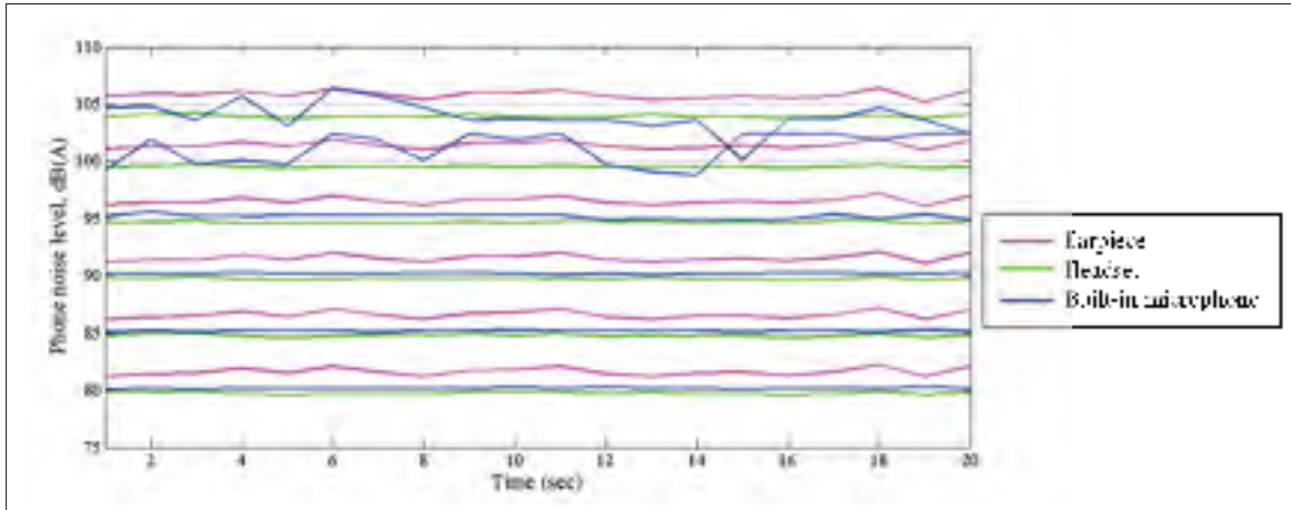
Figure 3.28 Built-in microphone, headset and earpiece L_{eq,A,1sec} , measured during the validation measurements for 6 noise levels
