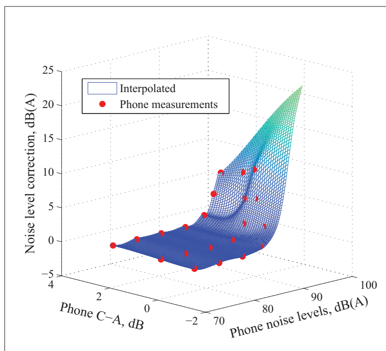
Figure-A VII-3 Built-in microphone measured noise level correction values (in red) and interpolated values with the griddata MATLAB function and its v4 method
