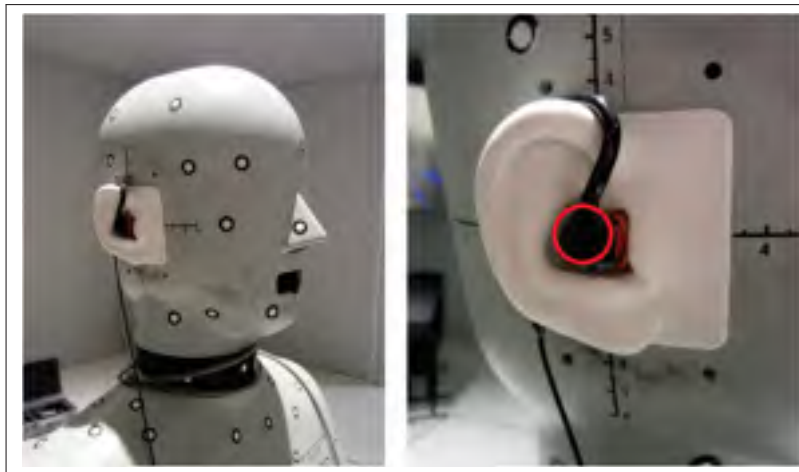
Figure 2.13 Sonomax® earpiece on the ATF's built-in ear simulator with the location of microphone encircled in red
