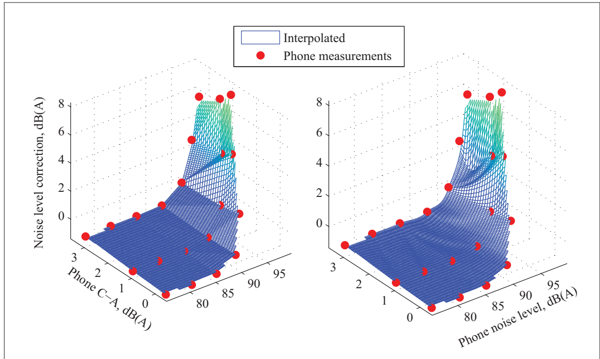
Figure-A VII-1 Built-in microphone measured noise level correction values (in red) and interpolated values with the griddata MATLAB function and the linear and cubic methods
