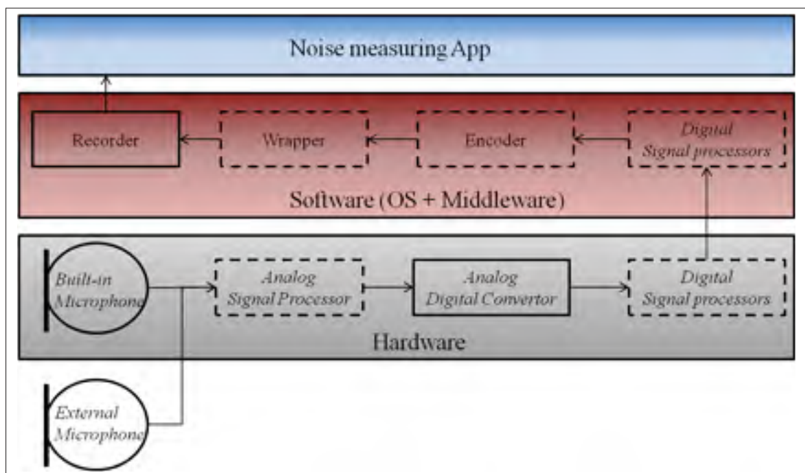
Figure 1.2 Hardware and software components of the audio recording path of mobile phones
