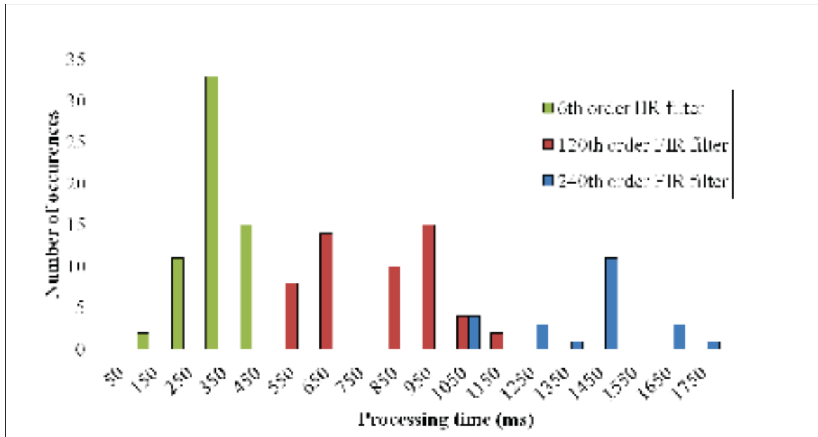
Figure 3.23 Histogram of the processing time required by the mobile phone app to compute a L_{eq,A,1sec} over a one-minute-measurement and depending on the IIR and FIR filters order
