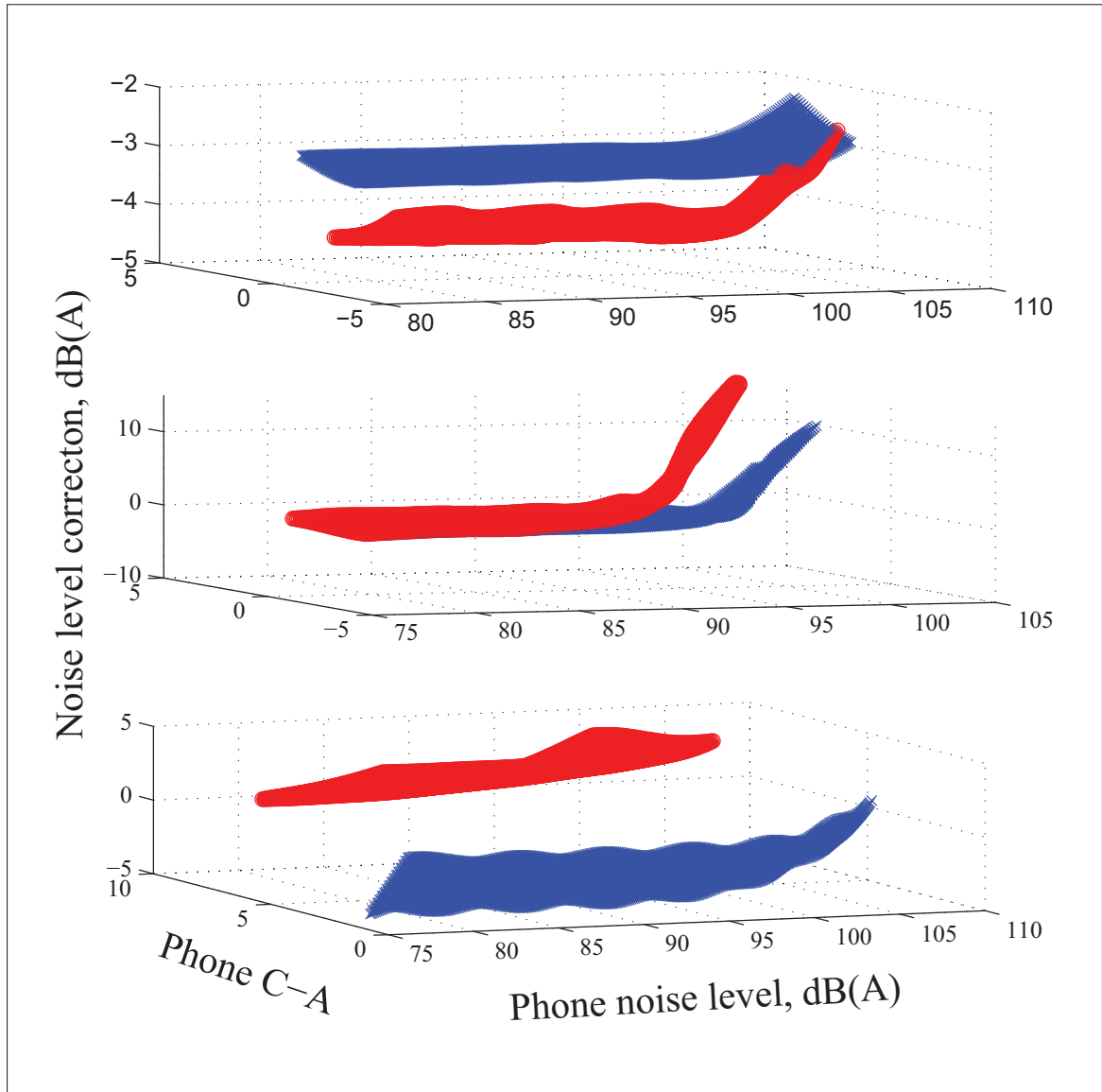
Figure 3.12 3D views of the interpolated noise level corrections measured in the semi-anechoic (in red) and reverberant (in blue) chambers for the headset (top), built-in (middle), and earpiece (bottom) microphones
