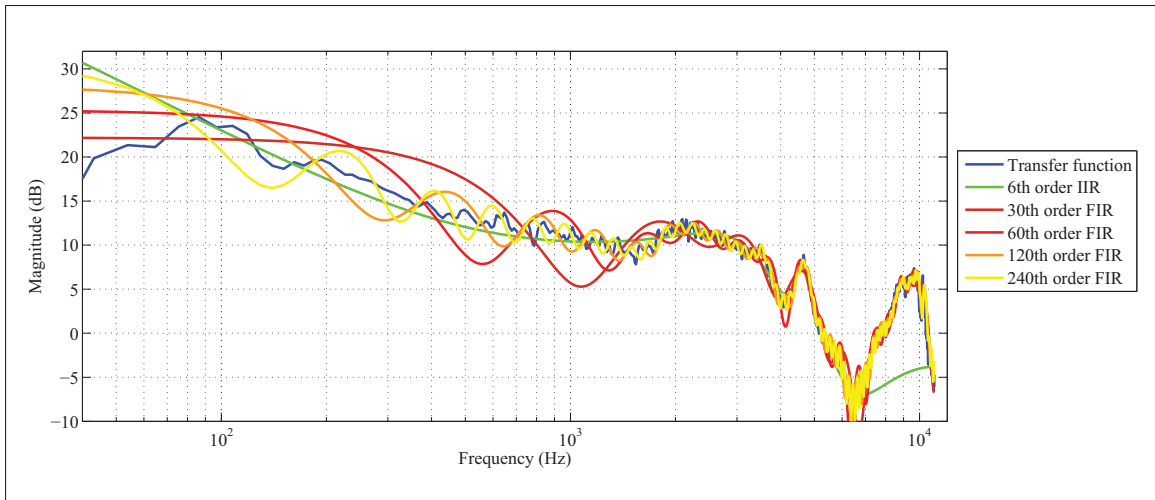
Figure 3.21 Frequency responses of IIR calculated from the truncated-transfer functions and frequency responses of FIR filters for orders from 30 th to 240 th order based on the initial built-in microphone transfer function
