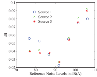
FIGURE 5: Uncertainty associated with the dB(A) phone measurement, u_{LP_{A,phone}} in dB
