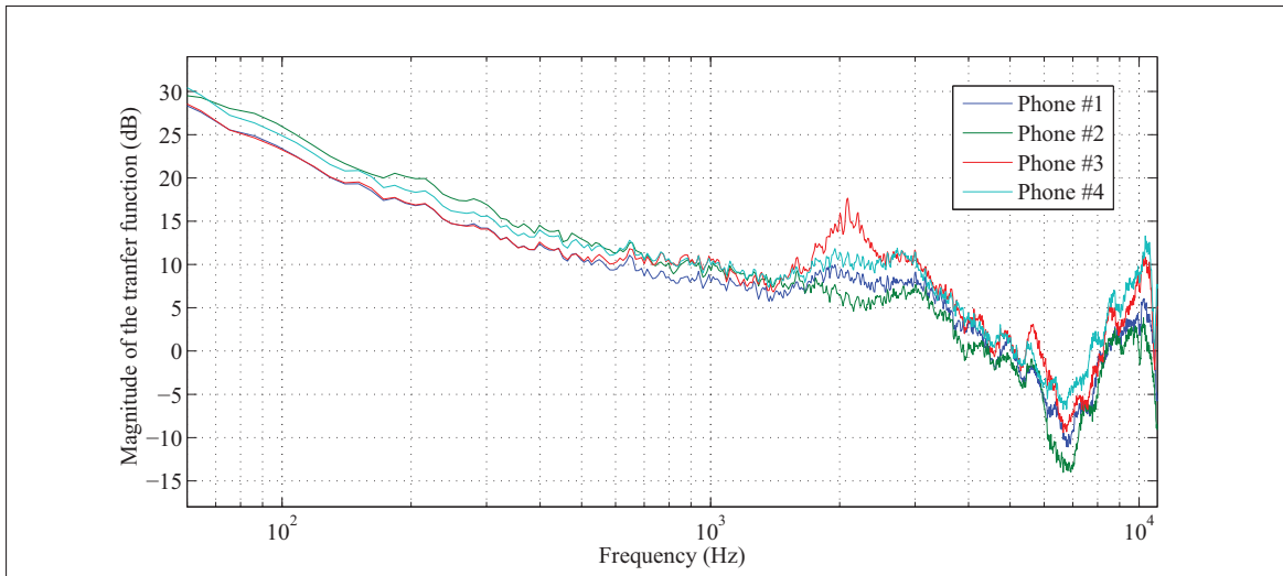
Figure 3.10 Transfer functions calculated from the built-in microphone measurements of the 4 ZTE N762 mobile phone units
