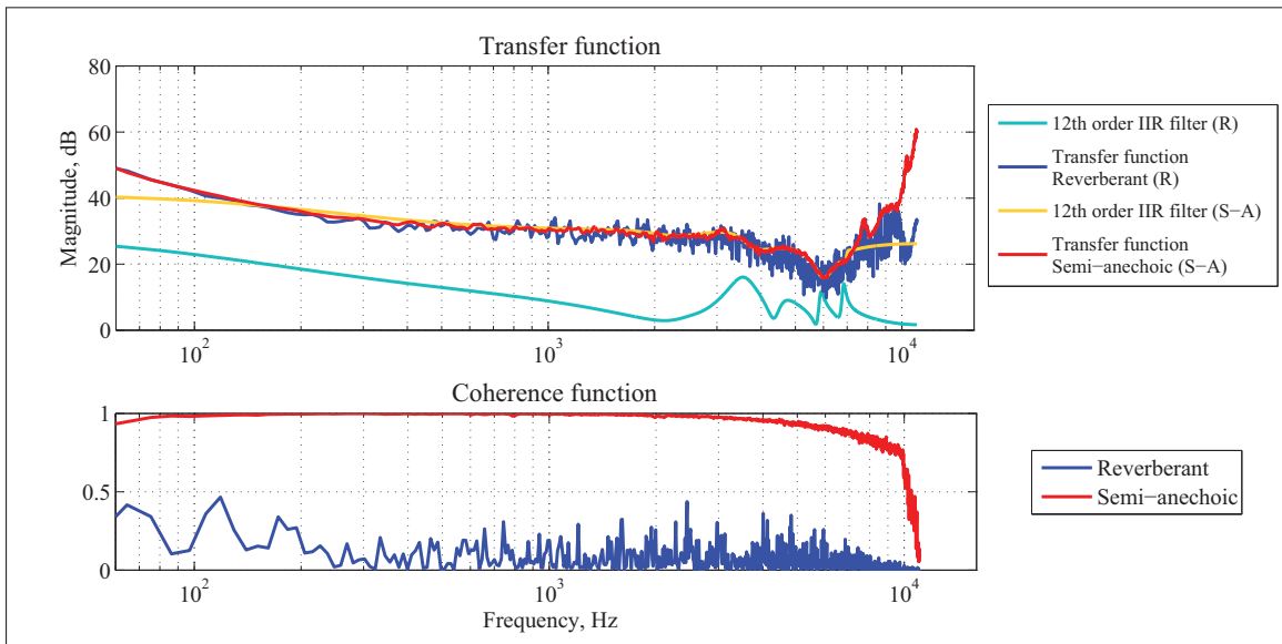
Figure 3.22 Earpiece transfer function and coherence values, frequency responses of 12 th order IIR filters
