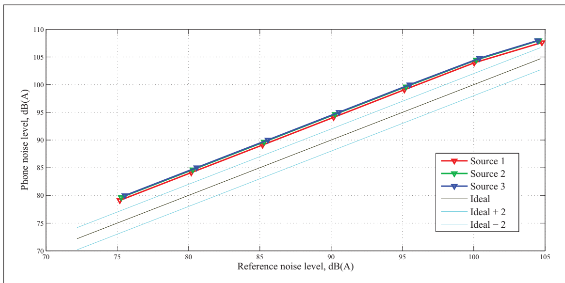
Figure-A VIII-4 Phone noise levels measured with the headset, as compared with the reference noise levels while measuring Source 1, 2 and 3 in the semi-anechoic chamber with the phone implementing the frequency-dependent calibration algorithm
