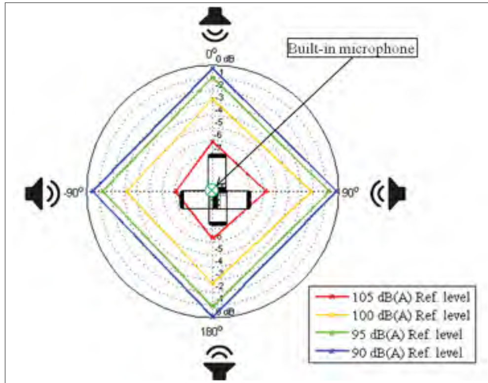
Figure 3.35 Built-in microphone overall A-weighted errors for various microphone placement and noise levels, while measuring Source 1 in the reverberant chamber
