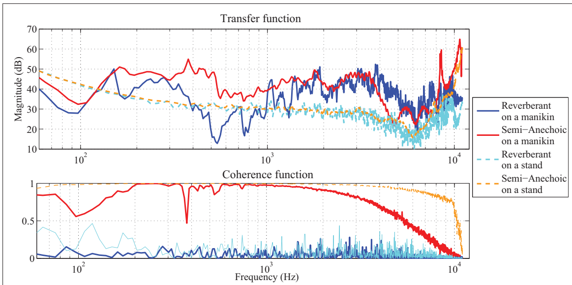
Figure 3.11 Transfer function and coherence values calculated from earpiece measurements in the semi-anechoic and reverberant chambers with the earpiece on a stand and on the ATF
