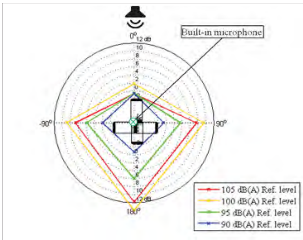
Figure 3.34 Built-in microphone overall A-weighted errors for various microphone placement and noise levels, while measuring Source 1 in the semi-anechoic chamber
