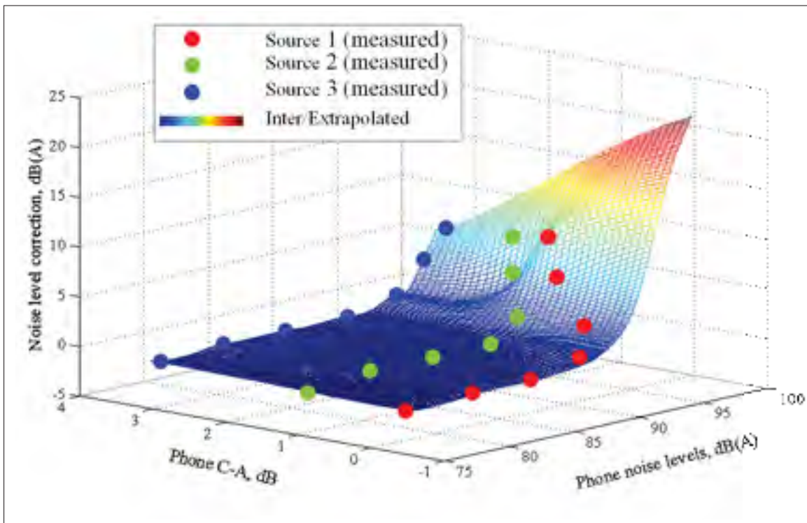
Figure 4.1 Built-in microphone noise level correction values measured in the semi-anechoic chamber (colored dots) and interpolated values calculated using the v4 method
