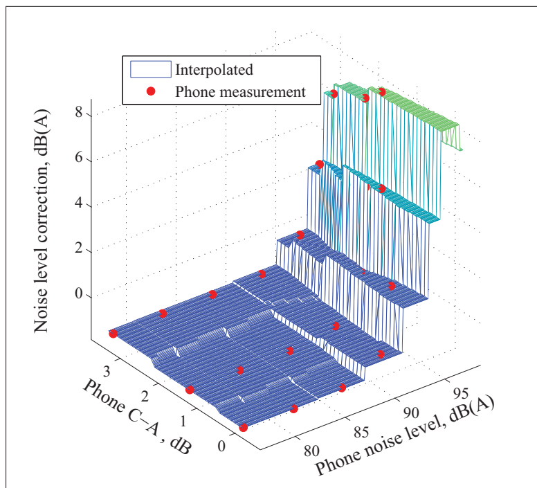
Figure 3.26 Measured built-in microphone noise level correction values (in red) and interpolated values with the griddata MATLAB function and its nearest method
