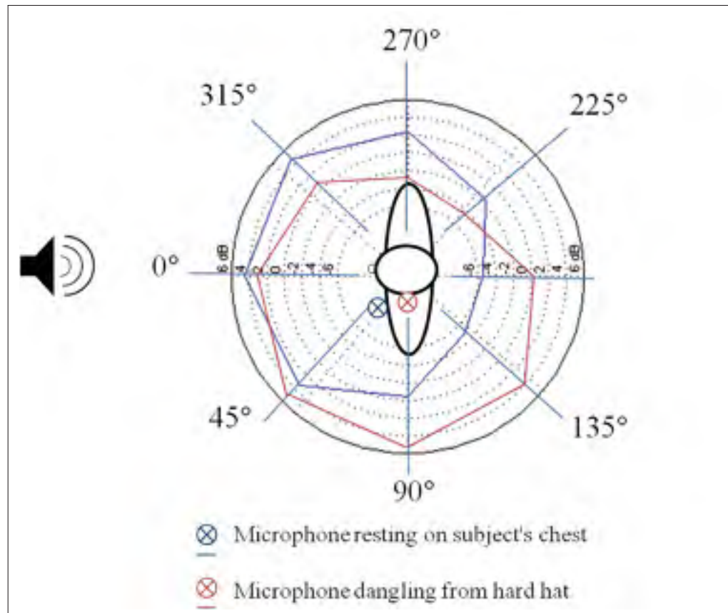
Figure 1.11 Mean A-weighted microphone placement errors (in dB) for the "Left-Chest" and "Left-Hanging" positions, adapted from Byrne and Reeves (2008)
