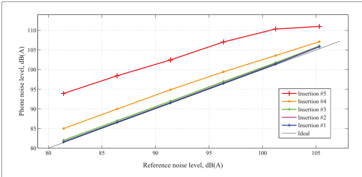
Figure 3.38 Noise level measurements for five variations of earpiece placement within the built-in ear simulator measured in the semi-anechoic chamber
