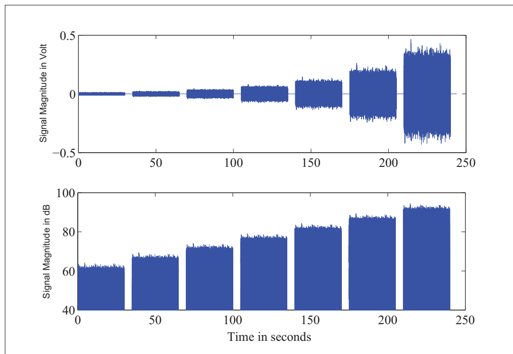
Figure 2.4 Sequence of 7 30-second signals of Source 1 with the noise level increasing by 5 dB every time and with a 5 second silence between each signal
