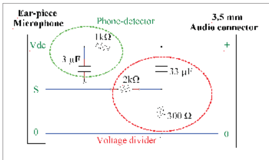
Figure 2.11 Electronic schematic of the adaptor cable with the circuit of the voltage divider and the phone-detector
