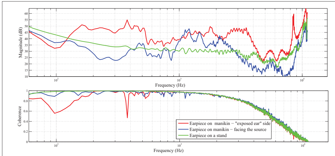
Figure 3.7 Transfer function and coherence values from the measurements conducted with the earpiece located on a microphone stand and for two positions on the ATF
