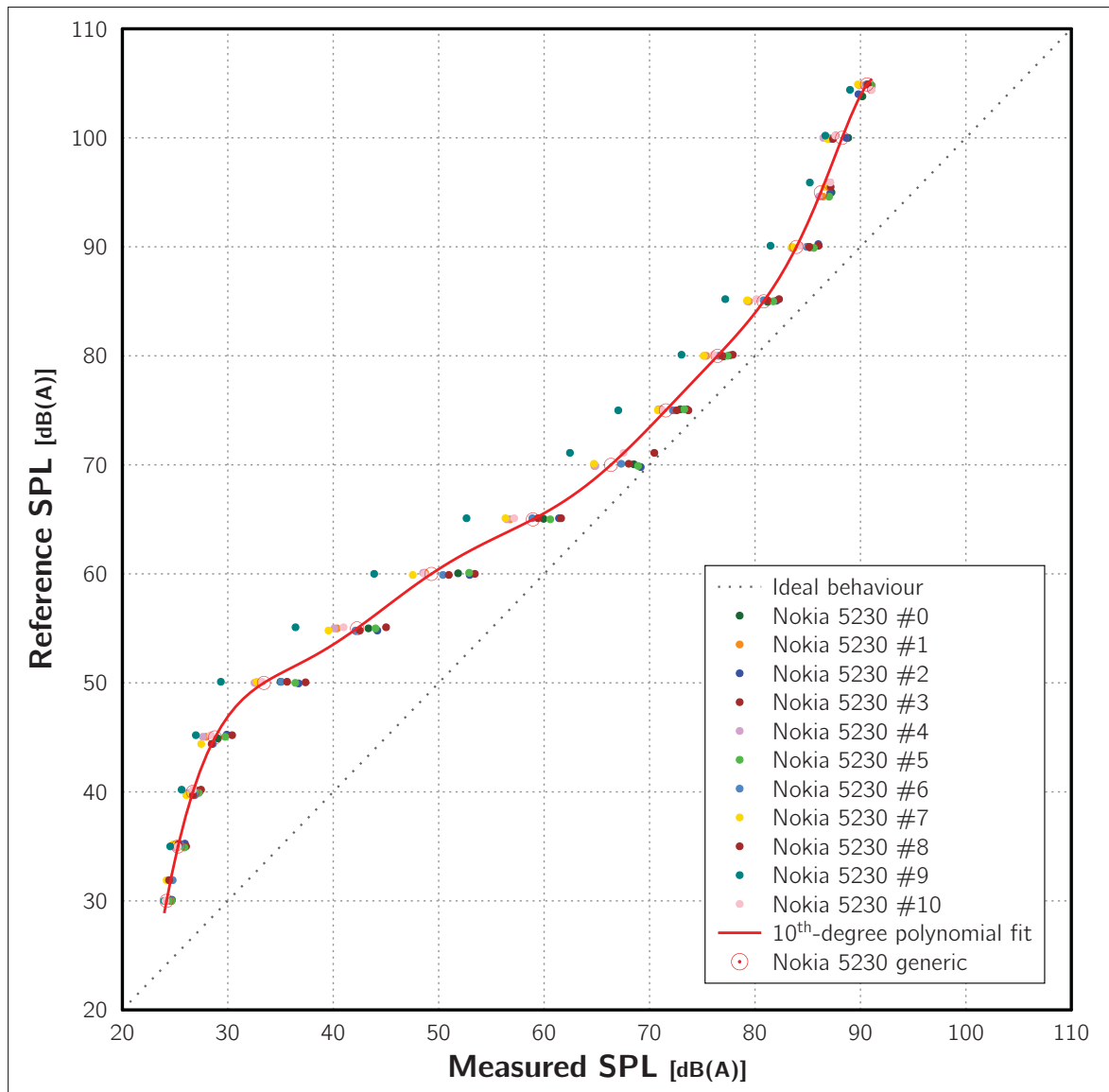
Figure 1.5 Calibration points for our 11 Nokia 5230 handsets (based on white noise calibration), plus the “average” calibration points for a generic Nokia 5230. Reproduced with the permission from Stevens (2012)
