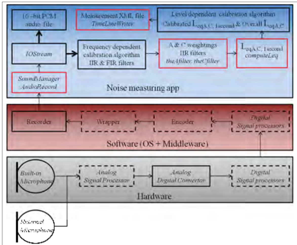
Figure 2.8 Audio processing components of the mobile phone and the noise measuring app, red boxes represent the components and classes that come from the NoiseTube Android app code source
