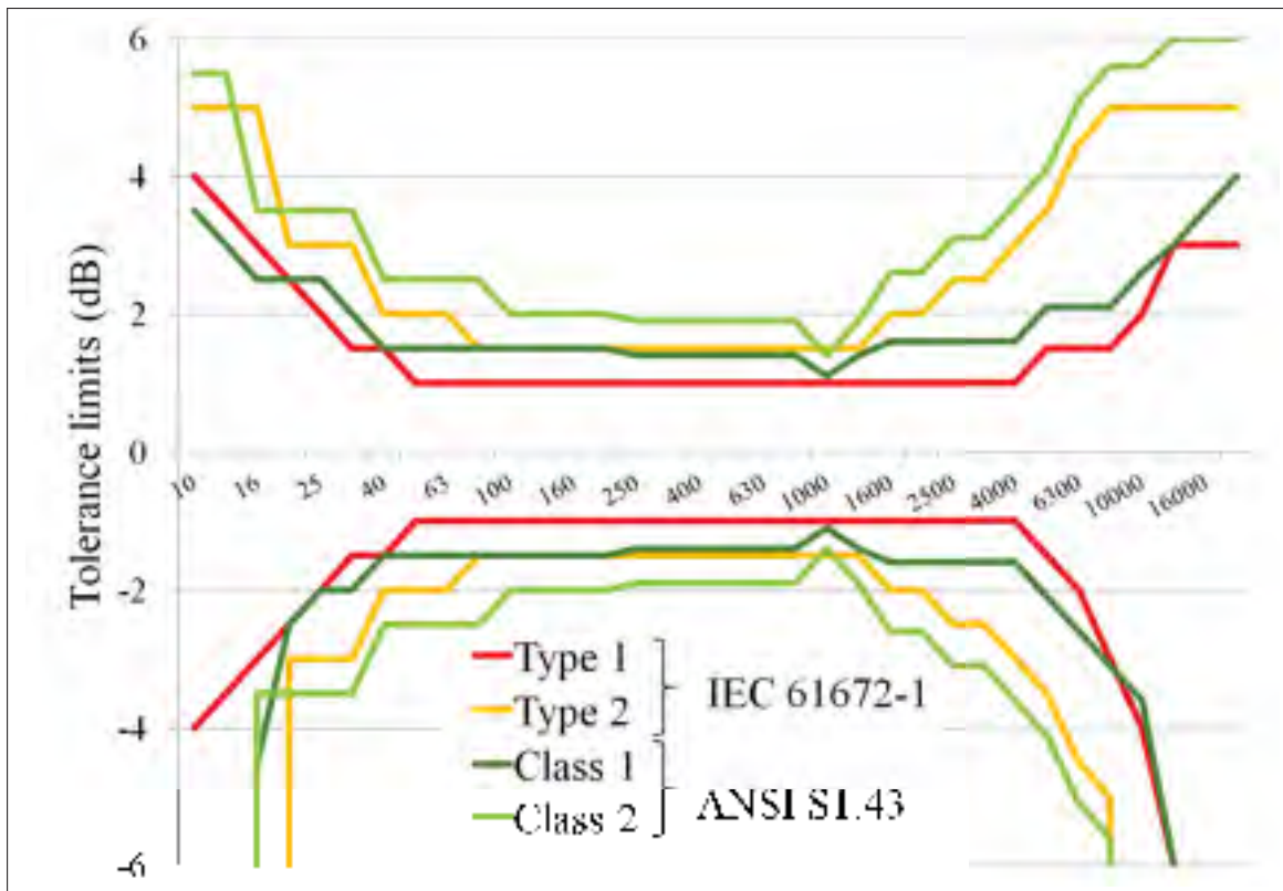
Figure-A III-3 Sound level meter frequency weightings' tolerance limits from ANSI (2007b) and IEC (2002)
