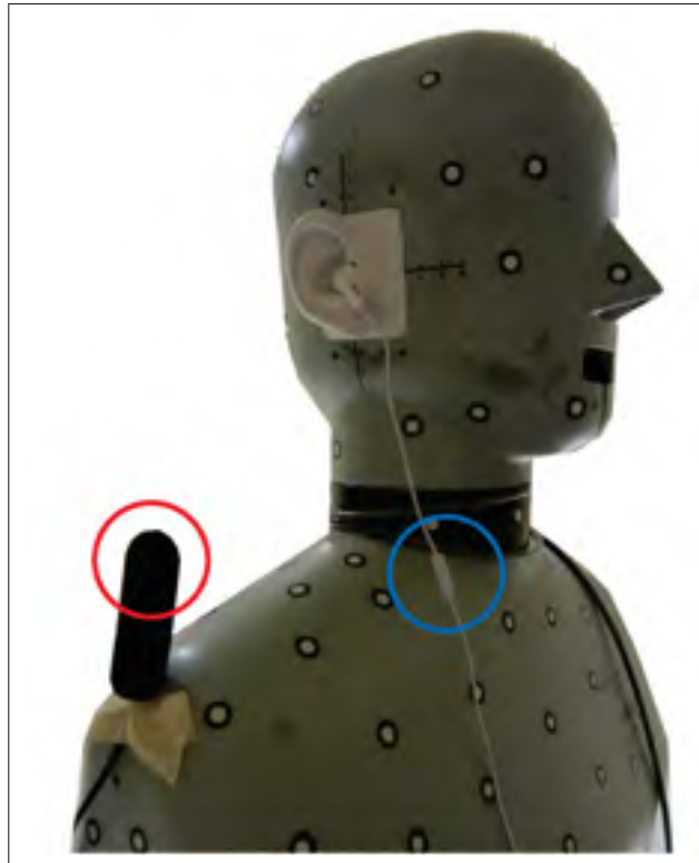
Figure 2.14 Placement of the Apple iPhone ® headset microphone (encircled in blue), and the standardized noise dosimeter (encircled in red) on the ATF
