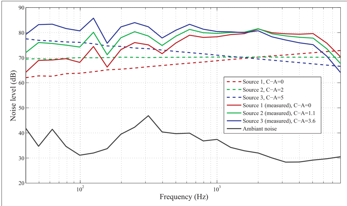
Figure 2.6 Frequency content, in third-octave bands of the ambient noise, the original signals of Sources 1, 2 and 3 and the measured Sources 1, 2 and 3 with the reference system in the reverberant chamber
