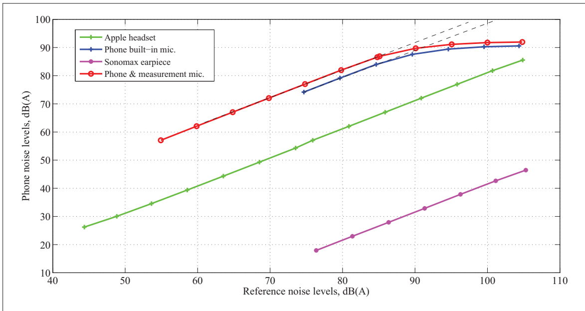
Figure 3.2 Mobile phone noise levels measured in the anechoic chamber while measuring Source 1
