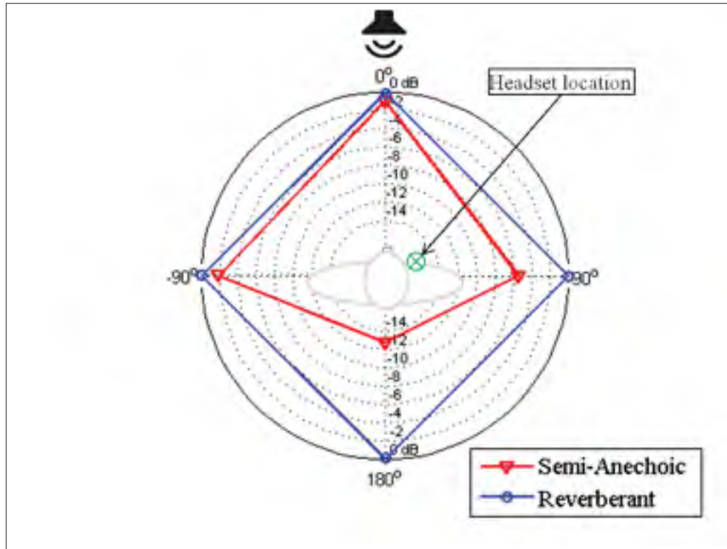
Figure 3.31 Headset overall A-weighted errors, averaged over the range of noise levels, in the semi-anechoic chamber (in red) and in the reverberant chamber (in blue)
