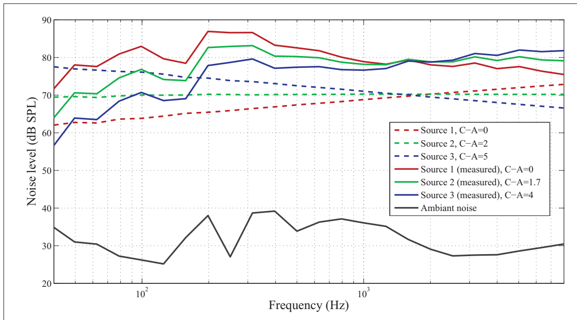
Figure 2.5 Frequency content of the ambient noise, the original signals of Sources 1, 2 and 3 and the measured Sources 1, 2 and 3 with the reference system in the semi-anechoic chamber
