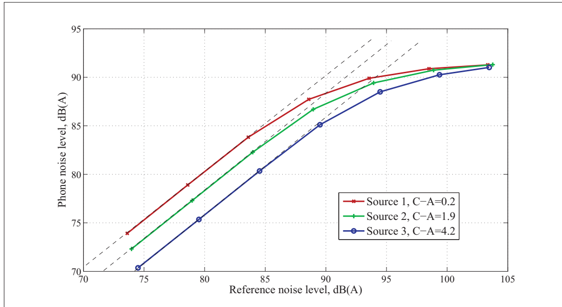
Figure 3.3 Built-in microphone noise levels while measuring Source 1, 2 and 3 in the semi-anechoic chamber
