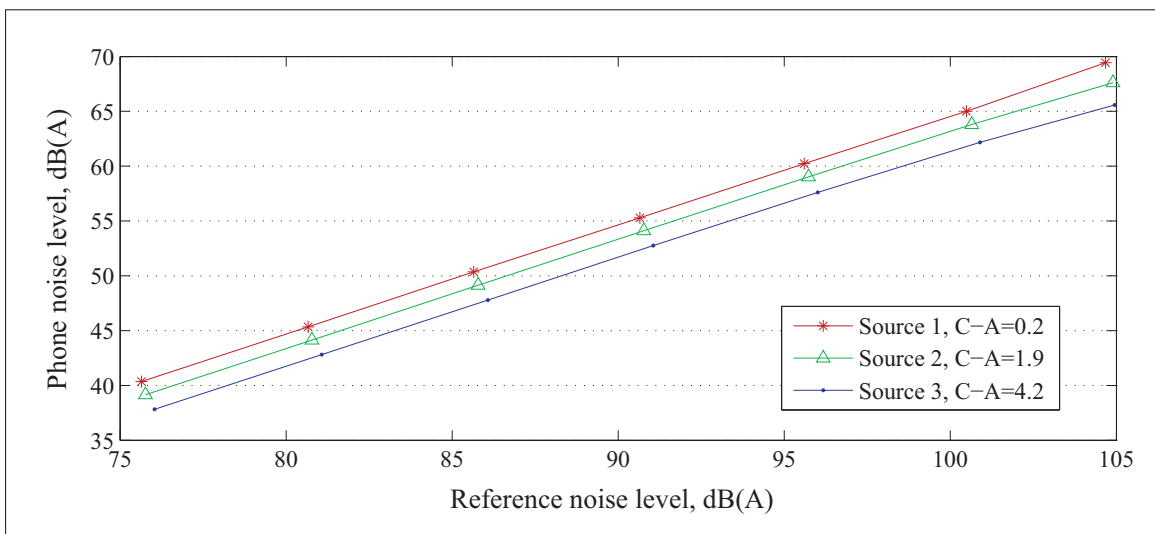
Figure-A VIII-3 Uncalibrated mobile phone noise levels measured with the headset, as compared with the reference noise levels while measuring Source 1, 2 and 3 in the semi-anechoic chamber
