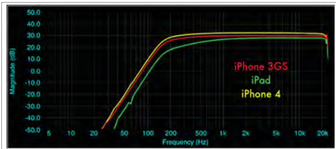
Figure 1.8 iPhone 4 Headset Microphone Frequency Response Comparison. Reproduced with the permission from Faberacoustical (2009)
