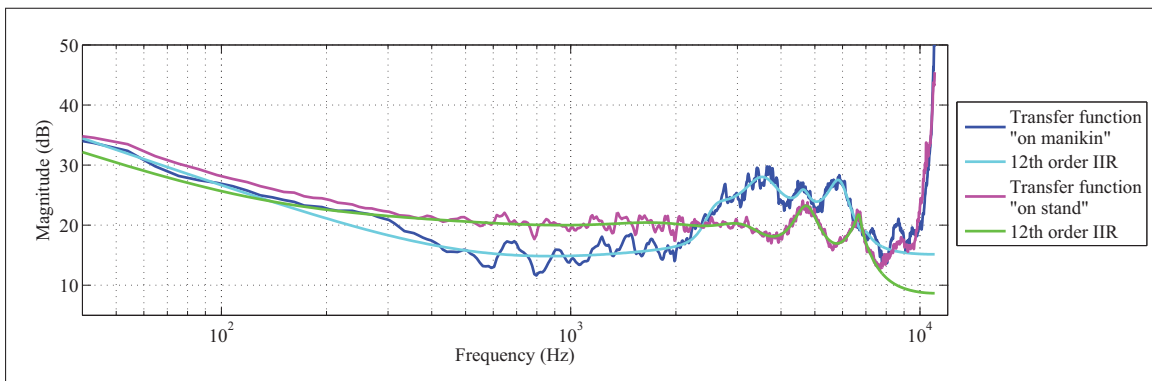
Figure 3.18 Headset transfer functions based on the measurement for different microphone placements and frequency responses of the 12 th order IIR filters, calculated from the truncated-transfer functions (from 43 Hz to 7250 Hz)
