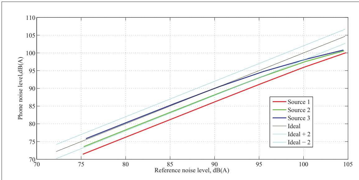
Figure-A VIII-2 Phone noise levels measured with the earpiece, as compared with the reference noise levels while measuring Source 1, 2 and 3 in the semi-anechoic chamber with the phone implementing the frequency-dependent calibration algorithm
