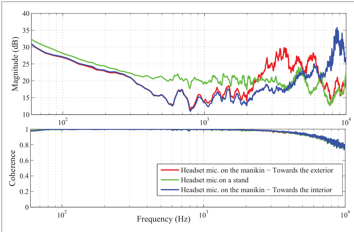
Figure 3.8 Transfer function and coherence values calculated from the measurements conducted with the headset microphone located on a microphone stand and on the ATF
