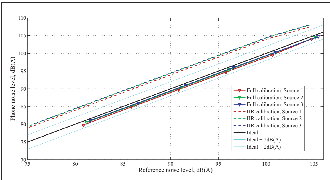
Figure 3.29 Headset noise level measurements carried out in the semi-anechoic chamber, with only a frequency-dependent calibration (IIR calibration) and with frequency and level-dependent calibration (Full Calibration)
