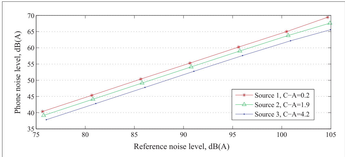
Figure-A VIII-1 Uncalibrated mobile phone noise levels measured with the earpiece, as compared with the reference noise levels while measuring Source 1, 2 and 3 in the semi-anechoic chamber
