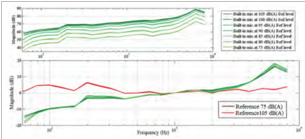
Figure 3.4 Frequency responses of the measurements conducted with the built-in microphone (top half), frequency responses with the magnitude normalized at the 1 kHz third-octave band noise level (top bottom)
