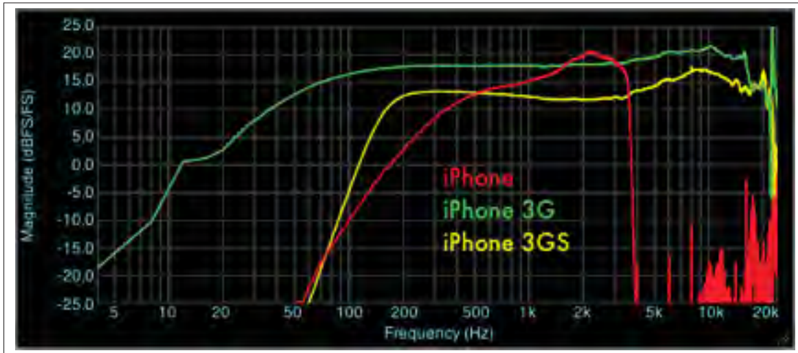
Figure 1.7 Built-in iPhone Microphone Frequency Response Comparison. Reproduced with the permission from Faberacoustical (2009)
