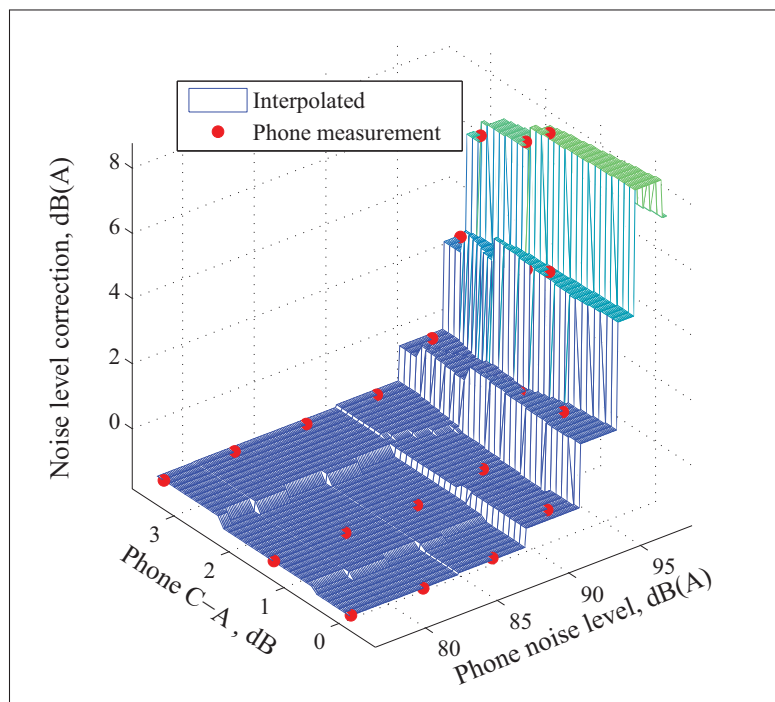
Figure-A VII-2 Built-in microphone measured noise level correction values (in red) and interpolated values with the griddata MATLAB function and its nearest method
