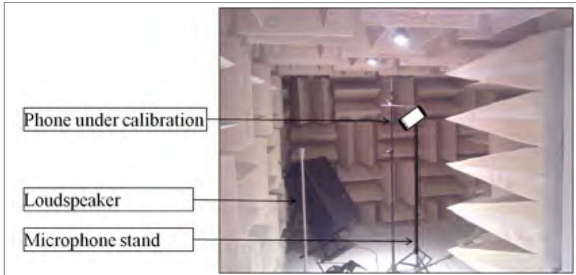
Figure 2.15 Setup of the calibration measurement in the semi-anechoic chamber showing a mobile phone under calibration and the loudspeaker
