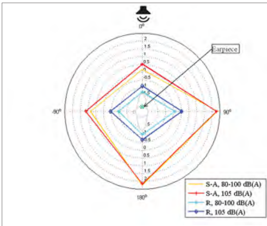
Figure 3.40 Earpiece overall A-weighted errors in the semi-anechoic chamber (in red and orange) and in the reverberant chamber (in blue)
