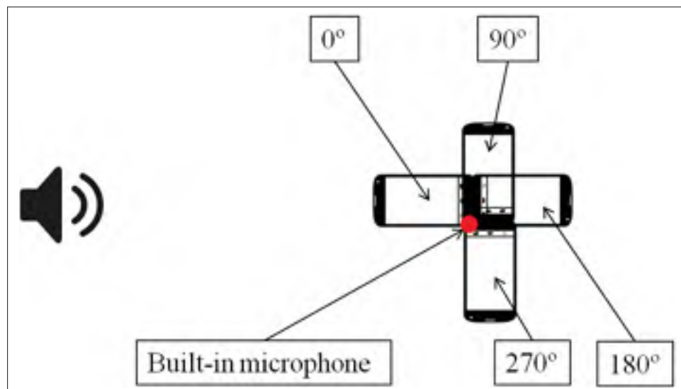
Figure 2.21 Top view of the built-in microphone orientation in the semi-anechoic chamber with the mobile phone placed flat
