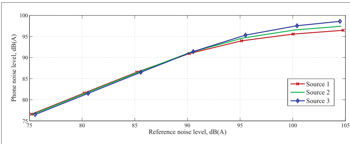
Figure 3.24 Built-in microphone noise level with a frequency-dependent calibration (6th order IIR filter), function of the reference noise level, while measuring Source 1, 2, 3
