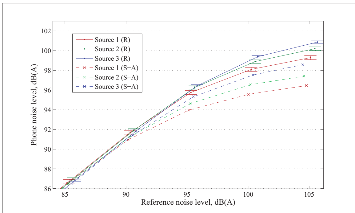
Figure 3.13 Built-in noise level measurements measured in the semi-anechoic (S-A, in dashed line) and reverberant (R) chambers
