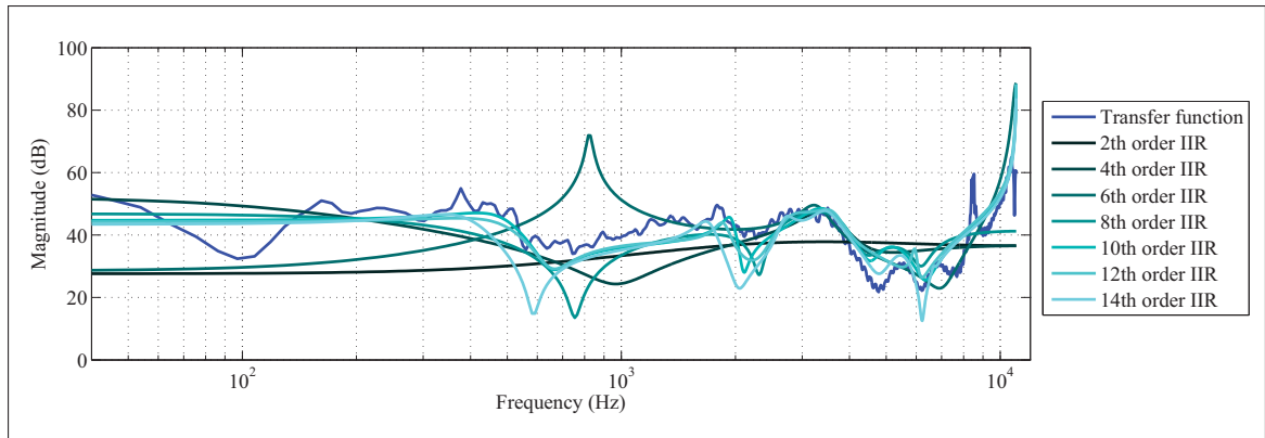
Figure 3.19 Earpiece initial transfer function for the earpiece located on the ATF and frequency responses of IIR filters for orders from 2 to 14
