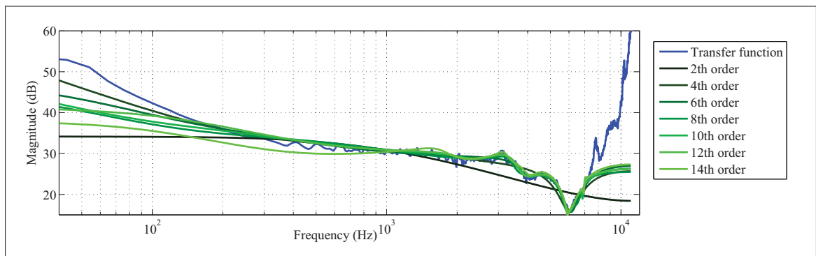
Figure 3.20 Earpiece initial transfer function for the earpiece located on a stand and frequency responses of IIR filters for orders from 2 to 14
