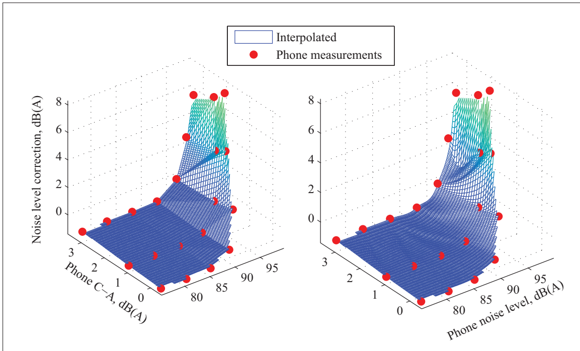
Figure 3.25 Built-in microphone measured noise level correction values (in red) and interpolated values with the griddata MATLAB function and the linear and cubic methods
