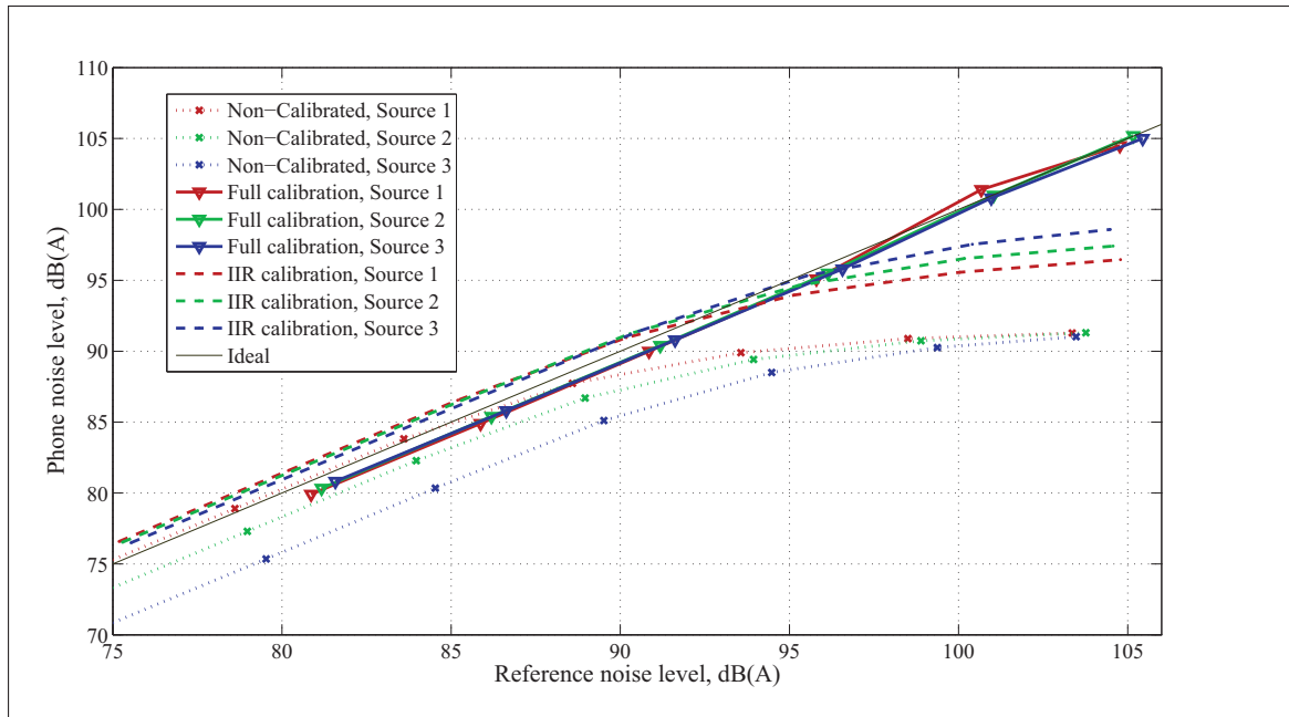
Figure 3.32 Built-in microphone noise level measurements in the semi-anechoic chamber without calibration, with only a frequency-dependent calibration (IIR calibration) and with frequency and level-dependent calibration (Full Calibration)
