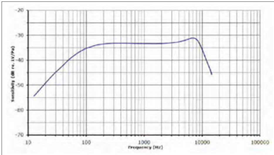
Figure 2.12 Frequency response of the Sonomax® earpiece microphone, extracted from Sonion (2009)
