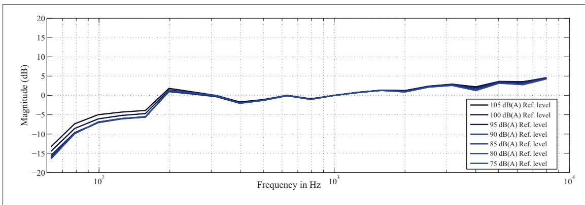
Figure 3.5 Frequency responses of the measurements conducted with reference microphone plugged into the mobile phone with the magnitude normalized at the 1 kHz third-octave band noise level
