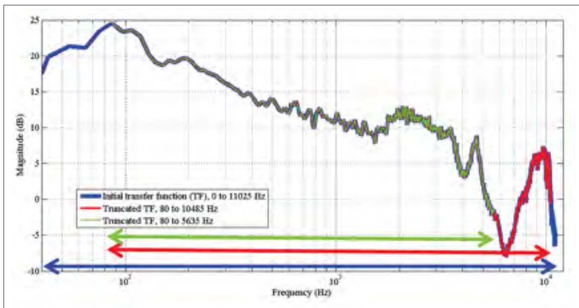
Figure 3.15 Initial transfer function (in blue) based on the built-in microphone measurement, truncated-transfer functions, defined from 80 Hz to 10485 Hz (in red) and to 5635 Hz (in green)
