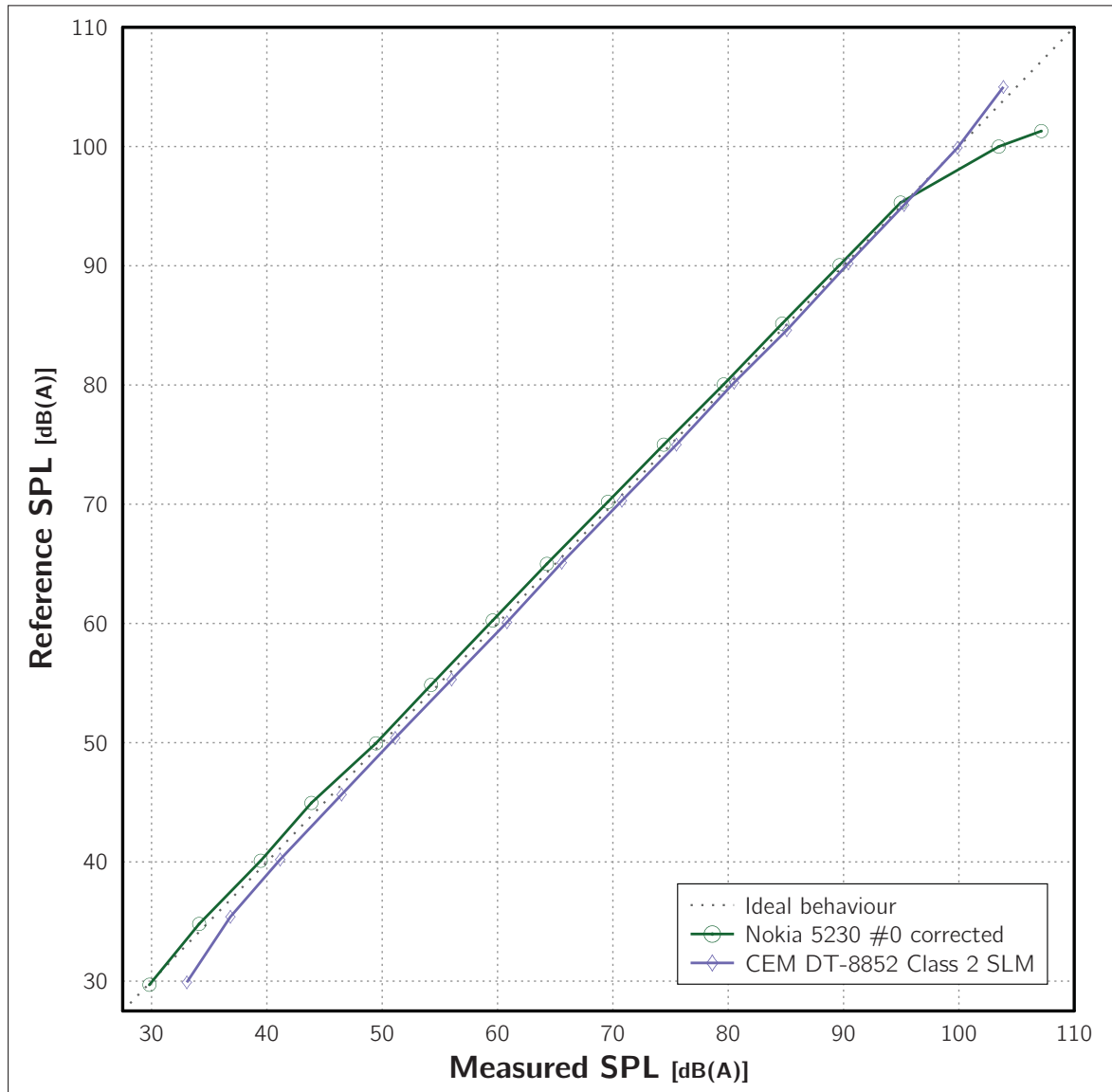
Figure 1.9 Validation measurements for white noise made by the calibrated Nokia 5230 #0 and a professional SLM. Reproduced with the permission from Stevens (2012)
