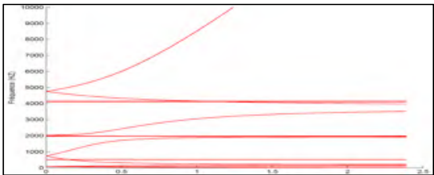
Figure 3 Campbell Diagram
