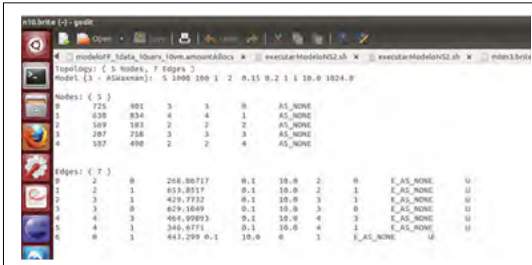
Figure A III. 2 BRITE Format with 5 nodes and 7 edges
