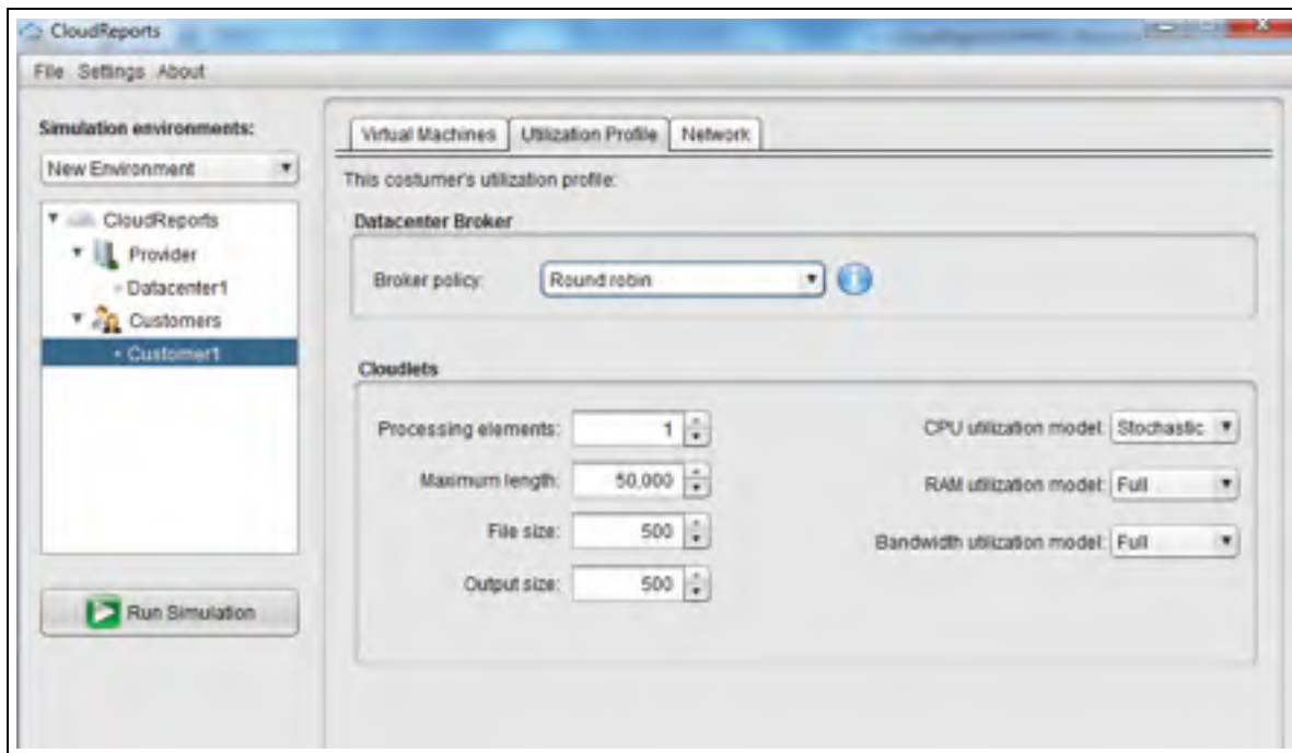
Figure A I. 6 Brocker policy in CloudReports
