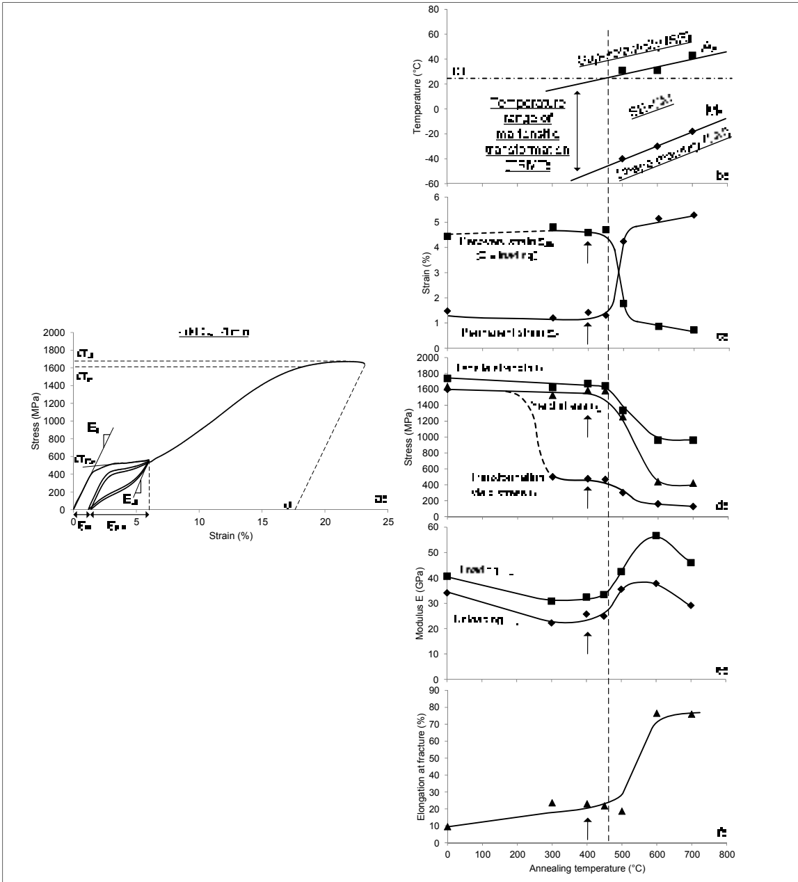
Figure 2.5 Mechanical properties of Ti-50.6at.%Ni Ø2mm rod:
