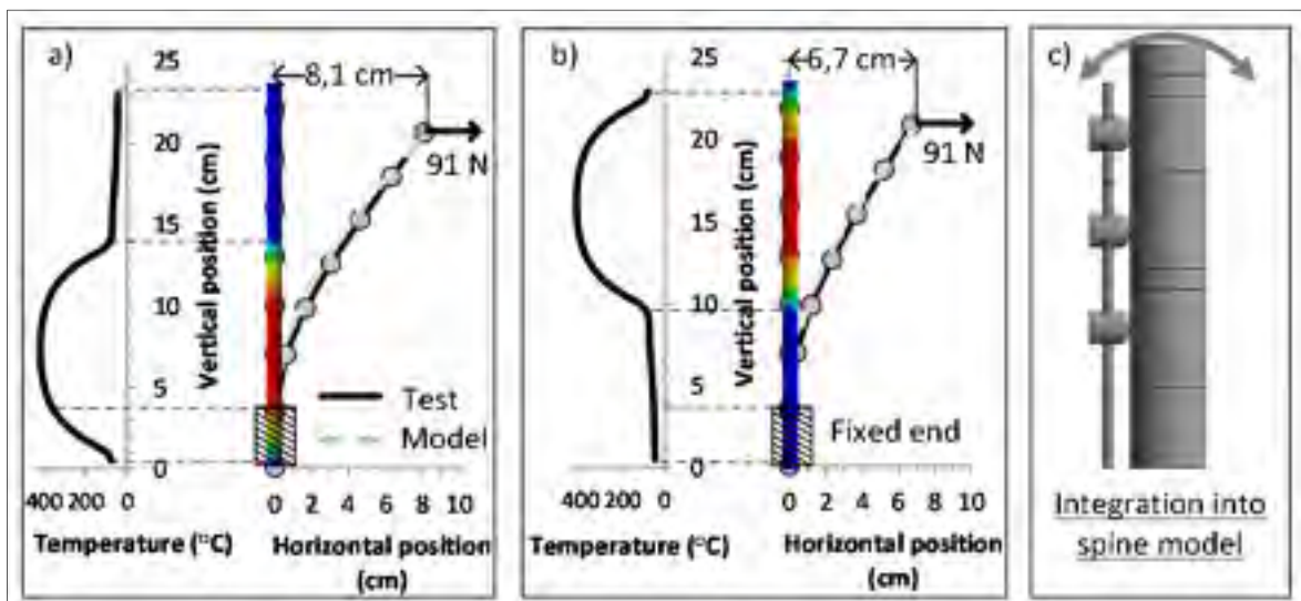
Figure 3.11 Application of the mechanical model: a,b) temperature distributions and bending profiles with a) superelastic end fixed, and b) hardened end fixed; c) Illustration of a potential integration into an instrumented model of the human spine
