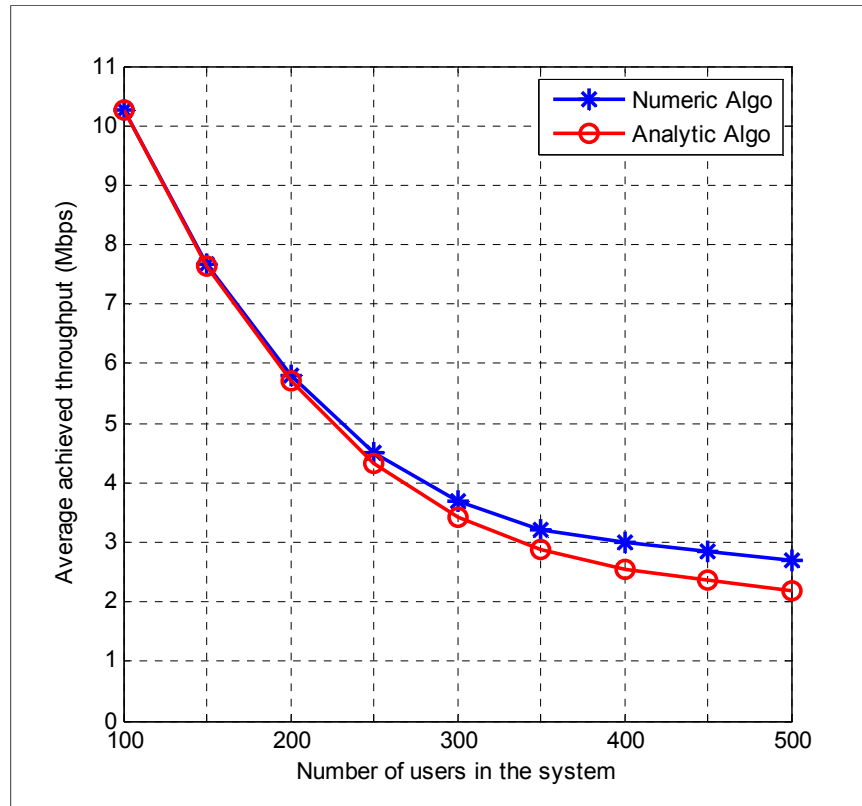
Figure 2.7 Average achieved throughput per user density
