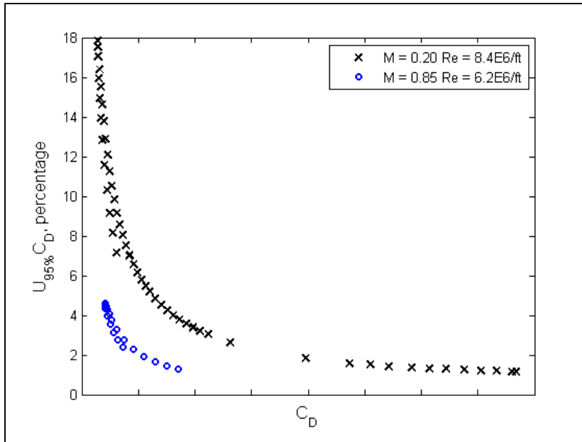
Figure 3.10 Coefficient of drag 95-percent uncertainty at different operating conditions ( C_D scale = 0.05)
