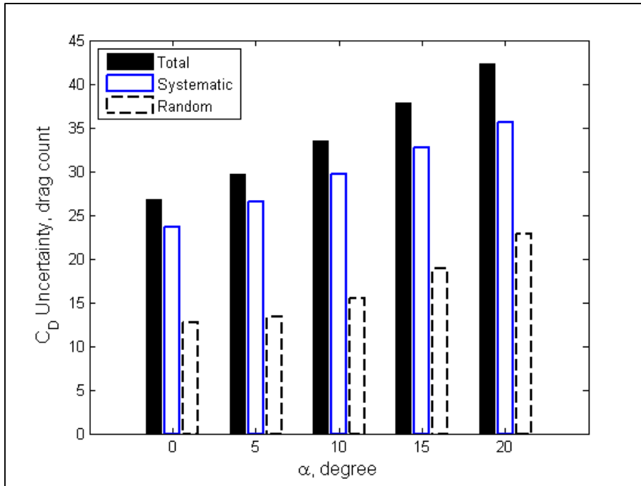
Figure 3.15 Systematic, random and total 95-percent uncertainty of coefficient of drag
