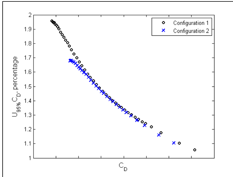
Figure 3.7 Coefficient of drag 95-percent uncertainty comparison between two different model configurations tested under similar wind tunnel operating conditions ( C_D scale = 0.05)
