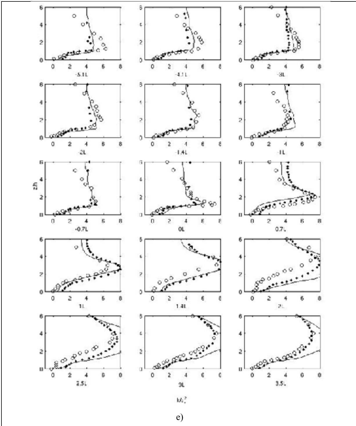
Figure 2: Comparison of numerical results over a forested hill, using a hybrid model (solid line); the LES model (dots); and observations (open circles) to show velocity a); shear stress b); variance u'u' c); variance w'w' d); and turbulent kinetic energy e)
