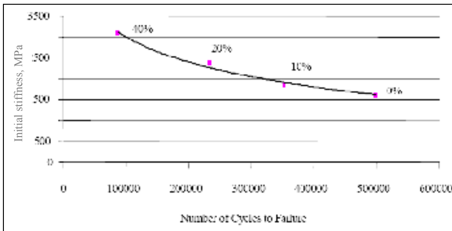
Figure 2.36 Beam Fatigue Cycles to Failure vs. Stiffness, PG 64-22, Low Strain Taken from McDaniel and Anderson (2001)
