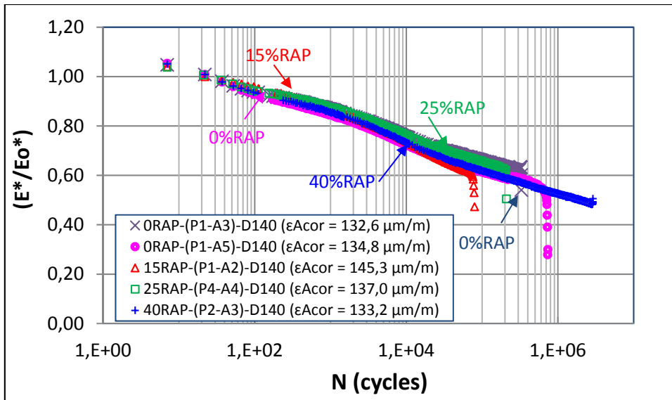
Figure 6.19 Comparison of a fatigue test at test at 140 \mu\text{m}/\text{m} strain level, values of real strain range from 133 to 145 \mu\text{m}/\text{m} , for 4 recycled mixtures in the axes |E^*/E_0| - log (N) (0% RAP, 15% RAP, 25% RAP, and 40% RAP)
