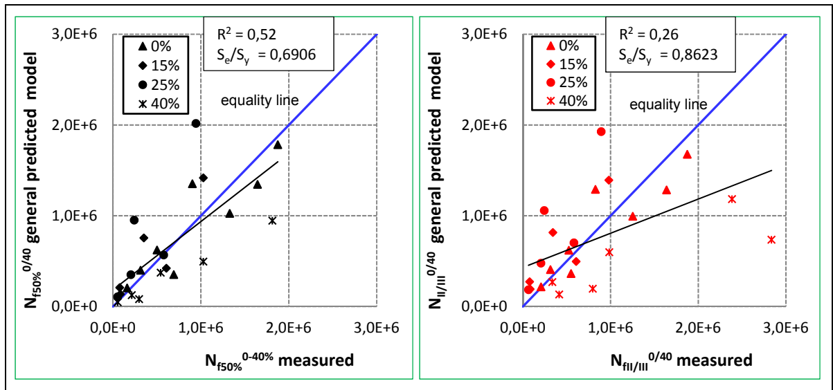
Figure 7.4 Predicted versus observed N_f using the two criterion N_{f50\%} and N_{fII/III} using the testing data up to 40% with the value of the parameter A^{0/40} (Table 7.2) fixed from the k_2^{\%RAP} - \%RAP relationship ( k_2^{0/40} versus %RAP)
