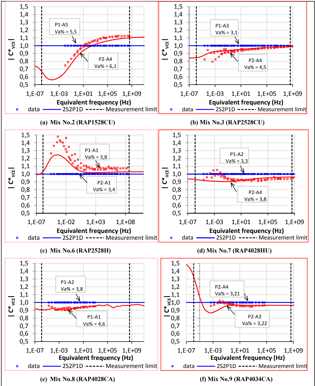
Figure 5.16 |C_{VCE-data}^*| and |C_{VCE-2S2P1D}^*| vs. equivalent frequency ( T_{ref} = 5^\circ C )
