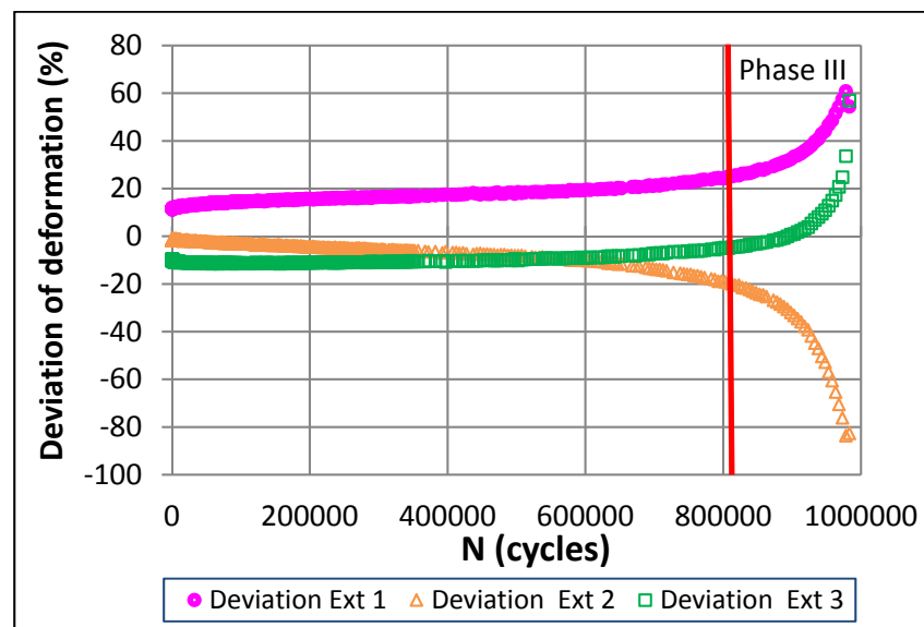
Figure 6.8 Differences relative to the mean of the deformation (average deviations of deformation) depending on the number of cycles for the test 25RAP-(P1-A1)-D110 ( \epsilon_A = 108,8 \mu\text{m}/\text{m} ; T = 10^\circ\text{C} )
