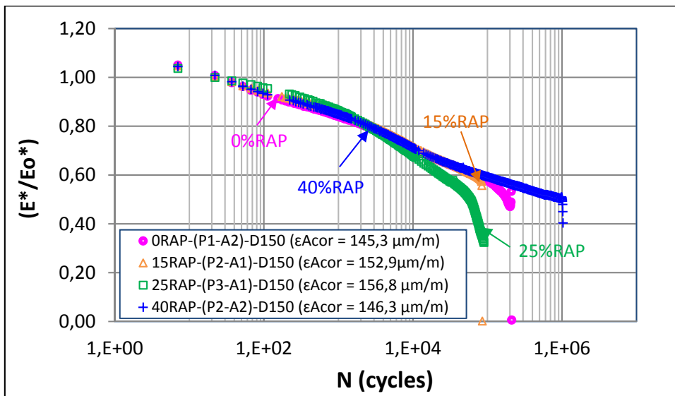
Figure 6.20 Comparison of a fatigue test at test at 150 \mu\text{m}/\text{m} strain level, real strain values lie in the range of 145 to 157 \mu\text{m}/\text{m} , for 4 recycled mixtures in the axes |E^*/E_0| - log (N) (0% RAP, 15% RAP, 25% RAP, and 40% RAP)
