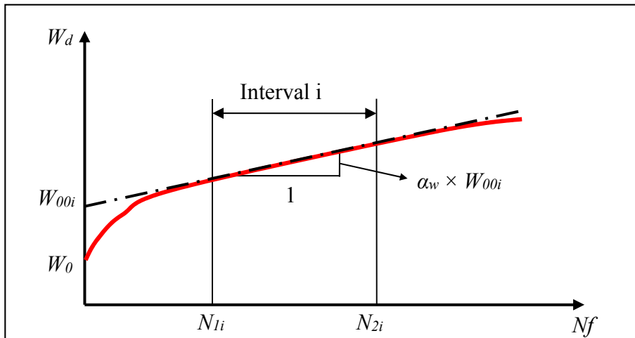
Figure 2.21 Determination of W_{00i} and a_w from the dissipated energy curve Taken from Baaj (2002)
