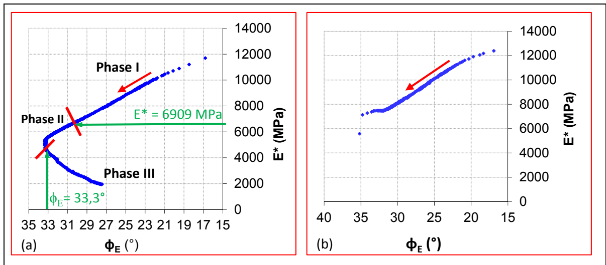
Figure 6.14 Presentation for the black space for the tests (a) 40RAP-(P1-A3)-D170 ( \epsilon_A = 168 \mu\text{m/m} ; T = 10^\circ\text{C} ) (b) 25RAP-(P4-A5)-D130 ( \epsilon_A = 128,5 \mu\text{m/m} ; T = 10^\circ\text{C} )
