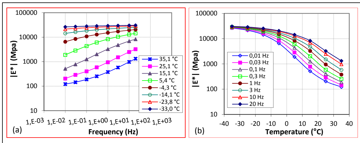
Figure 5.2 Isothermal curves (a) and isochrones (b) of the norm of the complex modulus versus the frequency and the temperature, respectively (mix RAP028: sample P1-A4)
