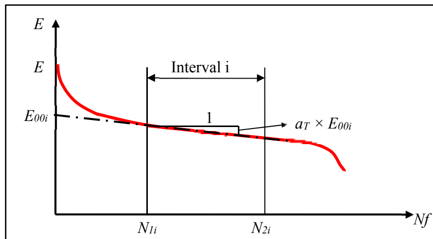
Figure 2.20 Determination of E_{00i} and a_T from the dissipated energy curve Taken from Baaj (2002)
