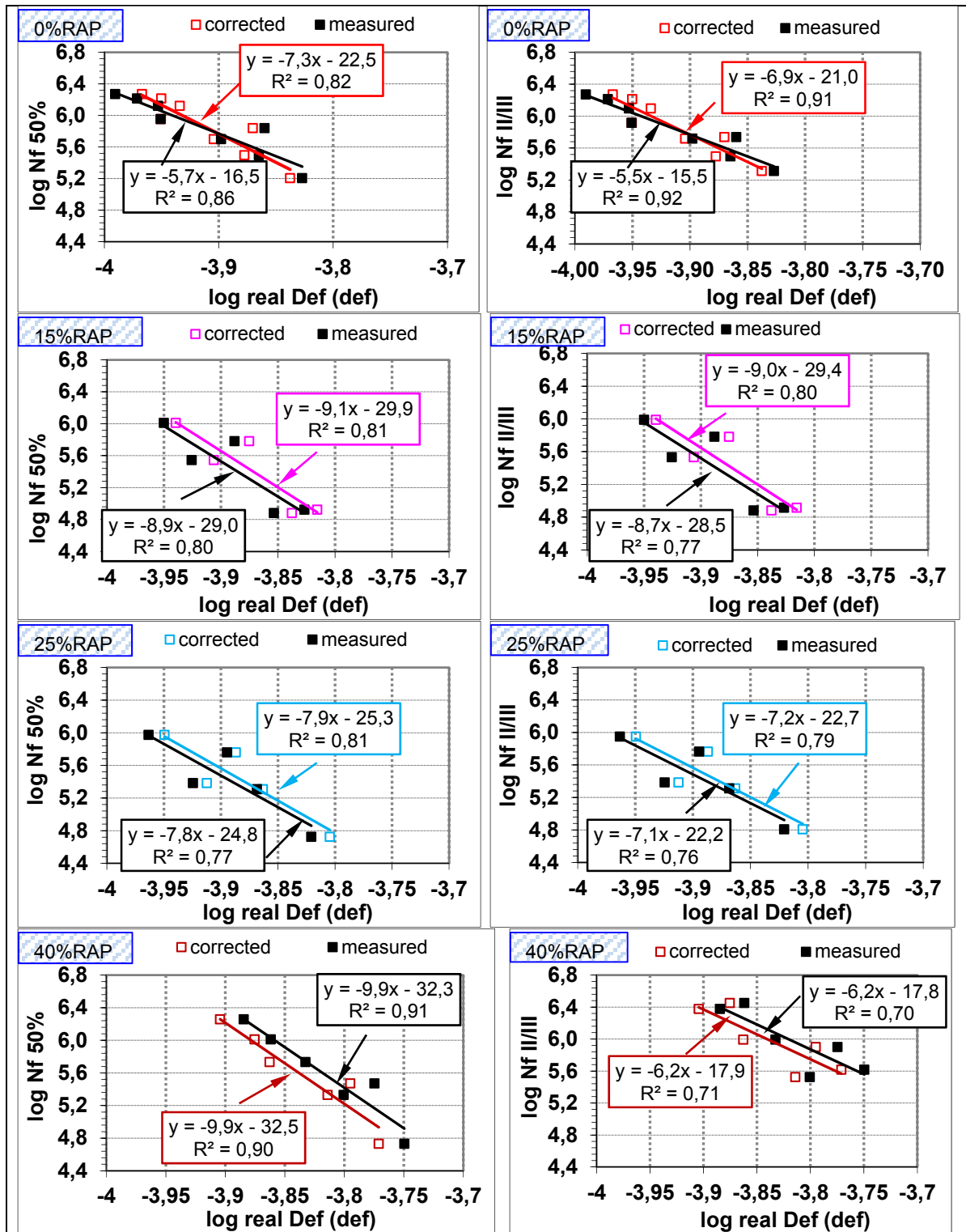
Figure-A III-1 Characteristic of fatigue for the selected tested mixtures before and after correction based on air void of 5,1% using the two criterions
