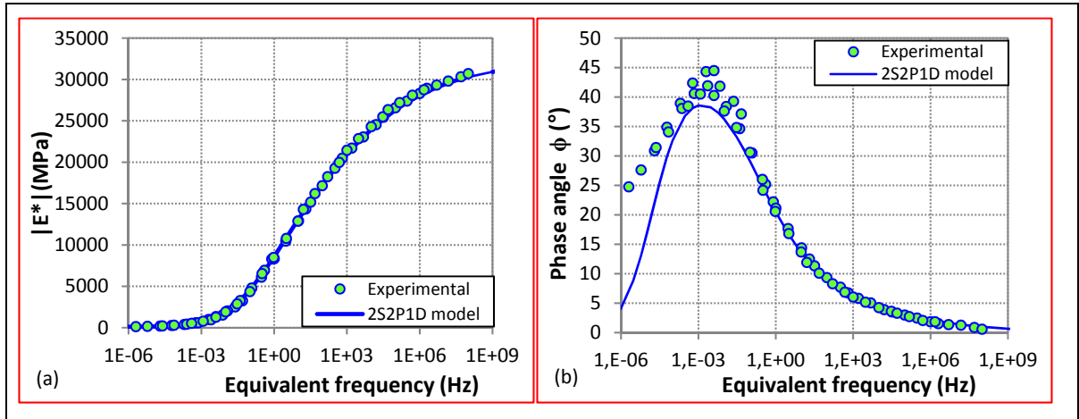
Figure 5.6 Master curves of the virgin mix (RAP028): Simulation with the model 2S2P1D ( T_{ref} = 5,4^{\circ}\text{C} ), (a) Master curves of the norm of the complex modulus |E^*| , (b) Master curve of \phi of the complex modulus
