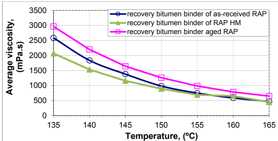
Figure 4.10 Viscosity of the unaged RAP and the aged RAP recovered asphalt binders
