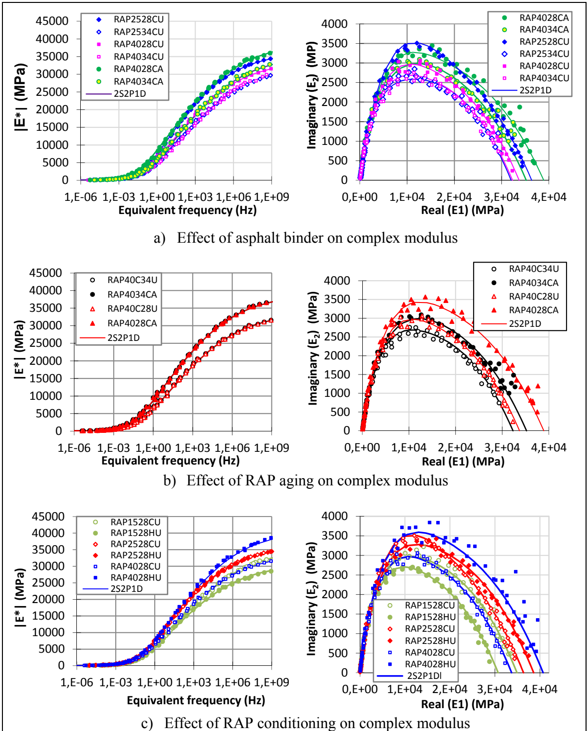
Figure 5.14 Master curves of the norm of the complex modulus ( T_{ref} = 10^\circ C ) and Cole-Cole diagram different mixes with different conditioning
