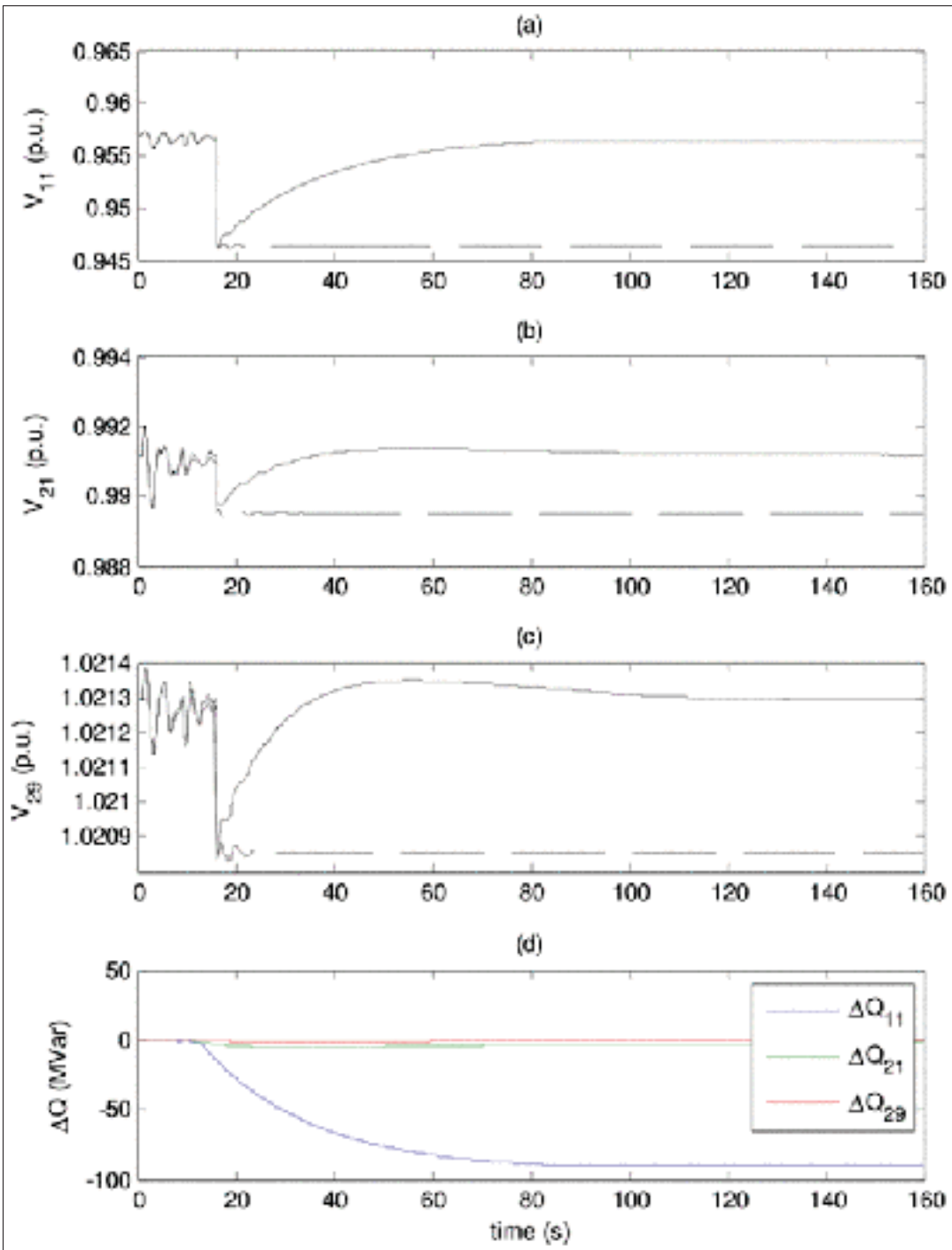
Figure-A I-7 Simulation Results for Scenario 1: (a,b,c) Voltage Profile at pilot nodes. Solid line: MPC SVC, dashed line: No Control. (d) Reactive power changes on pilot nodes by static var compensators
