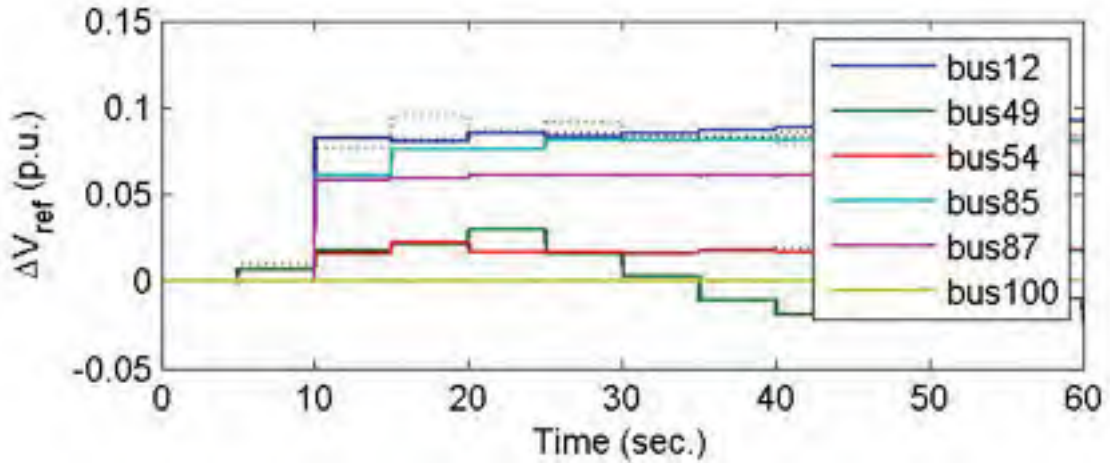
a) Change of reference voltage of AVRs connected to generators
