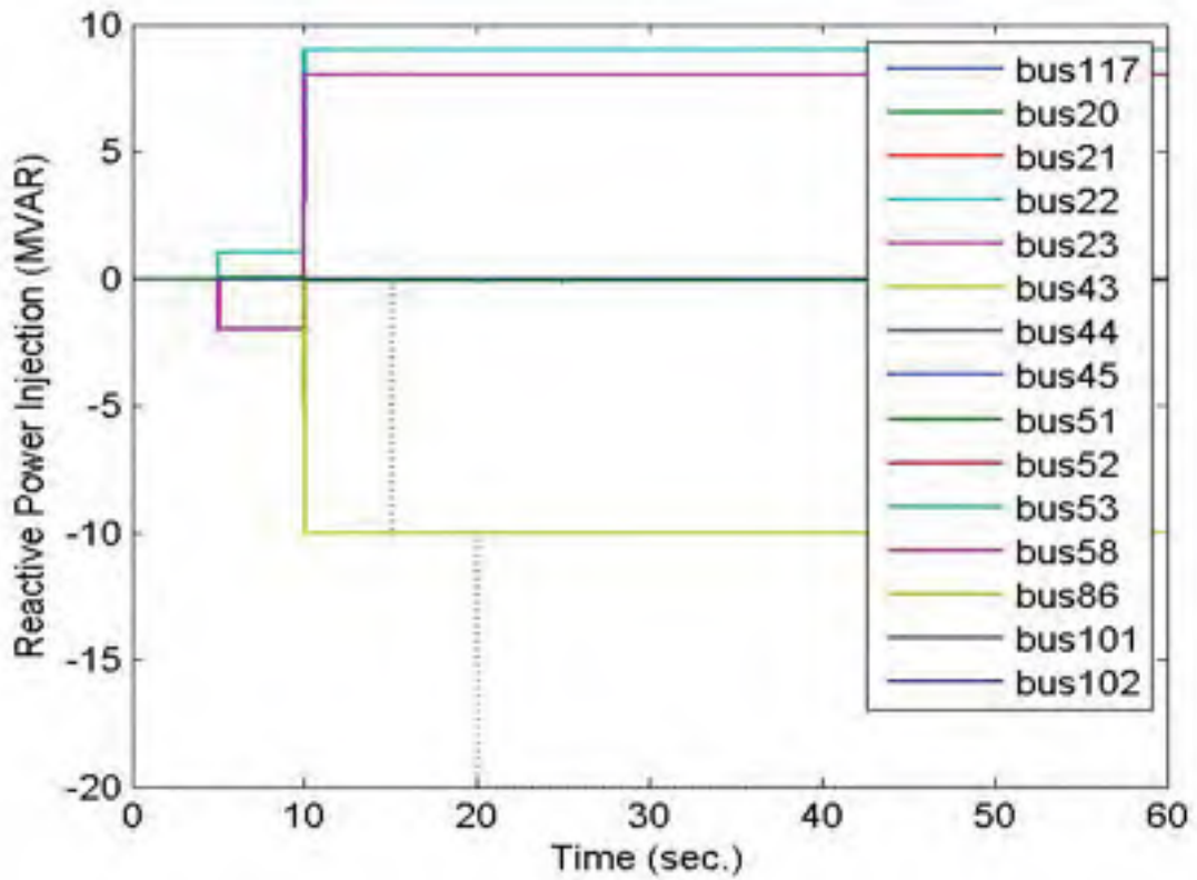
b) Reactive power injection by capacitor/inductor banks
