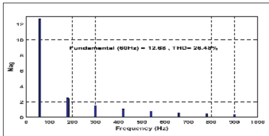
Figure 3.11 Harmonic spectrum of the source current in study state
