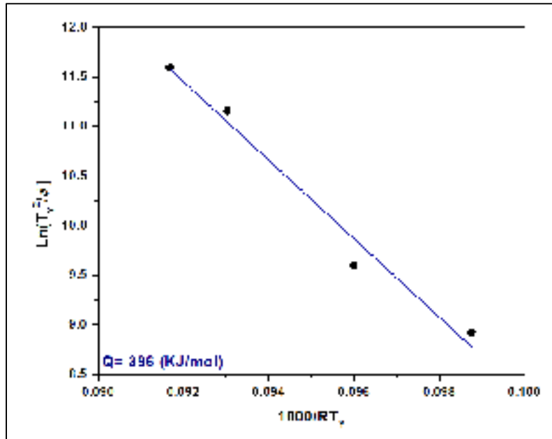
Figure 4.5 The relationship between \ln(T_Y^2/\varphi) and 1000/RT_Y for determining activation energies of \gamma' precipitation ( R^2=0.98 ).
