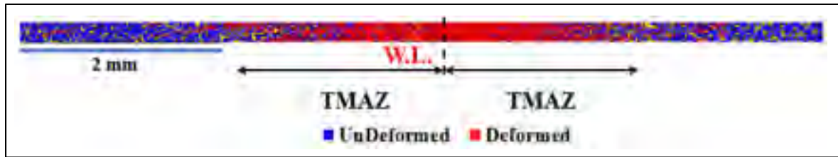
Figure 2.12 Low magnification EBSD map of the transversal cross section of the LFWed sample#4. Red zones depict deformed areas and blue areas are undeformed zones.
