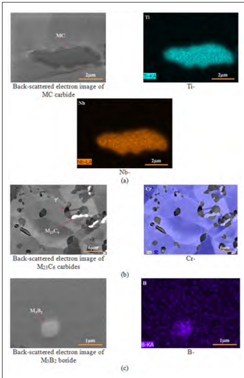
Figure 3.2 BSE/EDS X-ray maps of the (a) MC carbide mainly consisting of Ti, Nb (b) \text{M}_{23}\text{C}_6 carbides mainly consisting of Cr (c) \text{M}_3\text{B}_2 boride.
