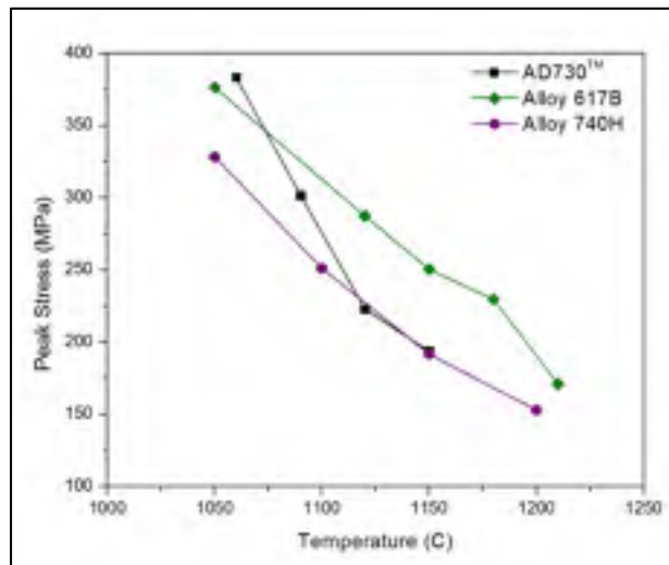
Figure 2.3 Peak stress values of the AD730™ and the other Ni-based superalloys at strain rate 1\text{s}^{-1} .
