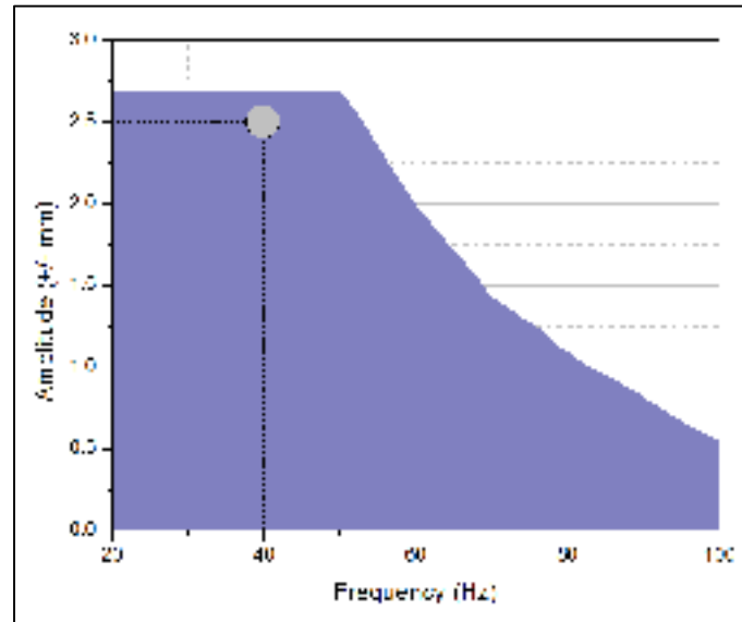
Figure 2.5 Operating window for LFW machine (FW34 at TWI, Cambridge, UK).
