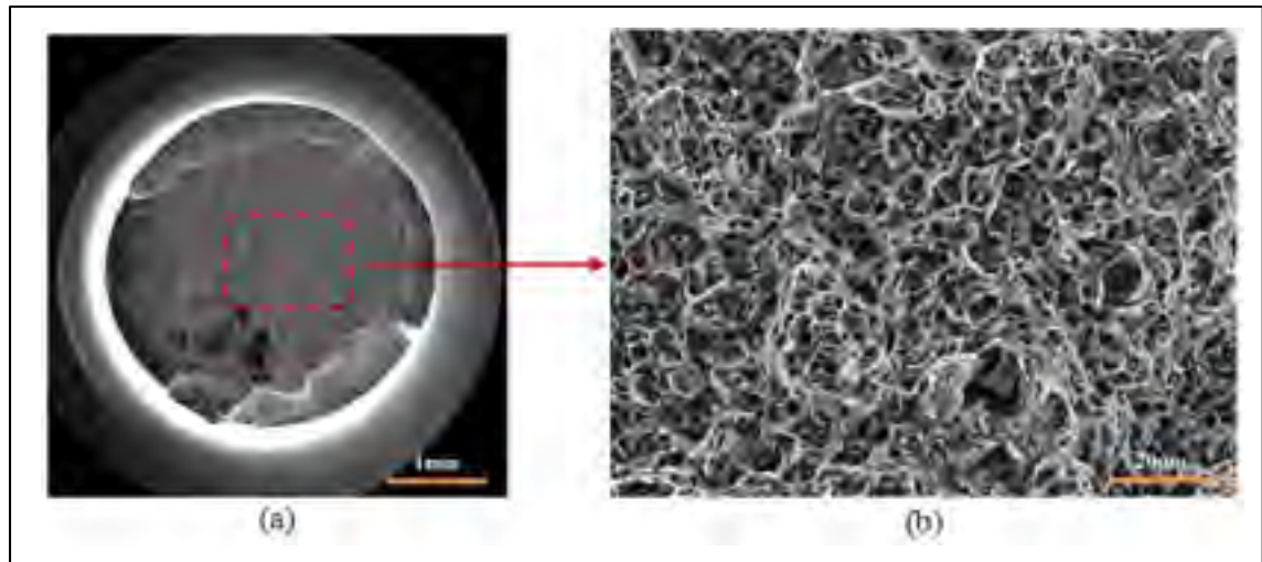
Figure 2.24 (a) Macrofractograph of the fractured surface at room temperature. The central portion of the fracture is slightly flat and 45^\circ shear lips surround this region. (b) Higher-magnification view of the selected area (red box) at the center of the specimen which consists of equiaxed dimples formed during ductile rupture.
