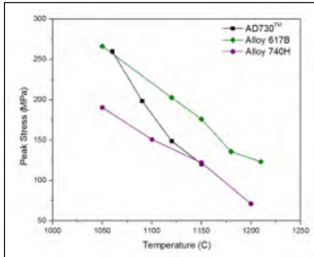
Figure 2.2 Peak stress values of the AD730™ and the other Ni-based superalloys at strain rate 0.1\text{s}^{-1} .
