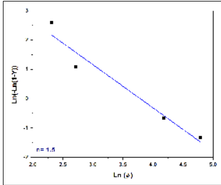
Figure 4.4 The relationship between \ln[-\ln(1 - Y)] and \ln\phi at 1039°C for determining Avrami exponent of \gamma' precipitation ( R^2 = 0.95 ).
