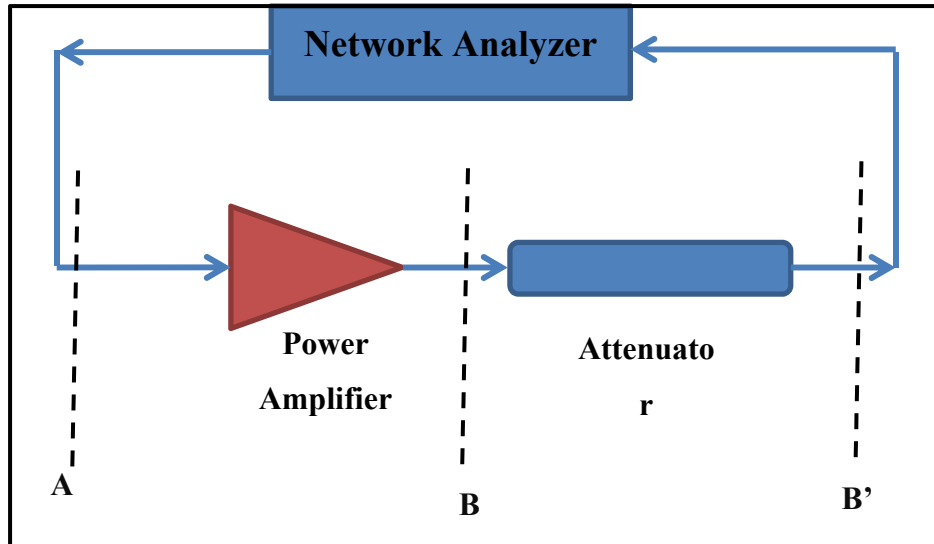
Figure 4.3 measurements setup of fabricated PA
