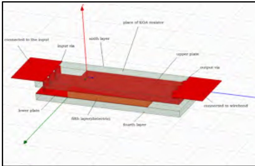
Figure 2.11 3D capacitor
