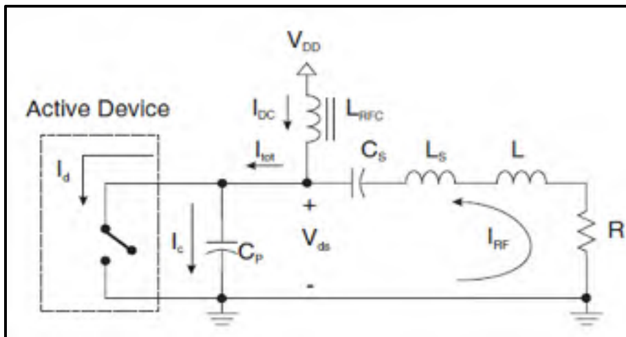
Figure 1. 9 Circuit diagram for Class E amplifiers
