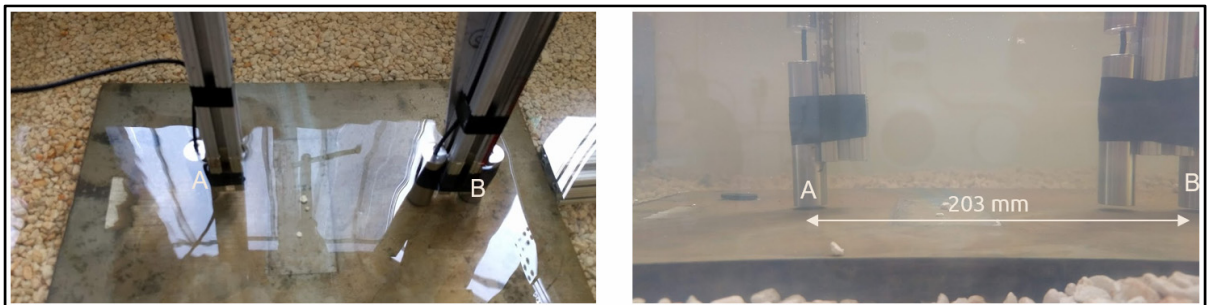
Figure 3.6 Measurement setup for pitch-catch tests on a cast-iron plate.
