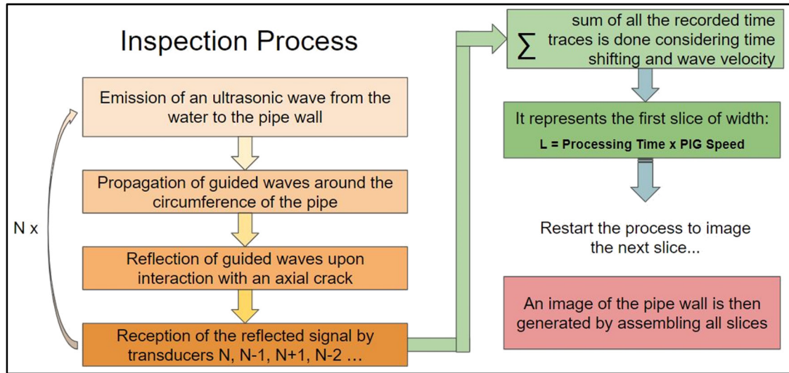
Figure 2.2 Inspection process
