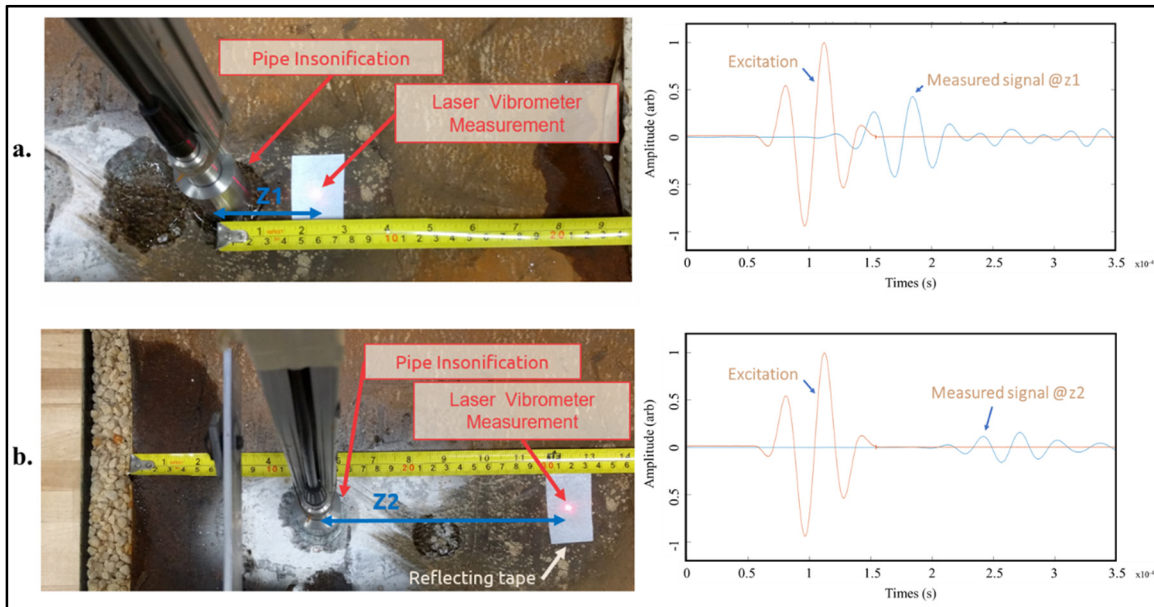
Figure 3.2 Dry tests, a. at a given distance Z_1 between the transducer and the laser vibrometer measurement, b. at a given distance Z_2 between the transducer and the laser vibrometer measurement. The setup is shown on the left and the emitted and received signal on the right
