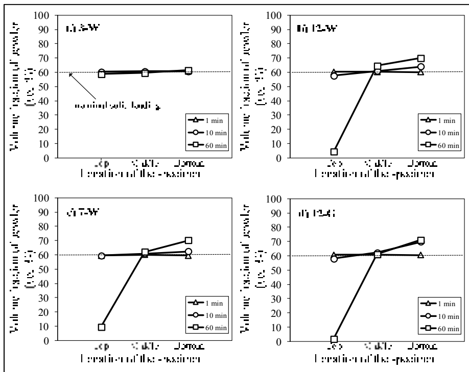
Figure 4.8 Volume fraction of powder according to the position, time left in the molten powder state, and feedstock
