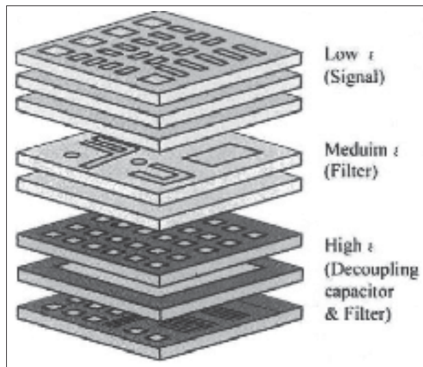
Figure 0.4 Passive components embedded in substrate (Imanaka (2005))
