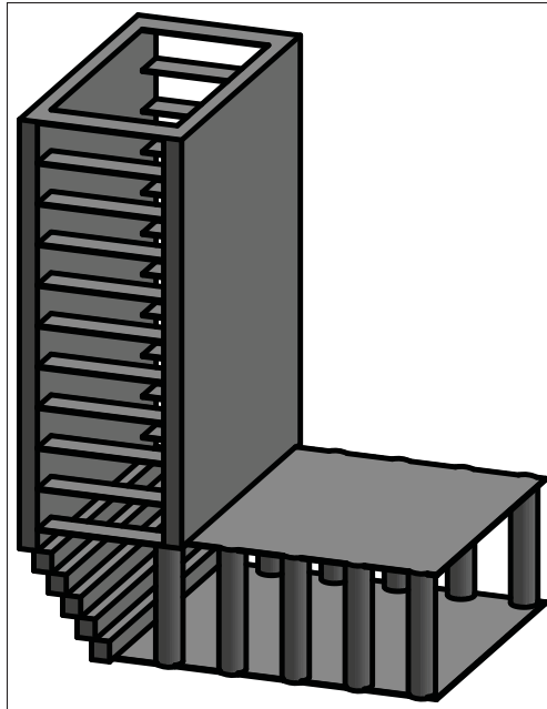
Figure 3.19 Geometry of V-LIW to H-LIW corner transition
