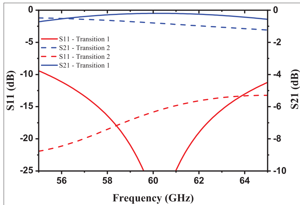
Figure 3.20 Simulation results for transition from V-LIW to H-LIW
