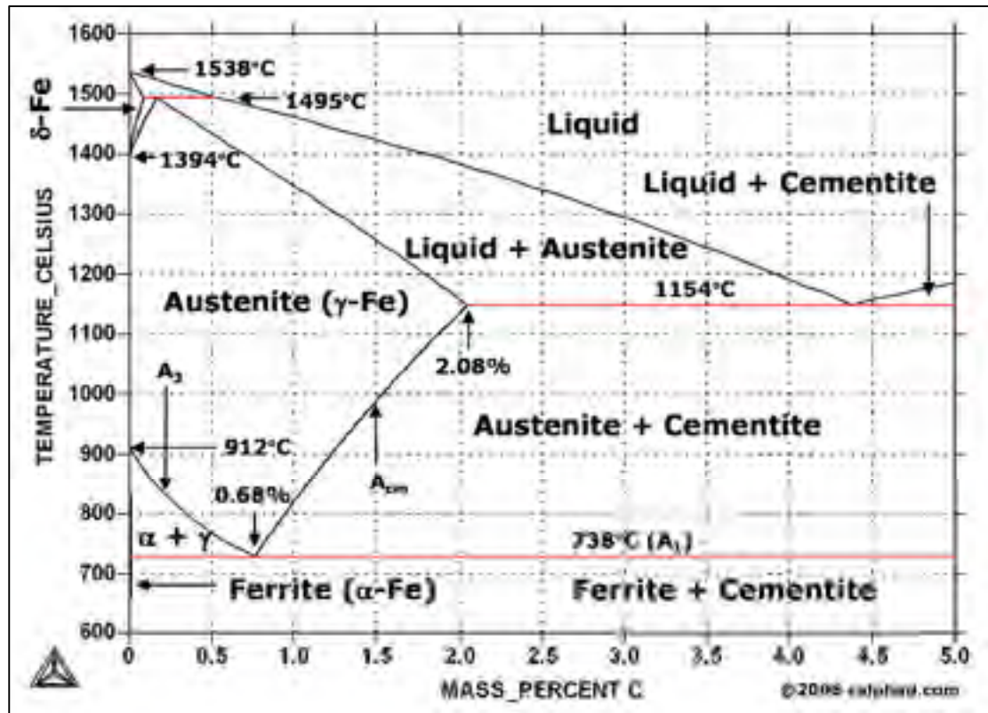
Figure 1.6 Illustration of \gamma solvus line in Fe-C phase diagram. http://www.calphad.com/iron-carbon.html
