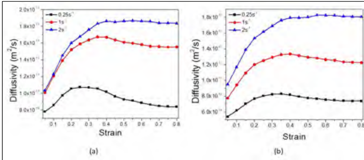
Figure 5.14 Graph depicting Diffusivity due to pipe diffusion vs strain for (a) 1200^\circ\text{C} and (b) 1150^\circ\text{C}
