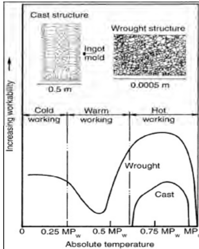
Figure 1.7 Schematic of relative workability of cast metals and wrought metals at cold, warm, and hot working temperatures. The melting point is denoted as MP_c (cast metals) or MP_w (wrought metals) (Dieter, Kuhn et Semiatin, 2003)
