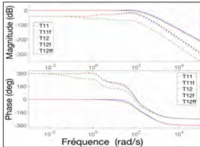
Figure 4.54 Bode de T_{11}(s) , T_{12}(s) , T_{11f}(s) , T_{12f}(s) , T_{12ff}(s)
