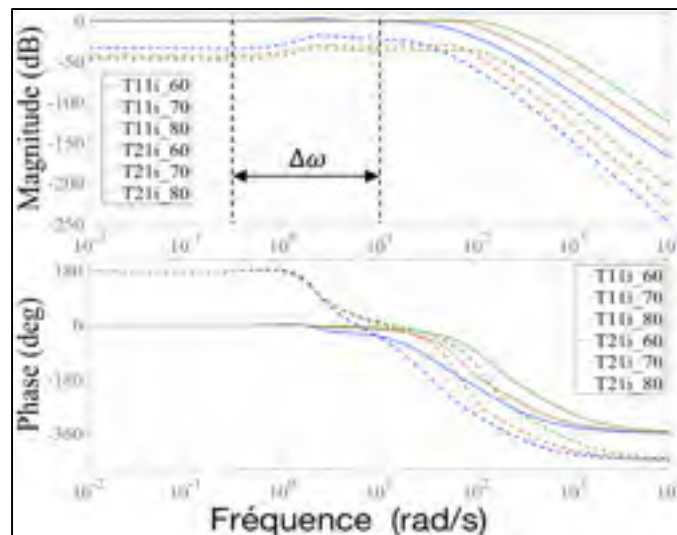
Figure 4.16 Bode de T_{11i}(s) et T_{21i}(s)
