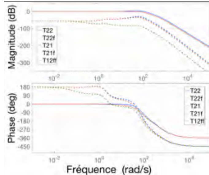
Figure 4.55 Bode de T_{22}(s) , T_{21}(s) , T_{22f}(s) , T_{21f}(s) , T_{21ff}(s)
